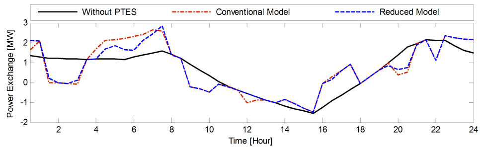
(a) Power exchange at the grid supply
