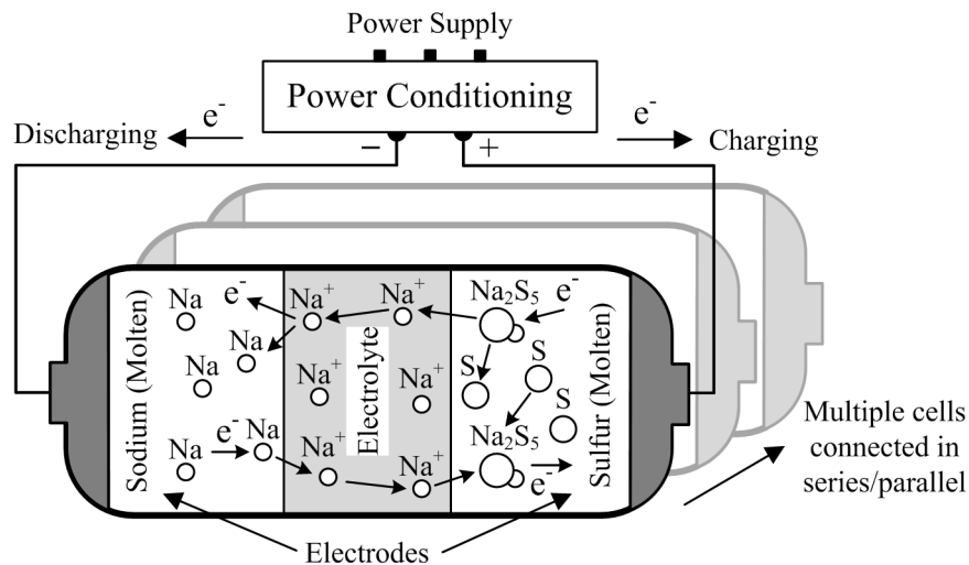
Figure 4.5: An example of battery storage operation
