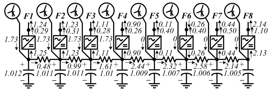
a) Pre-contingency operation
