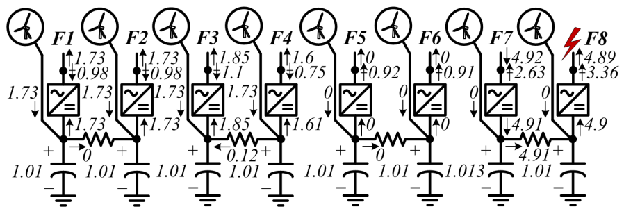
c) Post-contingency long-term operation
