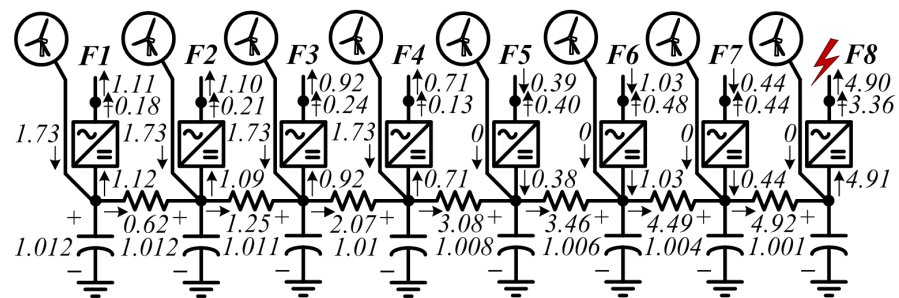
b) Post-contingency short-term operation
