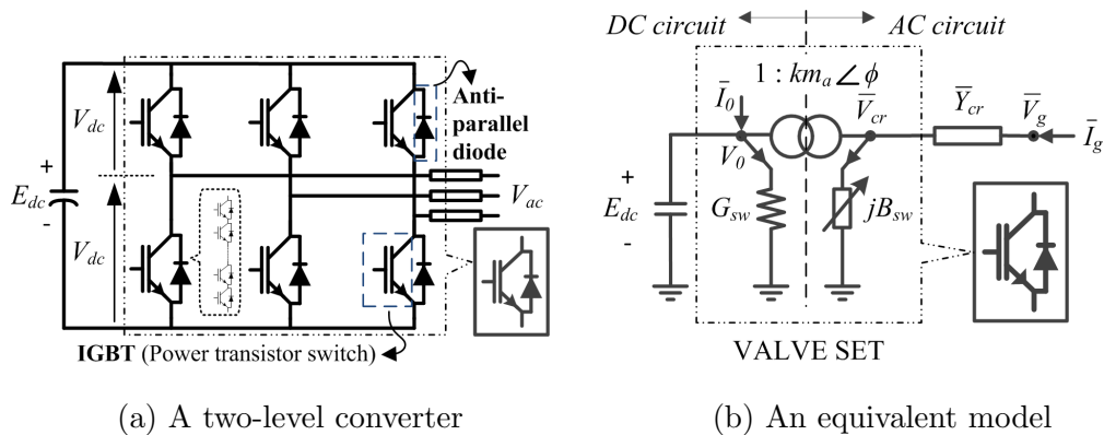
Figure 3.1: Three-phase voltage source converter
