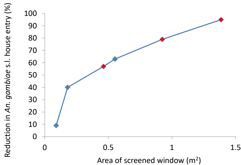
Fig. 3.3 Relationship between surface area of screened windows and reduction in house entry by An. gambiae s.l. Blue diamonds are results from the small window experiment and red diamonds are those from the large window experiment.
