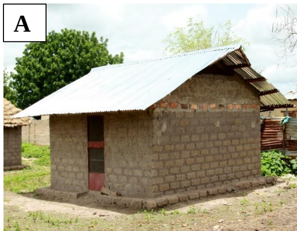
Fig. 2.2: RooPfs house and the gable window: A) RooPfs house B) close-up of screened gable window
