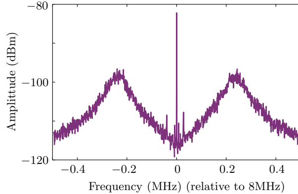
Figure 4.5: In-loop locked error signal noise observed on an RF spectrum analyser centred about the modulation frequency of 8 MHz. The noise sidebands peak at a frequency of \sim \pm 0.25 MHz, indicating the servo bandwidth.
