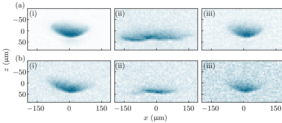
Figure 6.10: Images of the 5s36d\ ^3D_2 MOT for (a) an initial density of 1 \times 10^{12}\text{ cm}^{-3} and (b) an initial density of 5 \times 10^{10}\text{ cm}^{-3} where (i) no coupling laser applied (ii) t_d = 5\text{ ms} and (iii) t_d = 5\text{ ms} , then UV is turned off for 6 ms.
