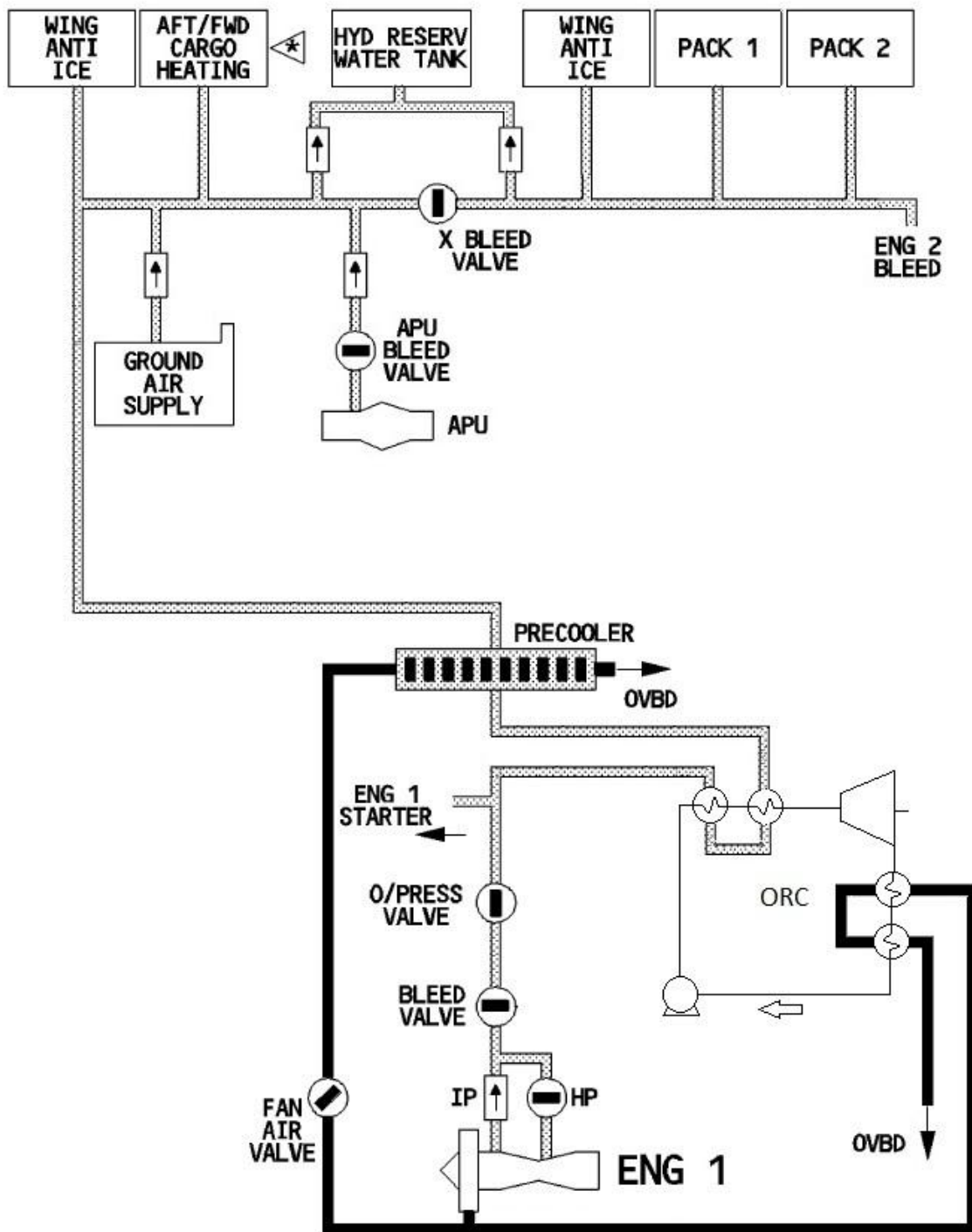
Figure 5-3: Modified diagram of bleed system from the flight crew operating manual [37] with ORC before the precooler.
