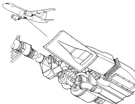
Figure 5-5: NACA air inlet [38].
