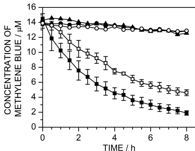
Figure 7.5: Degradation profiles of methylene blue dye solution (20 \mu\text{M} in high purity water, +70 wt%, TCL UK Ltd.): MS(N 2 /O 2 ) in the presence of visible light ( \blacktriangle ); MS(N 2 ) in the presence of visible light ( \blacksquare ); MS(N 2 ) in the absence of visible light ( \square ); in the presence of visible light without TiO 2 composite microspheres ( \bullet ); and in the absence of visible light without TiO 2 composite microspheres ( \circ ). Macrosphere loadings when present were 12.5 \pm 0.1 \text{ mg mL}^{-1} . Error bars are the standard deviation of three repeat experiments. Trend lines have been added only as a guide.
