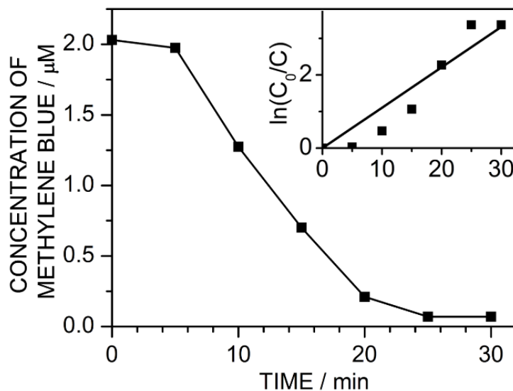
Figure 7.4: UV photodegradation profile of methylene blue dye solution ( 2 \mu\text{M} in high purity water, +70 wt%, TCL UK Ltd.) using MS( N_2/O_2 ) ( 5.6 \pm 0.1 \text{ mg mL}^{-1} ), following an initial equilibration period in the dark for 5 min. Inset shows the pseudo first-order kinetic profile with linear best fit, with a calculated photodegradation rate of 7.9 \times 10^{-3} \text{ min}^{-1} \text{ m}^{-2} .
