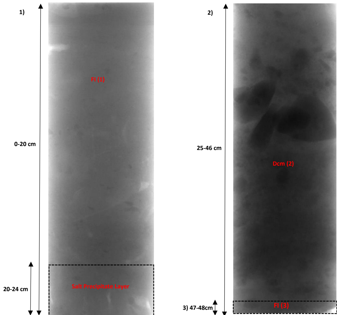
Figure 4.5: X-Rays of BC06 showing various lithofacies with the length of each facies displayed to the left of each. Each lithofacies have been numbered and corresponds to the description given above.
