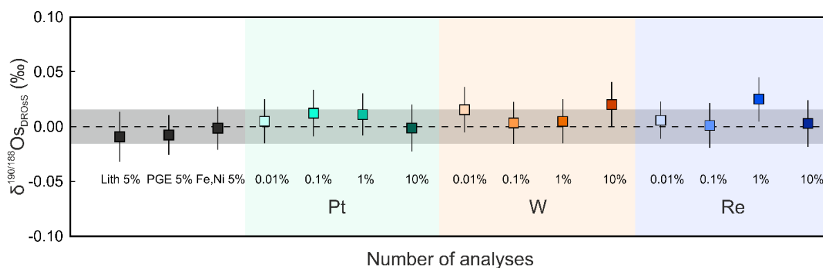
Figure 2-3 Results of doping tests to assess the robustness of the method against residual matrix effects on the MC-ICP-MS. Data show that all measurements display \delta^{190/188}\text{Os} compositions within analytical uncertainty of undoped DROs analyses for residual element abundances up to 10 % of the total Os concentration. The percentages indicate the presence of each named element at x% of the Os abundance, e.g. Si was present at 5% of the Os abundance. The black dotted line indicates the average DROs value with the \pm 2 sd represented by the grey shaded band as obtained in this study by MC-ICP-MS. Lith = lithophile elements (Si, Al, Mg, Fe, Ca, Ti, Ni, and Cr); PGE = Platinum Group Elements (Ru, Rh, Pd, Ir, and Pt).
