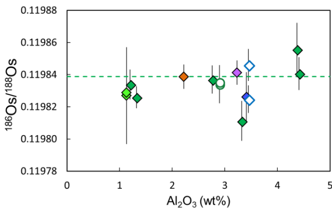
Figure 3-12 The \text{Al}_2\text{O}_3 (wt%), as a proxy of melt depletion, versus ^{186}\text{Os}/^{188}\text{Os} for Kilbourne Hole samples. All ^{186}\text{Os}/^{188}\text{Os} ratios are within analytical uncertainty of the primitive upper mantle (PUM) value (dashed line) as determined by Day et al. (2016; 0.119839 \pm 3 ). Symbols for Kilbourne Hole as in Figure 3-10 and 3-11.
