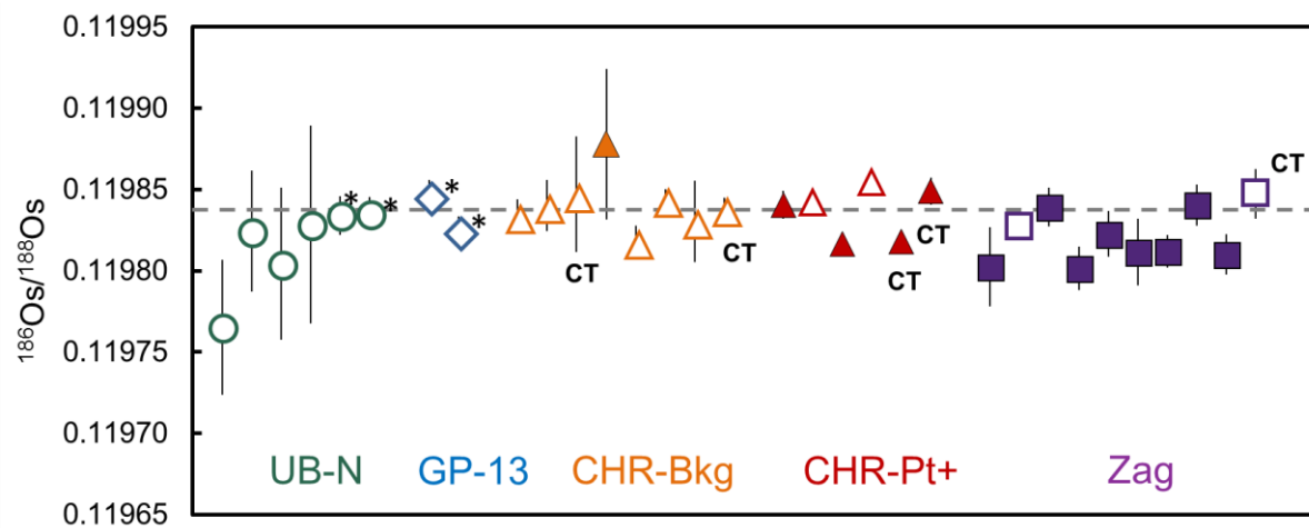
Figure I – 1b Revised Figure 2-11. Data was obtained using the DROsS isotope composition of Luguet et al. (2008). Where in the original figure the 186 Os/ 188 Os ratios plot consistently lower (see figure above) compared to the upper mantle value, the data below are, in general, within analytical uncertainty of the upper mantle value.
