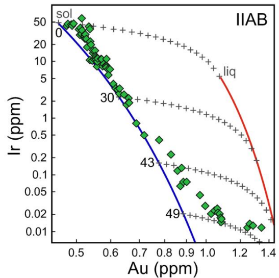
Figure 4-1 Elemental trend of \log[\text{Ir}] vs \log[\text{Au}] for IIAB iron meteorites, after Wasson et al. (2007). The solid lines indicate the estimated solid trend (blue) and liquid trend (red) in case of simple fractional crystallization. The green diamonds represent sample compositions. Wasson et al. (2007) explain their offset from the fractional crystallization trend by trapping of various amounts of melt. The amount can be estimated by the crosses, 5% between each cross, at 0%, 30%, 43% and 49% of crystallization.
