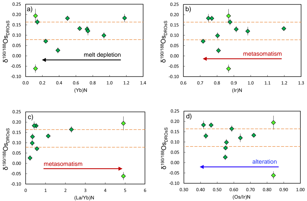
Figure 3-14 These figures reflect the various approaches that are illustrated in Figure 3-16 to quantify the effect of (a) melt depletion by (Yb)_N , (b, c) metasomatism by (Ir)_N and (La/Yb)_N , and (d) alteration using Os/Ir_N as a proxy. No systematic co-variation between \delta^{190}Os and any of the proxies is observed. Trace element and PGE data were taken from Harvey et al. (2011), and Harvey et al. (2012), and values were normalised against primitive upper mantle (underscore “N”) values determined by Palme and O’Neill (2003) for La and Yb and Becker et al. (2006) for Os and Ir. Arrows points towards and increasing degree of a certain process.
