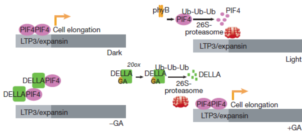
Figure 1.10: The mechanism of cell elongation under different condition. PIF4 mediates cell elongation in the dark condition. When exposed to the light, phyB degrades PIF4 and inhibits cell elongation. Due to DELLA protein accumulation in the absence of GA, PIF4 is bound to DELLA protein and no expansion can be observed. However, the addition of GA degrades DELLA protein and increases the free PIF4, hence cell elongation can be promoted. Figure was taken from de Lucas et al., 2008.
