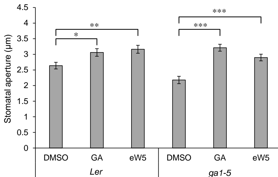
Figure 6.8: The stomatal aperture of ga1-5 mutants after the application of GA and eW5 at 100µM concentration. The assay was conducted in a minimum source of light and performed in three replicates. Error bars represent standard errors. Asterisks indicate statistically significant differences (independent t-test, * P < 0.05 , ** P < 0.005 , *** P < 0.001 ) between chemical treatment.
