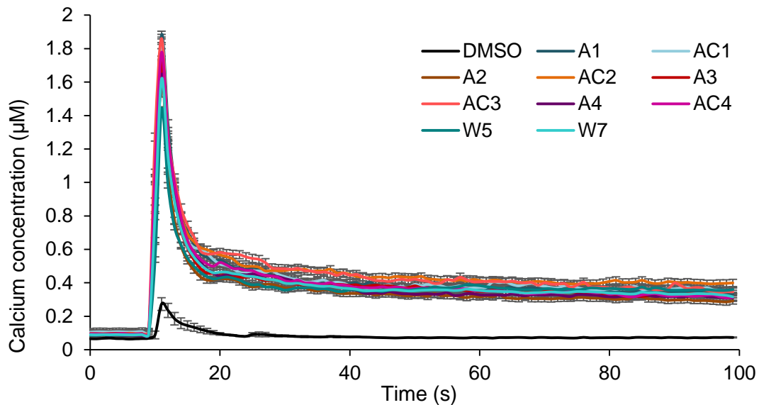
Figure 3.7: Cytosolic calcium response upon chemicals application at the concentration of 25 \mu\text{M} . DMSO was used as a control and the data presented was based on three biological replicates.
