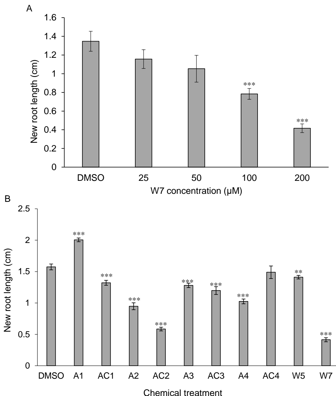
Figure 3.4: Root growth analysis of 7th days old seedlings after 5 days of chemical treatment. Error bars represent standard error of 18 seedlings. A) The experiment was performed at different concentration of W7 to choose the concentration to be used for the rest of the chemicals. B) The screening of the compounds in the series at the concentration of 100 μM. Asterisks indicate statistically significant differences (independent t-test, ** P<0.005, *** P<0.001) between DMSO and chemical treatment.
