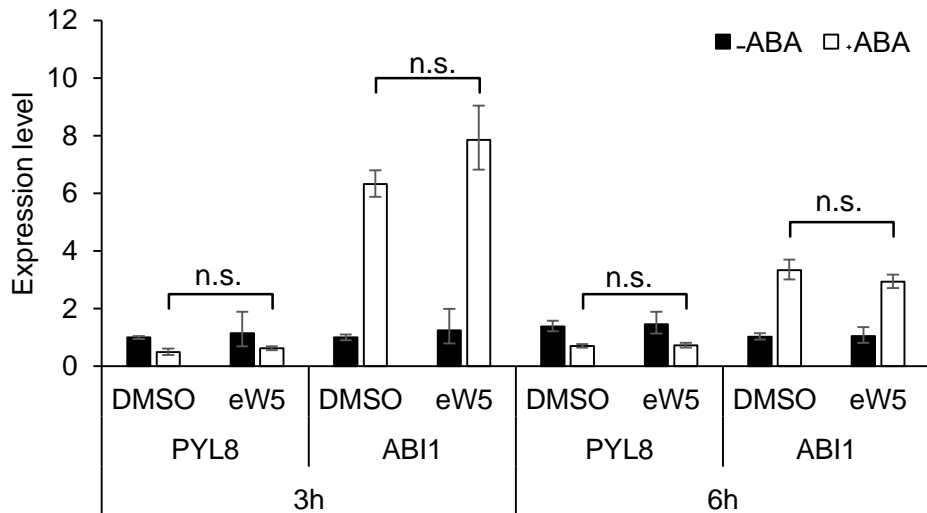
Figure 5.12: The expression levels of ABI1 and PYL8 to investigate the effect of eW5 on genes encode ABA signalling components, protein phosphatase and ABA receptor. The experiment was conducted in three replicates and the error bars represent standard error.
