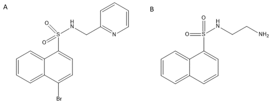
Figure 5.1: Structural similarity between A) pyrabactin and B) eW5. Both of the compounds have sulfonamide moieties that attached to naphthalene ring.
