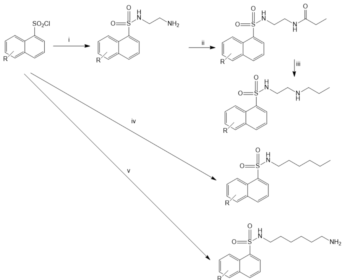
Figure 3.3: The schematic reaction for the synthesis of the analogues. i) ethylene diamine, \text{CH}_2\text{Cl}_2 ; ii) propionic anhydride, \text{Et}_3\text{N} , \text{CH}_2\text{Cl}_2 ; iii) \text{BH}_3 \cdot \text{THF} , \text{THF} ; iv) hexylamine, \text{Et}_3\text{N} , \text{CH}_2\text{Cl}_2 ; v) 1,6-diaminehexane, \text{CH}_2\text{Cl}_2 .
