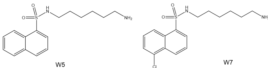
Figure 3.1: The structural similarity between W5 and W7 where W7 has a chlorine substituent at its C-5 naphthalene ring position.
