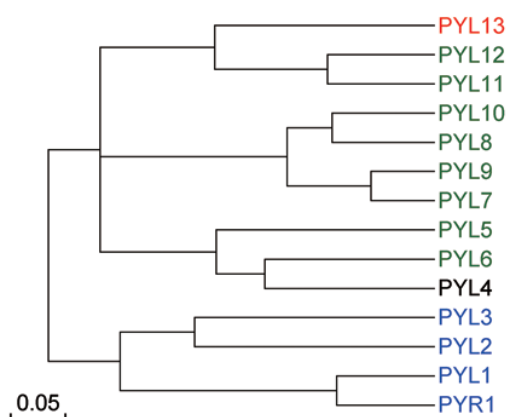
Figure 1.3: The classification PYR/PYLs ABA receptors based on phylogenetic tree analysis. The receptors classified in green colour can interact with PP2Cs in the absence of ABA, while receptors in blue colour are ABA-dependent to interact with PP2C.
