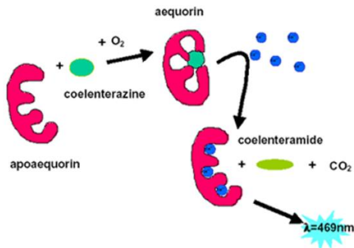
Figure 3.5: Reaction of coelenterazine and apoaequorin that lead to the emission of blue light that will be detected by luminometer. Figure was adapted from Mithofer and Mazars (2002).
