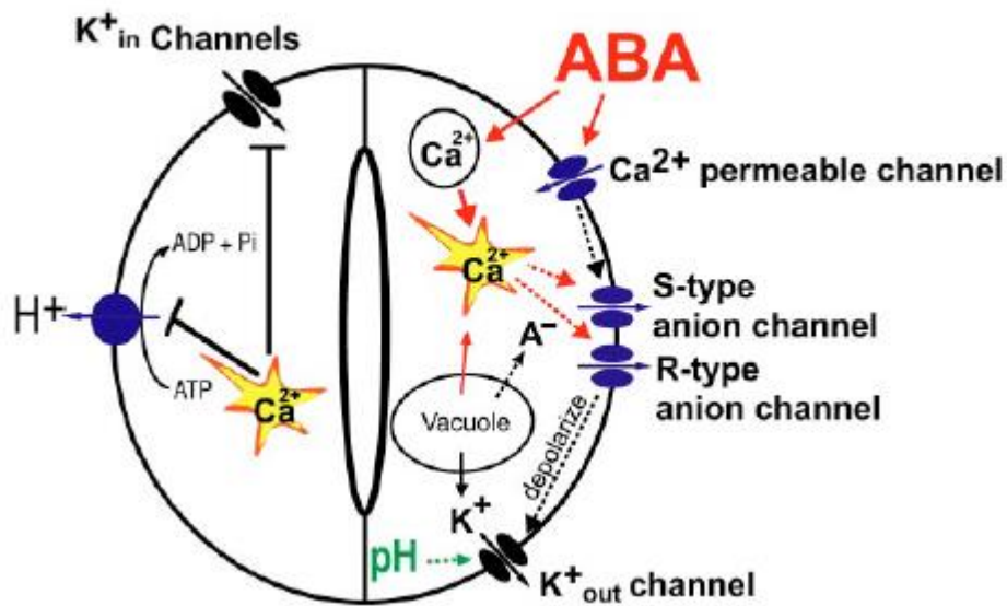
Figure 1.6: A guard cell model. ABA increases the concentration of [Ca^{2+}] . The influx of Ca^{2+} initiates the intracellular Ca^{2+} transient and release Ca^{2+} from vacuoles. Higher [Ca^{2+}] activates anion channel and caused depolarization.
