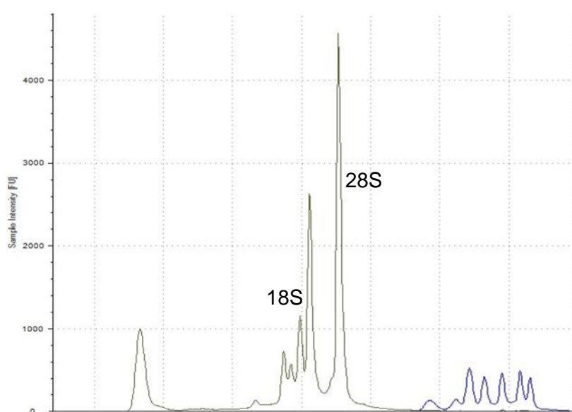
Figure 4.3: An electropherogram of an RNA sample used for RNA-seq analysis, which showed a high quality of RNA. The x-axis and y-axis indicate time and fluorescence signal, respectively.
