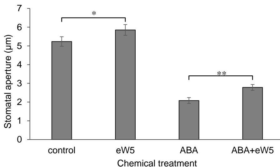
Figure 5.9: Inhibitory effect of eW5 on the size of the stomatal. The stomatal aperture was measured after two hours of chemical treatment. Error bars represent standard error. The experiment was performed in three biological replicates, with 3 peels (10 pores per peel) for each replicate. Asterisks indicate statistically significant differences (independent t-test, * P < 0.05 , ** P < 0.005 ) between chemical treatment.
