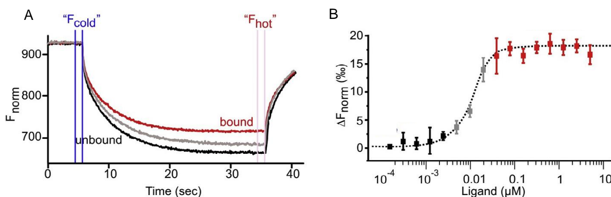
Figure 5.4: A) The MST time traces of the capillaries containing the protein and ligand solution. B) The normalized fluorescence of the MST traces plotted against the concentration of the ligands. The figure was taken from Jerabek-Willemsen et al., 2014.
