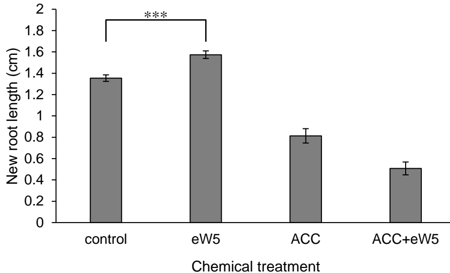
Figure 5.8: Root growth assay to investigate the competition study between eW5 and ethylene precursor, ACC. Chemical treatment was performed for 5 days using seven-day old seedlings. The experiment was conducted using at least 18 seedlings. Asterisks indicate statistically significant differences (independent t-test, *** P < 0.001 ) between chemical treatment.
