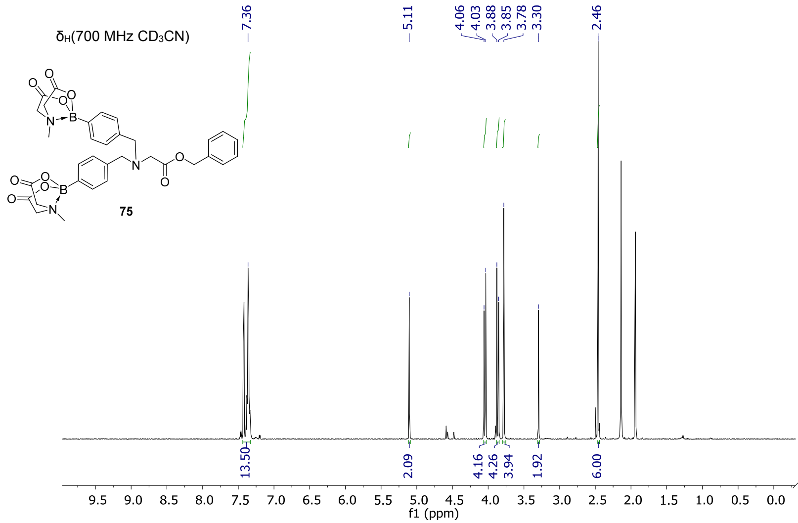
Figure A6 1 H NMR of di-MIDA ester 75 .
