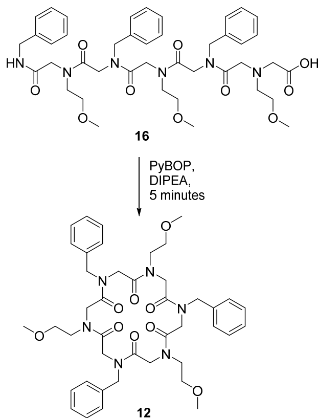
Scheme 1.6 Head to tail cyclisation of a linear peptoid ( 16 ) hexamer to form a cyclohexamer ( 12 ).
