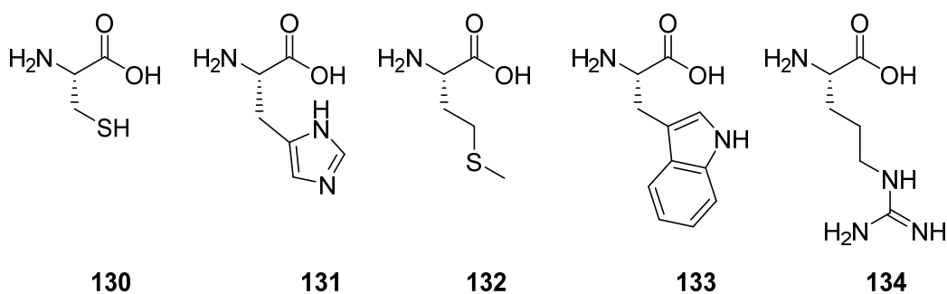
Figure 3.8 Amino acids in the p15 peptide that are prone to side-reactions (including racemisation) during synthesis or cleavage: cysteine ( 130 ), histidine ( 131 ), methionine ( 132 ), tryptophan ( 133 ) and arginine ( 134 ).
