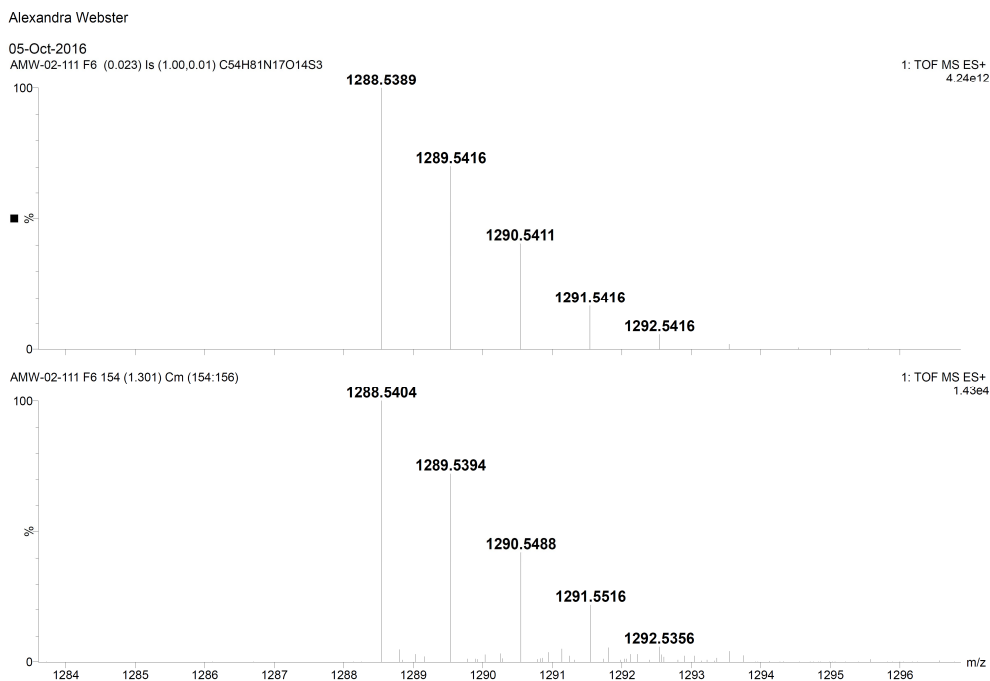
Figure C2 HRMS of disulphide-bridged p15 peptide 126 , C 54 H 81 N 17 O 14 S 3 , calculated [M+H] + = 1288.5389, observed [M+H] + = 1288.5404.
