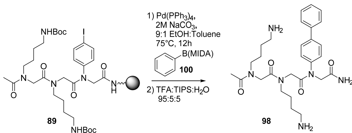
Scheme 2.25 Intermolecular Suzuki cross-coupling reaction carried out on aromatic iodide containing peptoid ( 89 ).
