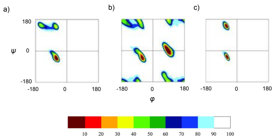
Figure 1.9 Experimentally observed Ramachandran plots of allowed dihedral angles ( \varphi and \psi ). The plot is colour coded according to the percentage of total amino acids in each area, i.e 10% of all amino acids are in the dark red areas, which make them the most densely populated. The white area typically takes up about 80 – 90% of the total area but only contains 10% of all amino acids: a) Observed regions for alanine. The region in the lower left quadrant is characteristic of the \alpha -helical conformation. The region in the upper left quadrant contains two maxima and is the \beta -sheet region; b) Observed regions for glycine. Glycine has more allowed regions as a result of its lack of side-chain. This results in fewer steric clashes with neighbouring groups and hence can adopt a wider range of conformations; c) Observed regions for proline. Proline is a five membered ring about the backbone amide which restricts \varphi to about -65^\circ resulting in fewer favourable conformations. Ramachandran plots obtained from Hovmöller et al. , Acta Cryst. D. , (2002), 58 , 768-776. Reproduced with permission of the International Union of Crystallography, https://journals.iucr.org
