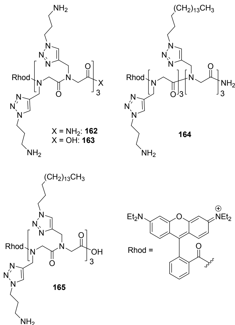
Figure 4.2 Structures of cell-penetrating peptoids made using CuAAC by S. B. L. Vollrath et al.
