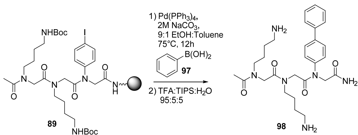
Scheme 2.23 Intermolecular Suzuki cross-coupling reaction carried out on aromatic iodide containing peptoid ( 89 ).
