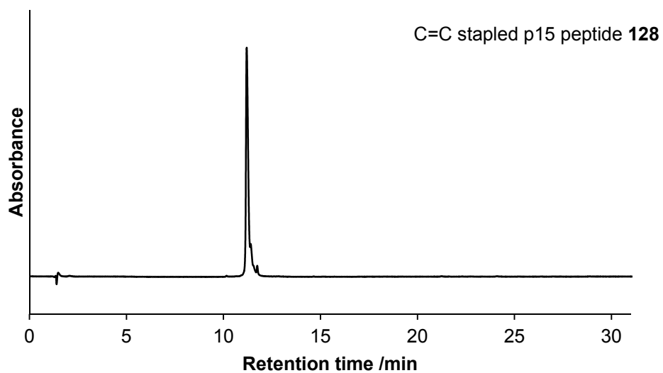
Figure 3.26 Analytical HPLC trace of purified C=C stapled p15 peptide ( 128 ), \lambda = 280 nm.
