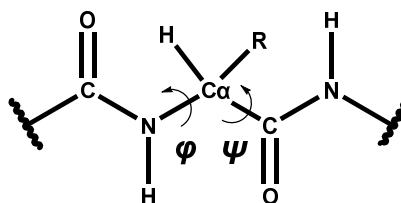
Figure 1.8 The dihedral angles of amino acids in a peptide backbone. The angle between N and C\alpha is \varphi and the angle between C\alpha and the carbonyl carbon is \psi .
