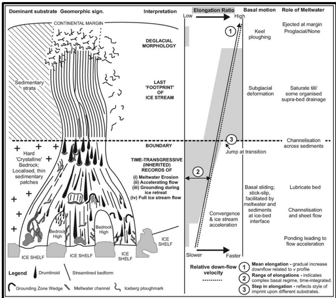
Figure 2.9 - A model for palaeo-ice stream landforms on the West Antarctic continental shelf. This schematic illustrates the landsystem assemblages interpreted, the velocity inferred, the role of meltwater and bedform elongation (Graham et al., 2009).
