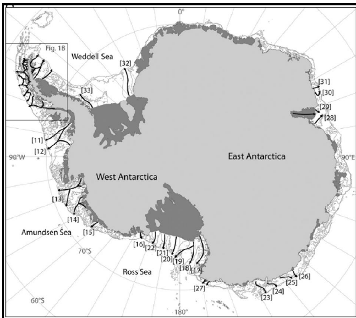
Figure 2.4 - Locations of the main palaeo-ice streams known on the Antarctic continental shelf. Approximate locations of ice streams are depicted by a black arrow and the numbers refer to corresponding citation and evidence outlined in Livingstone et al. , 2012.
