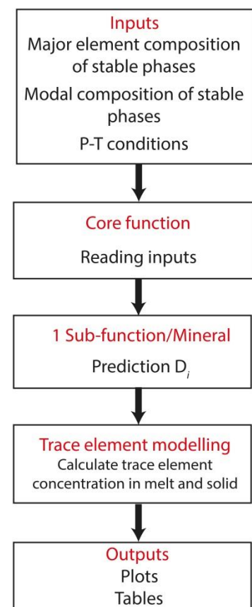
Figure 4-1: Flow diagram of TEPM displaying the computational development of the code.
