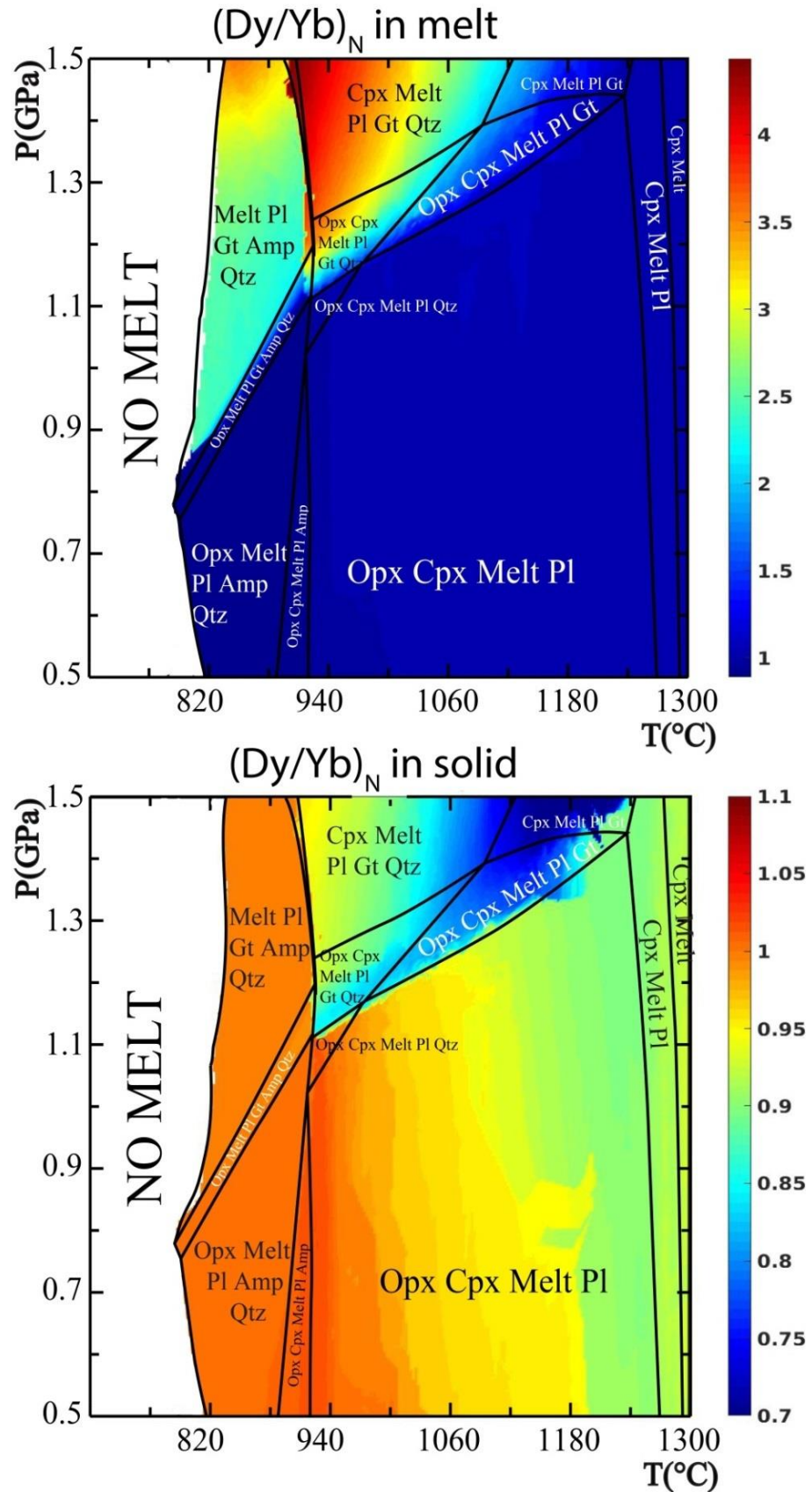
Figure 4-11: P - T grids of (\frac{Dy}{Yb})_N behaviour in an amphibolite system calculated from the coupling of TEPM and Perple_X . Top: (\frac{Dy}{Yb})_N evolution in the melt (see text for explanations); Bottom: (\frac{Dy}{Yb})_N evolution in the bulk solid (see text for explanations).
