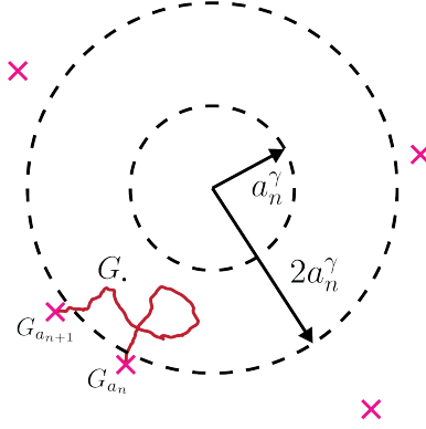
Figure 8.1: Controlling G_n along a subsequence.
