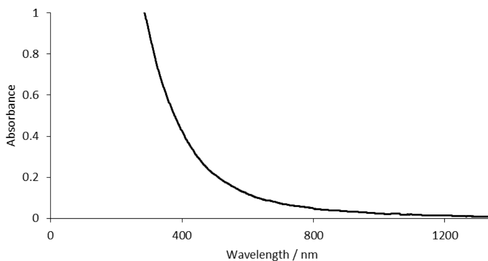
Figure 3.23. UV-vis spectra for unwashed platinum/PVP nps, recorded in ethanol at 1\text{mg mL}^{-1} concentration. Spectra are shown up to 1350 nm due to the detection limit of the instrument.
