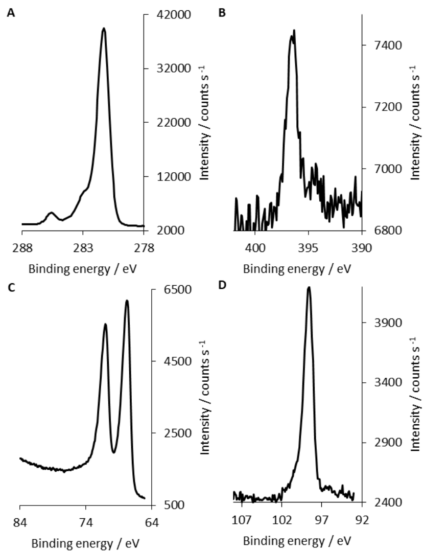
Figure 3A.16. XP spectra for sample three of five for the second five points surveyed for platinum/PVP nps supported using LB techniques upon a silica window (with one dipping of the substrate within the trough) for the following elements and bands: A) carbon 1s, B) nitrogen 1s, C) platinum 4f, and D) silicon 2p.
