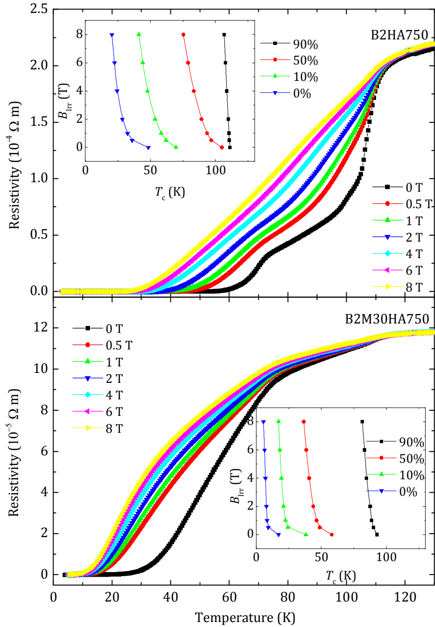
Figure 6.7: Upper panel: Resistivity of the B2HA750 sample measured in fields of 0 T – 8 T with a constant excitation current of 5 mA. Inset: B_{Irr} determined using the criteria of 90%, 50% and 10% of \rho_N(0 \text{ T}, 120 \text{ K}) , and zero resistivity ( 0\% \rho_N ). Lower panel: Equivalent data for the B2M30HA750 sample.
