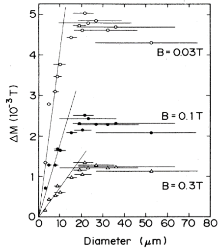
Figure 3.8: Magnetisation loop width as a function of particle diameter in YBCO, measured at 0.03 T, 0.1 T and 0.3 T and 77 K [56].
