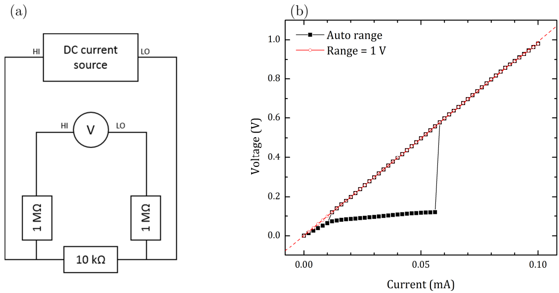
Figure 5.7: (a) Circuit used to reproduce the V - I hysteresis in which a 10\text{ k}\Omega resistor represents a nanocrystalline sample and the 1\text{ M}\Omega resistors represent high contact resistances at the voltage taps. (b) V - I characteristics obtained with this circuit. The hysteresis was seen when the Keithley DMM 2100 was set to auto range whereas the standard Ohmic behaviour was seen when range was set to 1\text{ V} .
