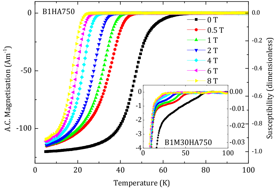
Figure 6.9: A.c. magnetic susceptibility as a function of temperature of the B1HA750 sample. The data were taken with an excitation field of 0.4 mT and at a frequency of 777 Hz. Inset: Equivalent data for the B1M30HA750 sample.
