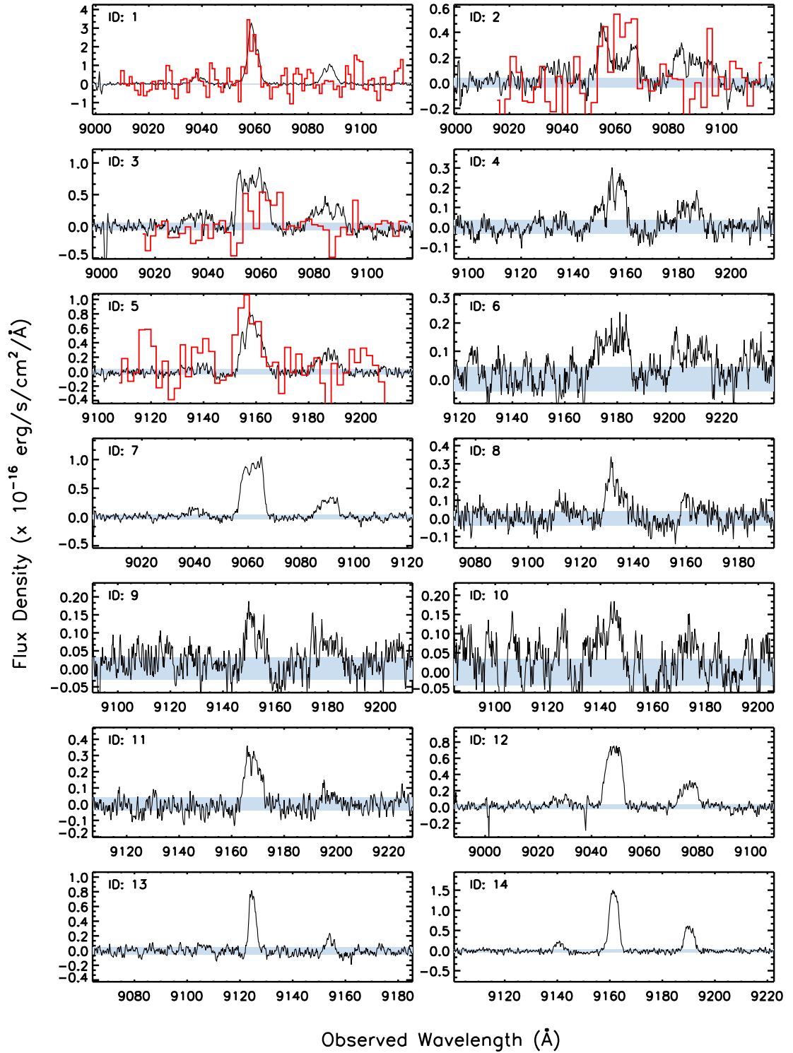
Figure 2.3: Integrated spectra around redshifted H\alpha and [NII] (6548,6583) emission lines. Parameters such as redshifts and [NII]/H\alpha ratios are listed in Table 2.1. Many galaxies show split emission line profiles, indicative of high velocity rotation and possibly strong obscuration towards the dynamical centre. We suspect the dynamics of galaxy IDs 23 and 24 may be affected by an AGN. For IDs 1, 2, 3, 5 and 16 we overlay the CO spectra in red, and find that the velocity centroid and line width are well matched to the H\alpha emission. Shaded regions show the \pm 1\sigma noise, measured at wavelengths away from the H\alpha and any residual sky emission.
