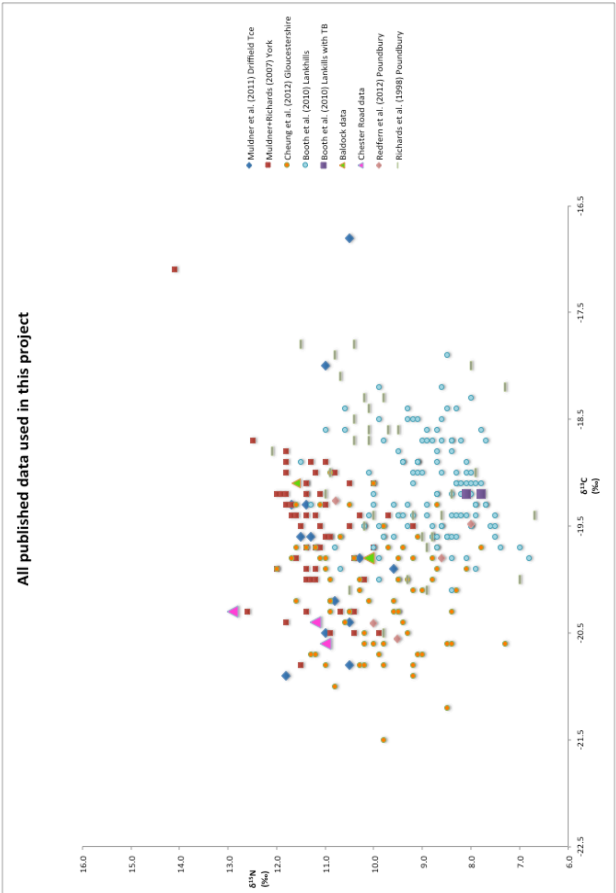
Fig. 8.5 All published carbon and nitrogen isotope data for the sites used in this project
