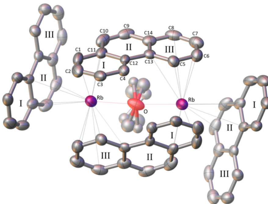
Figure 27: Coordination environment of \text{Rb}^+ ions in \text{Rb}_2(\text{C}_{14}\text{H}_{10})_2(\text{THF}) compound. The two outer benzene ring planes are labelled as I, III, and the central plane as II. Black dotted lines and red dotted lines represent \text{Rb}^+\cdots\text{C} and \text{Rb}^+\cdots\text{O} coordination interactions respectively. Colour code: Rb violet; O red and C grey. Hydrogen atoms are omitted for clarity. Thermal ellipsoids are shown with 50% probability level and the occupancy of carbon atoms in THF molecule were fixed to 0.5. Depicted structure was obtained from data collected at 120 K.
