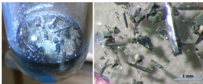
Figure 81: Isolated product in reaction vessel (left panel) and single crystals of \text{Rb}_4(\text{C}_{14}\text{H}_{10})_3(\text{THF})_4 , along with some olive green powder under 40 \times magnification (right panel). Thick pale blue line represents 1mm length.
