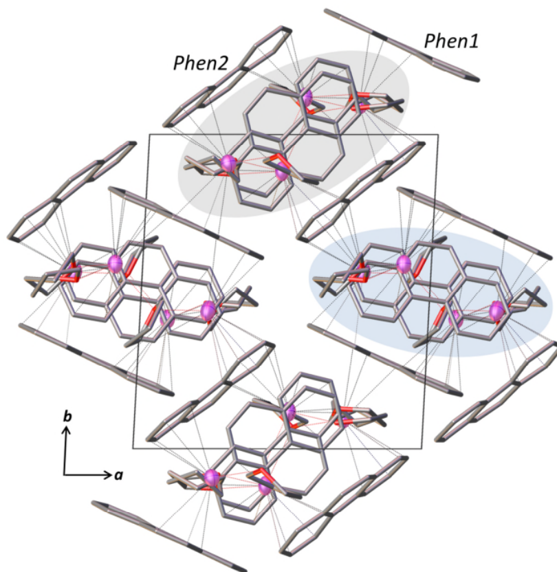
Figure 74: Projection of K_4(C_{14}H_{10})_3(THF)_4 structure along the [001] direction showing four channel-like motifs forming a 3D polymeric network of K^+ \cdots C interaction (black dotted lines) between alkali metal ions and the phenanthrene radical anions. The pale grey and the pale blue ellipses present chains comprised of Phen3' , THF3 , THF4 , K3^+ and K4^+ , and Phen3'' , THF1 , THF2 , K1^+ and K2^+ respectively. Hydrogen atoms are omitted, and carbon-carbon and carbon-oxygen bonds are depicted as tubes for clarity. Colour code: K lilac; O red and C grey, red dotted lines represent K^+ \cdots O coordination.
