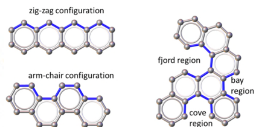
Figure 3: The periphery of PAHs represented by colouring of C-C bonds in blue.
