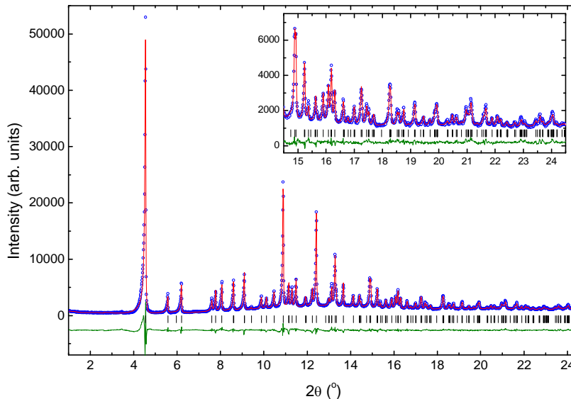
Figure 32: Powder diffraction of the rubidium phenanthridine sample. The experimentally obtained diffraction profile ( \lambda = 0.7093 \text{ \AA} , Mo K\alpha ) at 294 K (blue open circles), the calculated profile (red solid line), difference (olive green solid line) and predicted peak position (black tick marks). The inset shows high 2\theta region. The weight profile and expected R factors are R_{wp} = 7.606\% and R_{exp} = 2.334\% .
