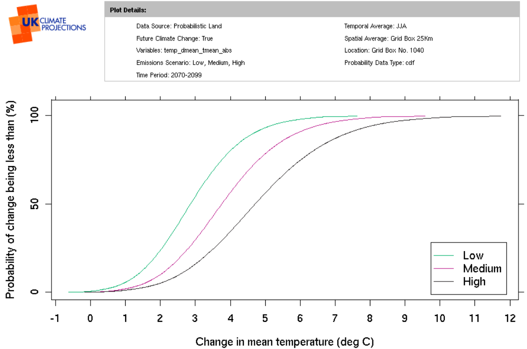
Figure 2.6 Projected changes in Newby Beck mean summer temperatures. © UK Climate Projections 2009
