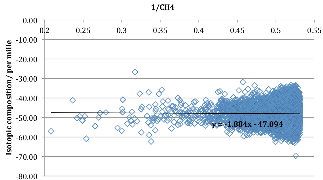
Figure 3.11: KM5 wellpad isotopic composition from 20/10/2015
