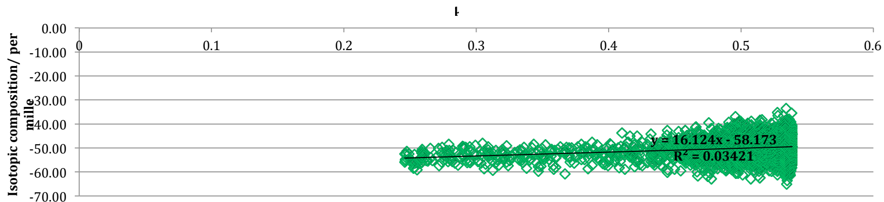
Figure 3.12: KM5 wellpad isotopic composition from 20/7/2016
