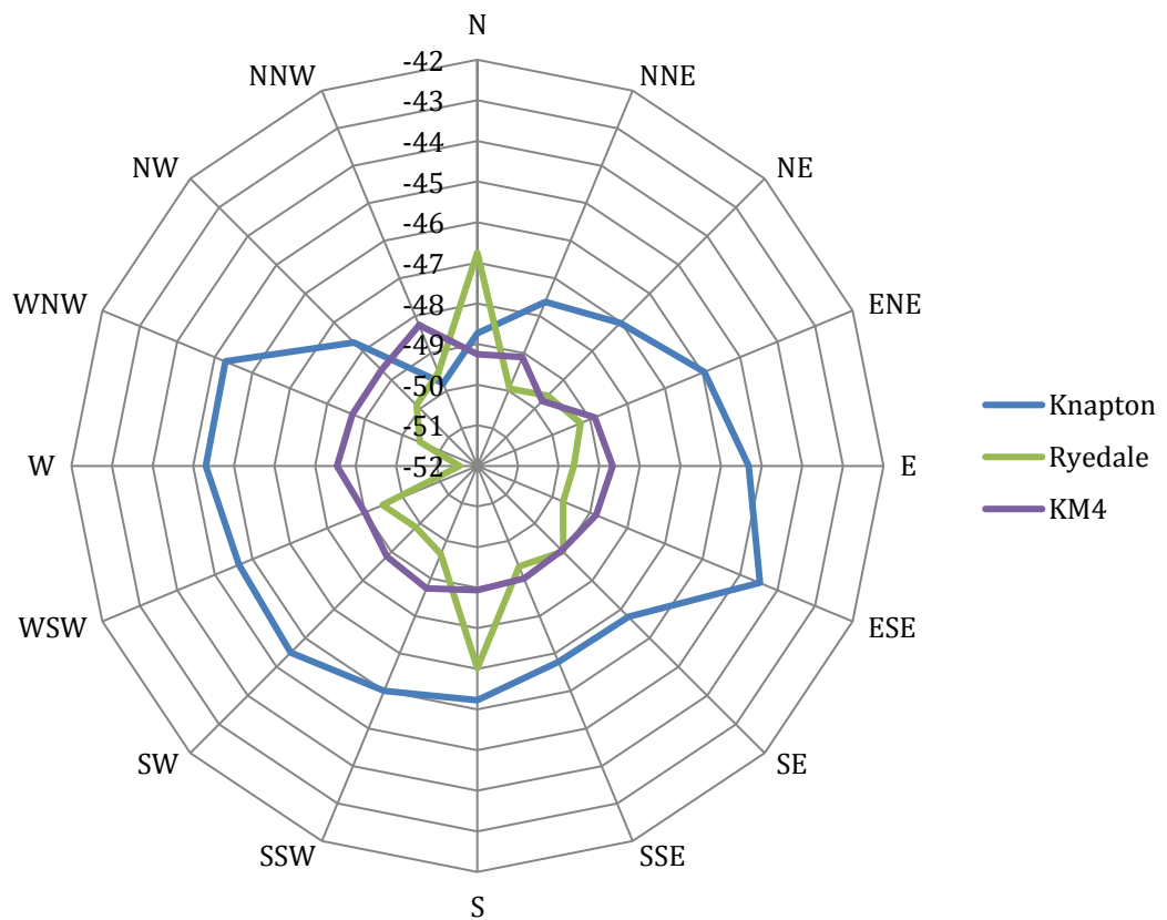
Figure 3.19: Isotopic composition of Knapton generation station (knapton), KM5 wellpad (KM4) and Cranford House control site (Ryedale)
