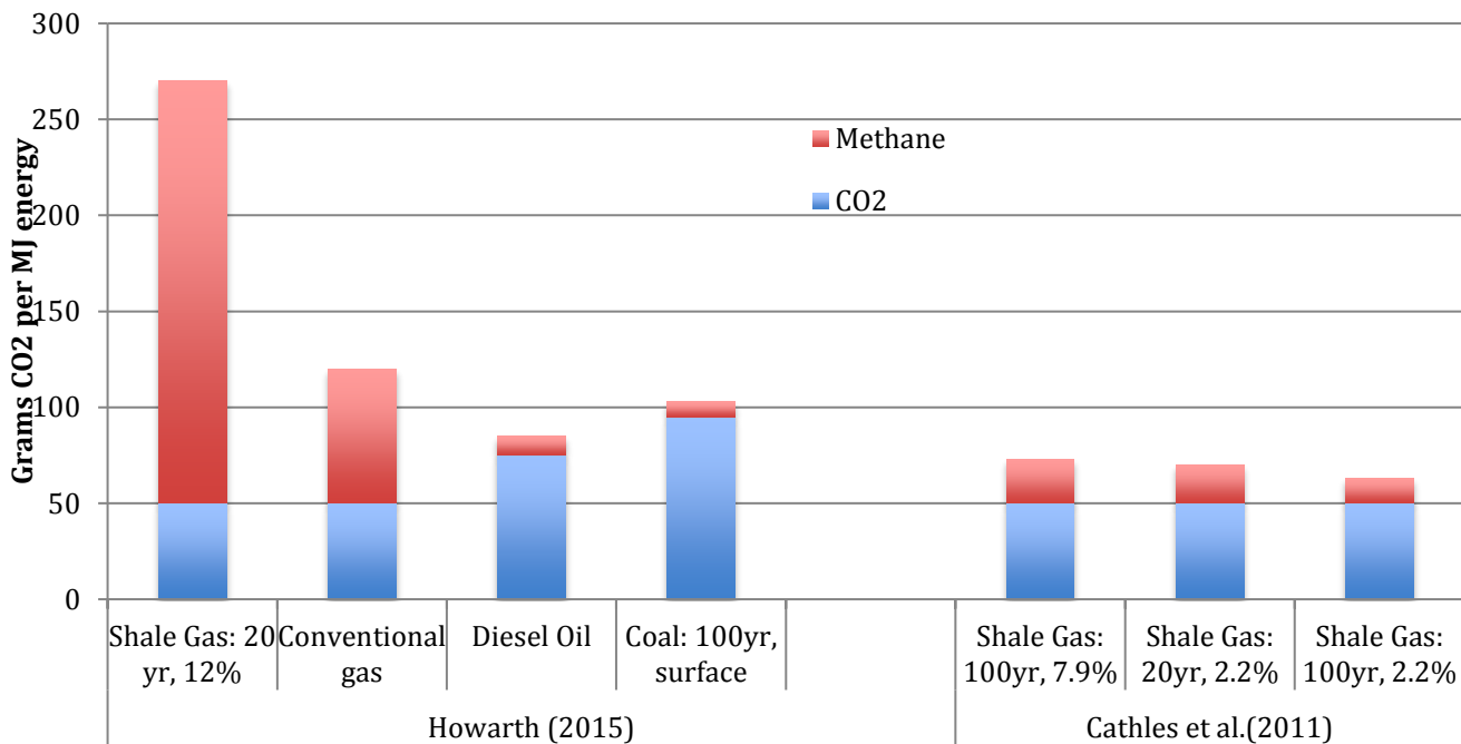
Figure 4.5 :The climatic effects and comparison of fuel source emissions under specific scenarios (Source: Howarth (2015) and Cathles et al. (2011))
