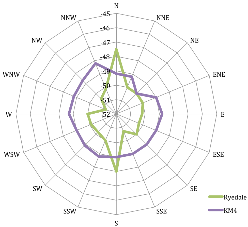
Figure 3.13: KM5 (KM4) and Cranford Farm (Ryedale) control isotopic composition
