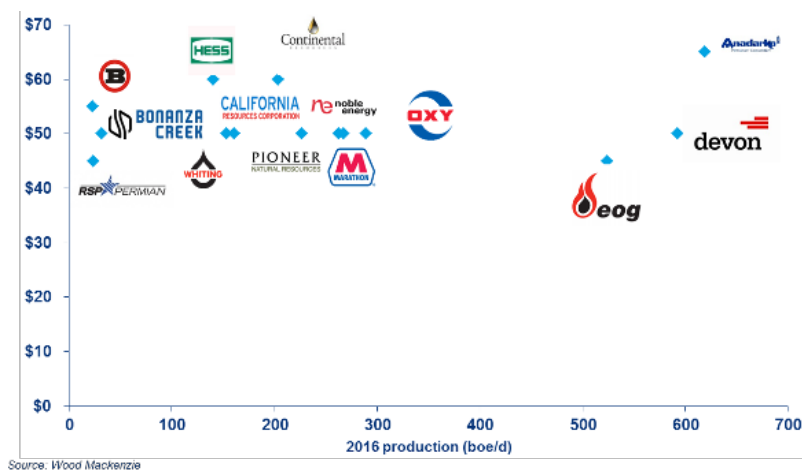
Figure 1.3: Price requirements for shale gas production to be profitable (Wood MacKenzie, 2014)
