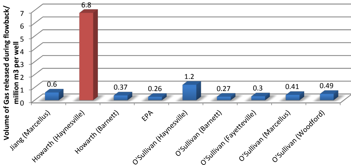
Figure 1.7: Comparison of well completion flowback emissions from different unconventional wells
