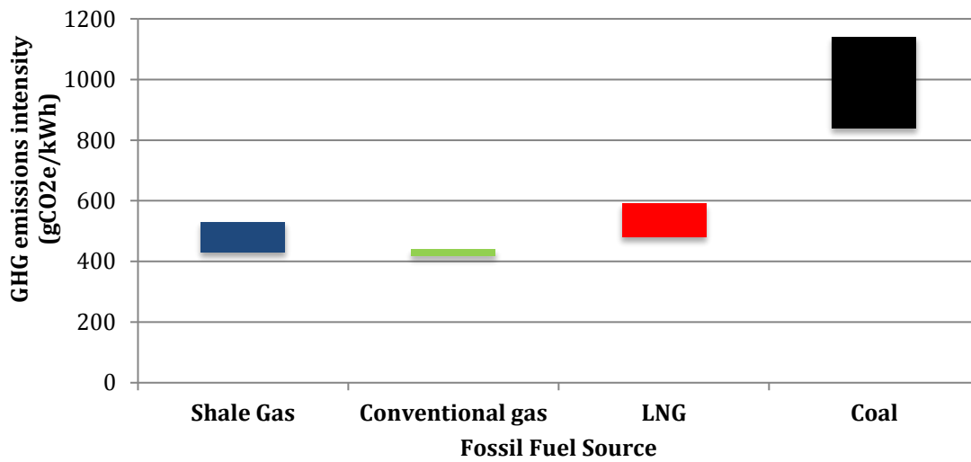
Figure 4.3: Emissions from fossil fuel sources (adapted from Mackay and Stone, 2013)
