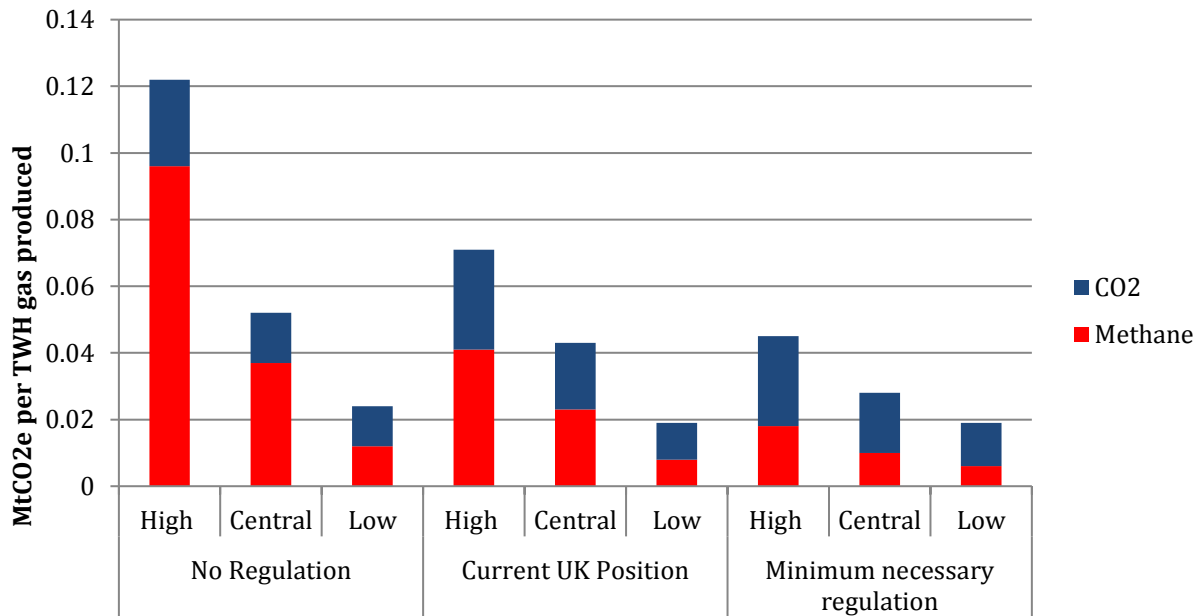
Figure 4.4: Emissions per tWh from shale gas exploitation under different regulation scenarios (Source: Committee on Climate Change, 2016)
