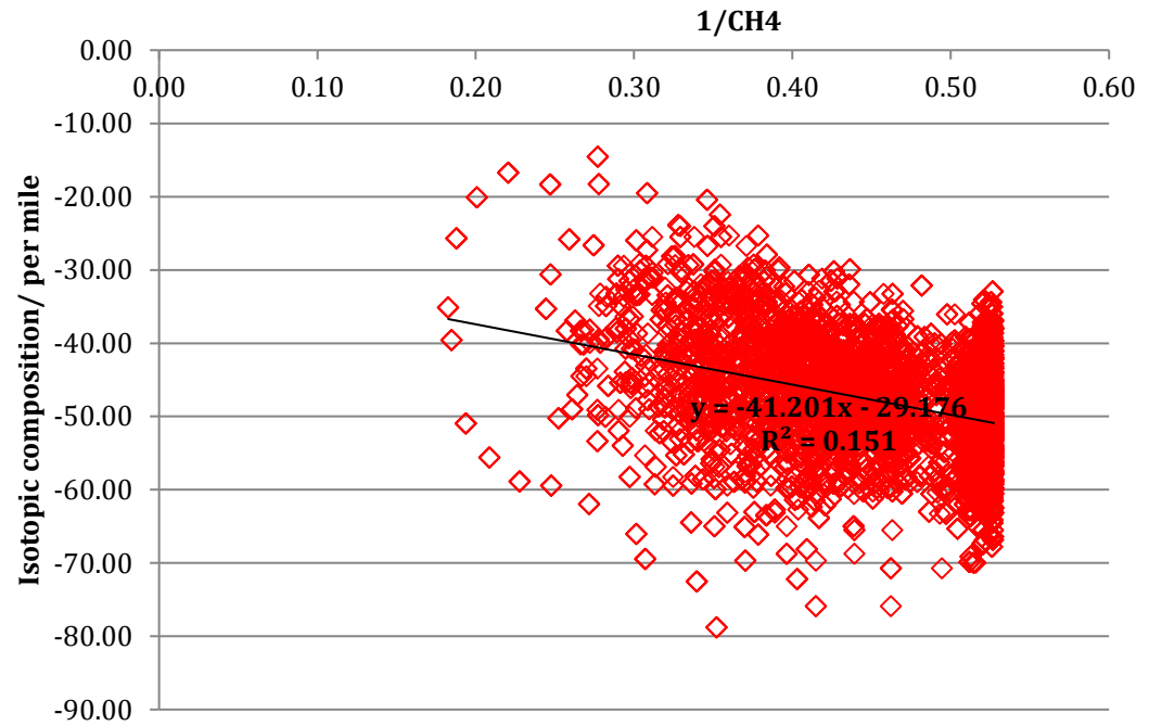
Figure 3.17: Isotopic composition of Knapton methane measurements from the 29/4/16
