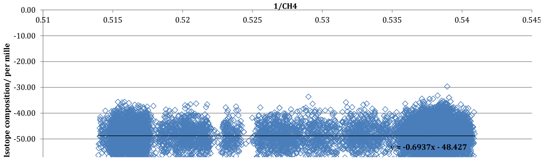
Figure 3.5: Methane isotopic composition from 21/10/16 at Cranford House
