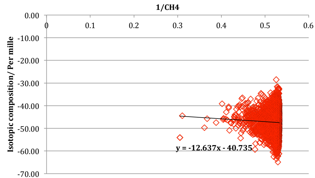
Figure 3.10: KM5 wellpad isotopic composition from 13/10/2015
