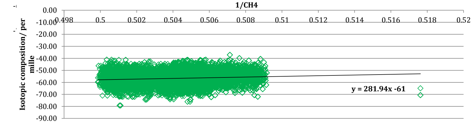
Figure 3.6: Methane isotopic composition from 9/5/16 at Cranford House
