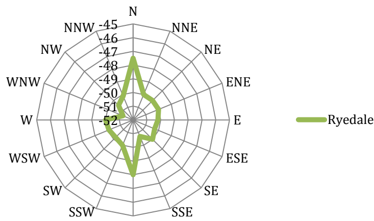
Figure 3.4: Cranford House (Ryedale) Isotopic composition
