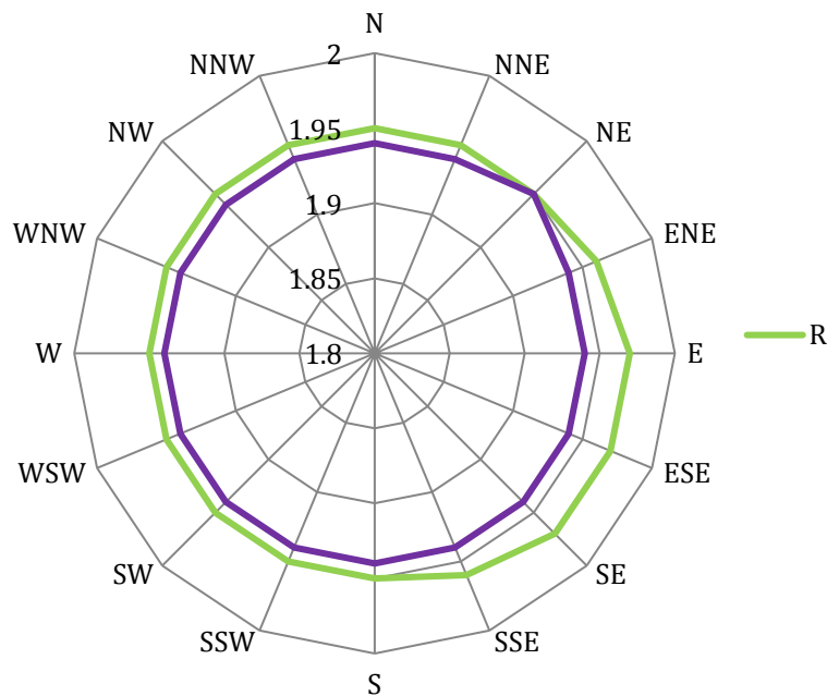
Figure 3.7: Average methane concentration at KM5 (purple) and Cranford House control site (R)
