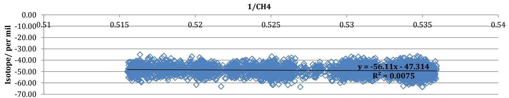
Figure 3.18: Isotopic composition of Knapton methane measurements from the 26/7/16
