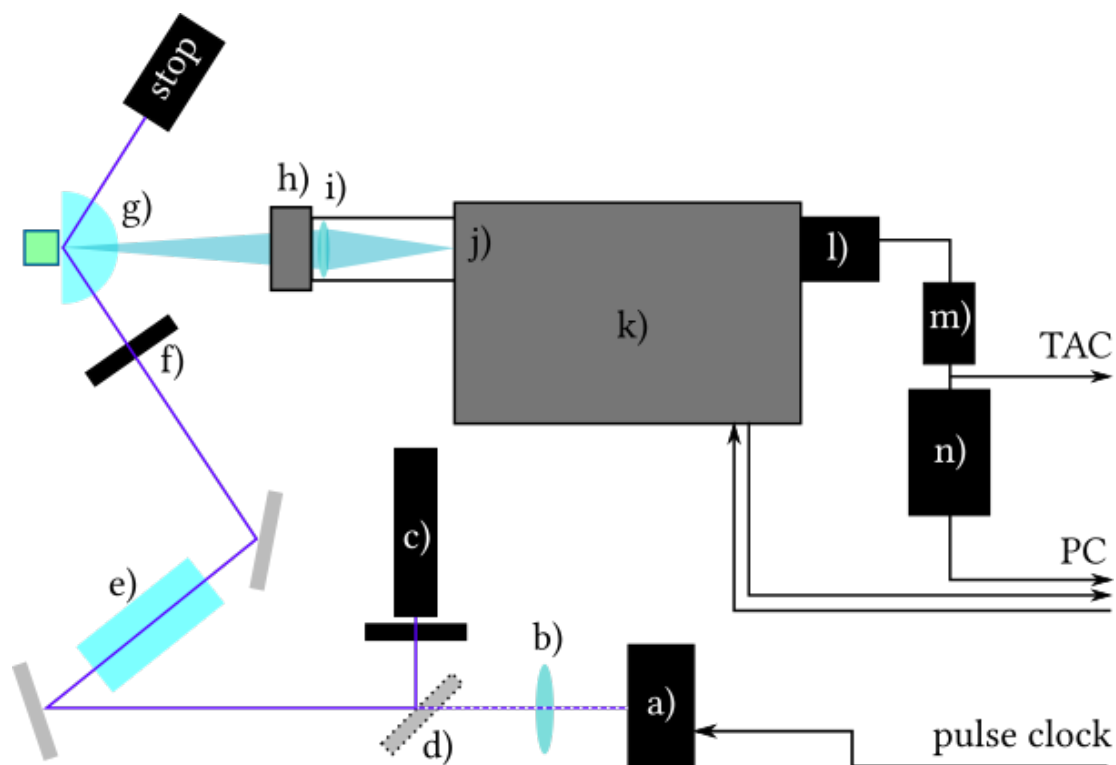
FIGURE 3.1: EWIFS SPECTROMETER LAYOUT: Schematic representation of the EWIFS instrument, viewed from above. Note the collinearity of the CW and pulsed beams after the flip-mirror. a) pulsed laser; b) collimation lens; c) CW laser; d) flip-mirror; e) double fresnel rhomb; f) scatter cleanup aperture; g) TIR element and beam stop; h) Glan-Thompson prism; i) f-matching lens; j) position of filter wheel; k) monochromator; l) photomultiplier; m) PMT power control; n) DAQ unit. Beam path shown in purple, data and signal travel along black arrows.
