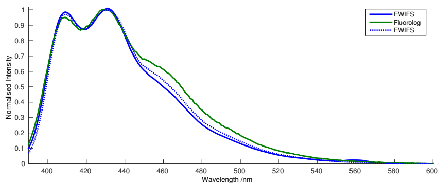
FIGURE 3.7: COMPARISON OF EWIFS INSTRUMENT WITH HORIBA FLUOROLOG: The two instruments produce comparable spectral forms for an OB49/DMSO standard.
