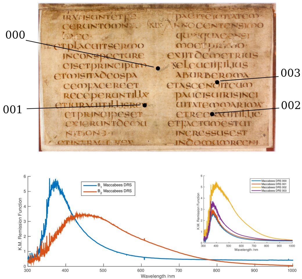
FIGURE 8.22: DCL B.IV.16 f. 169 Maccabees. Top: f. 169 and DRS spectra locations. Bottom: NMF basis functions of the F(R) spectra. Bottom inset: F(R) spectra.
