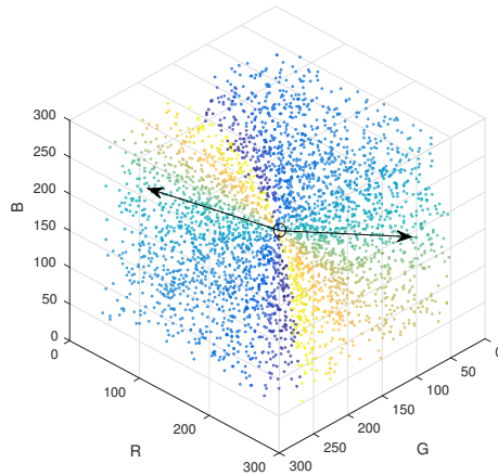
FIGURE 7.8: SCATTER GRAPHS OF sRGB TO L * A * B * CONVERSION: ARCTAN(B * /A * ): The a * b * values from figure 7.7 have been converted to \theta_{a^*} = \tan^{-1}(b^*/a^*) which gives the angle between the a * axis and each a * b * co-ordinate expressed as a displacement vector from the grey-point ( a^* = b^* = 0 ). The points are coloured by \theta_{a^*} , and the viewing axis is along R = G = B . In this way, two general families of hue can be seen either side of the yellow-blue discontinuity ( \theta_{a^*} = \{90^\circ, 270^\circ\} ). The two vectors approximate \theta_{a^*} = \{0^\circ, 180^\circ\} , the rightmost of which is 0^\circ , with hue-angles progressing clockwise numerically through the figure.
