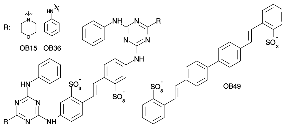
FIGURE 4.1: STRUCTURE OF OPTICAL BRIGHTENER ANIONS: Shown anions of disodium salts OB15 ( \text{Na}_2\text{C}_{40}\text{H}_{38}\text{N}_{12}\text{O}_8\text{S}_2 ; 924.91 \text{ g mol}^{-1} ), OB36 ( \text{Na}_2\text{C}_{44}\text{H}_{34}\text{N}_{12}\text{O}_6\text{S}_2 ; 936.93 \text{ g mol}^{-1} ) and OB49 ( \text{Na}_2\text{C}_{28}\text{H}_{20}\text{O}_6\text{S}_2 ; 562.56 \text{ g mol}^{-1} ).
