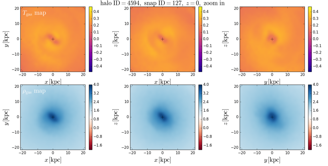
Figure 5.8: The projected halo gas temperature (upper row) and density (lower row) maps for the central region halo 4594 at z = 0 . The meanings of maps and symbols are the same as Fig. 5.7, and for more information see its caption.
