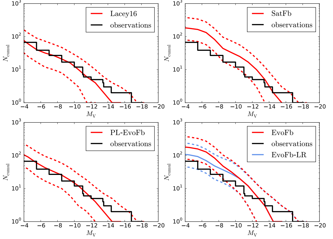
Figure 3.4: Cumulative luminosity function of satellite galaxies in Milky Way-like host halos at z = 0 . The solid black line in each panel is the observed Milky Way satellite cumulative luminosity function. For M_V < -11 , this shows the direct observational results from McConnachie (2012) , while for M_V \geq -11 , it shows the results from Koposov et al. (2008) , who applies some corrections for incompleteness in the observations. The other lines in each panel show the model predictions, with the solid red line showing the median for a sample of MW-like halos, and the dashed lines indicating the 5 – 95% range. The corresponding model names are given in the line key in each panel.
