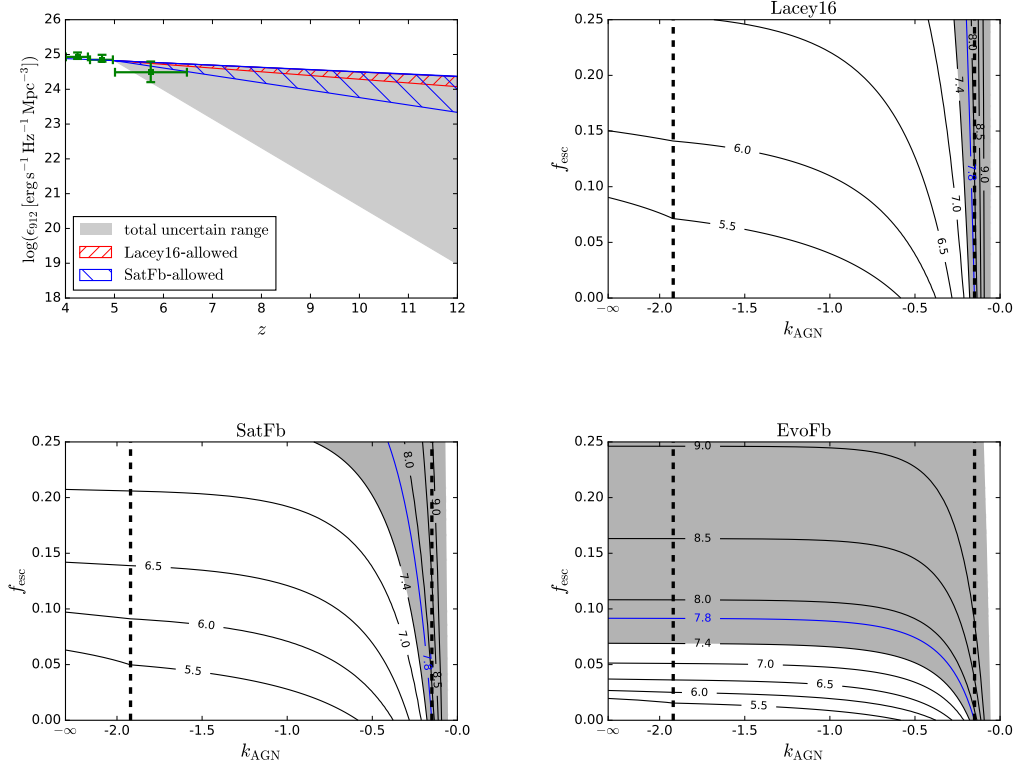
Figure 3.11: Upper left panel: extrapolations of the AGN emissivity at the Lyman limit, \epsilon_{912} , allowed by the errorbar of the measurement at z \simeq 6 . The three data points with errorbars are the observations taken from Fig. 1 of Madau & Haardt (2015) , the grey shaded region shows the allowed extrapolations. The extrapolation adopted by Madau & Haardt (2015) lies on the upper boundary of the region; the red and blue hatched regions encompass the extrapolations required to bring the Lacey16 and SatFb models respectively into agreement with the Planck constraints, for f_{\text{esc}} = 0.2 . Reducing f_{\text{esc}} shrinks these regions towards the upper boundary. Remaining three panels: predicted z_{\text{re, half}} (contour lines) for different combinations of f_{\text{esc}} and k_{\text{AGN}} , where f_{\text{esc}} is the escape fraction for stars and k_{\text{AGN}} is the slope of the AGN emissivity extrapolation shown in the upper left panel. The panels correspond to the Lacey16, SatFb and EvoFb models, as labelled. The grey shaded area in each panel represents the region allowed at 1-\sigma by the Planck data. The vertical dashed lines indicate the lower and upper limits of the extrapolation slope, i.e. k_{\text{AGN}} = -1.92 and k_{\text{AGN}} = -0.15 . The line labelled k_{\text{AGN}} = -\infty corresponds to the case of no AGN contribution.
