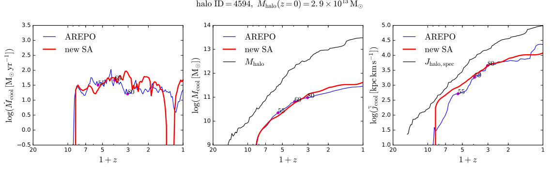
Figure 5.5: The cooling histories predicted by the SA model and simulation for halo with id 4594. The meaning of labels is the same as in Fig. 5.3, and for more information see the caption there.
