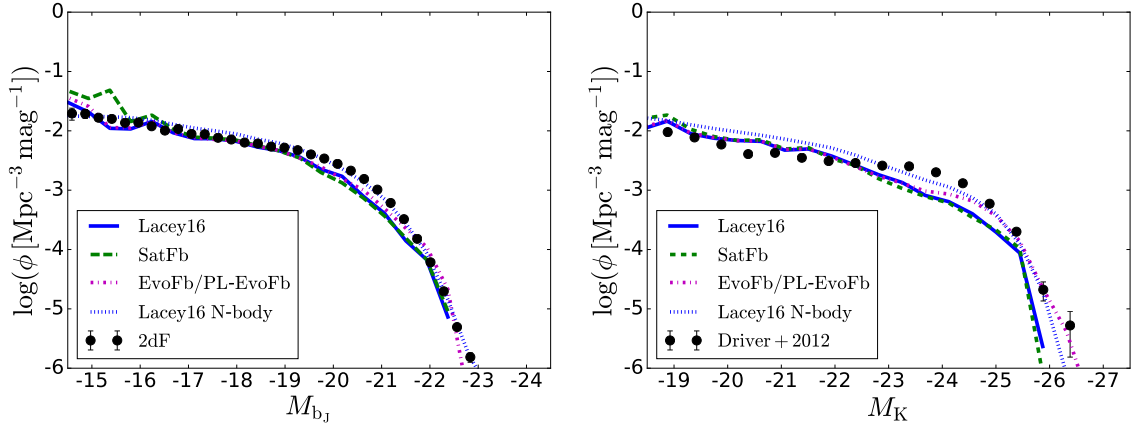
Figure 3.2: z = 0 field luminosity functions. The left panel shows the b_J -band luminosity function and the right panel the K -band luminosity function. In both panels the solid, dashed and dashed-dotted lines with different colours show the predictions using Monte Carlo merger trees for different SN feedback models, as indicated in the line key, while the blue dotted lines are for the Lacey16 model run with N-body merger trees. The magenta lines show the results of the EvoFb model, but the results for the PL-EvoFb model are almost identical. The black points with errorbars are observational data, from Norberg et al. (2002) for the b_J -band and from Driver et al. (2012) for the K -band.
