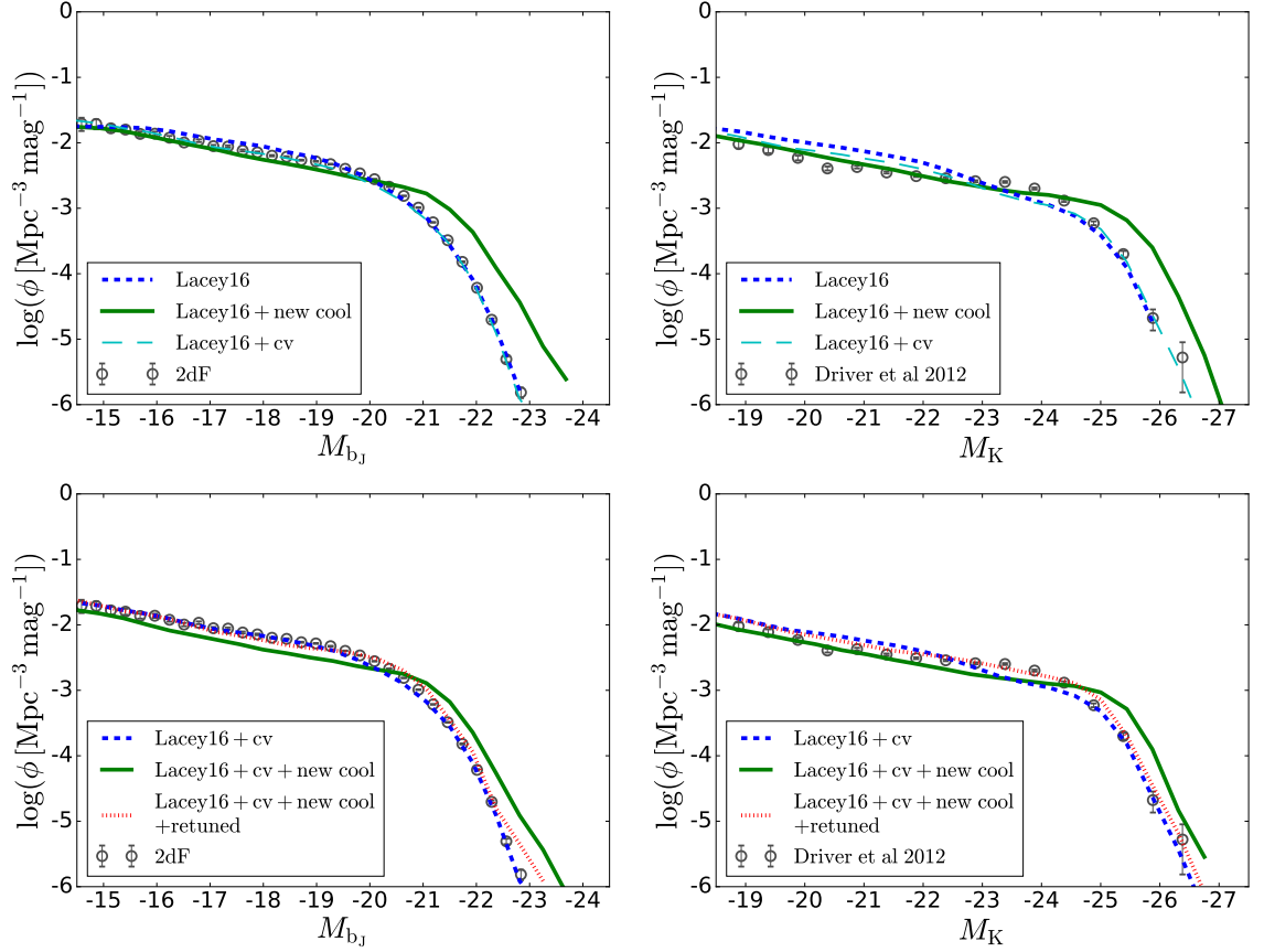
Figure 4.5: The field galaxy luminosity functions at z = 0 in the b_J and K bands for different variants of the Lacey16 model. Each line shows the prediction for a different model, with the corresponding model name given in the key. The different models are described in the text. The top panels show the original Lacey16 model and the separate effects of changing to the new cooling model or of updating the halo virial velocity at every timestep. In the bottom panels all models have the halo virial velocity updated at every timestep. The bottom panels include the retuned Lacey16 model incorporating the new treatment of gas cooling. The gray open circles with error bars are observational data, from Norberg et al. (2002) for the b_J -band and from Driver et al. (2012) for the K -band.
