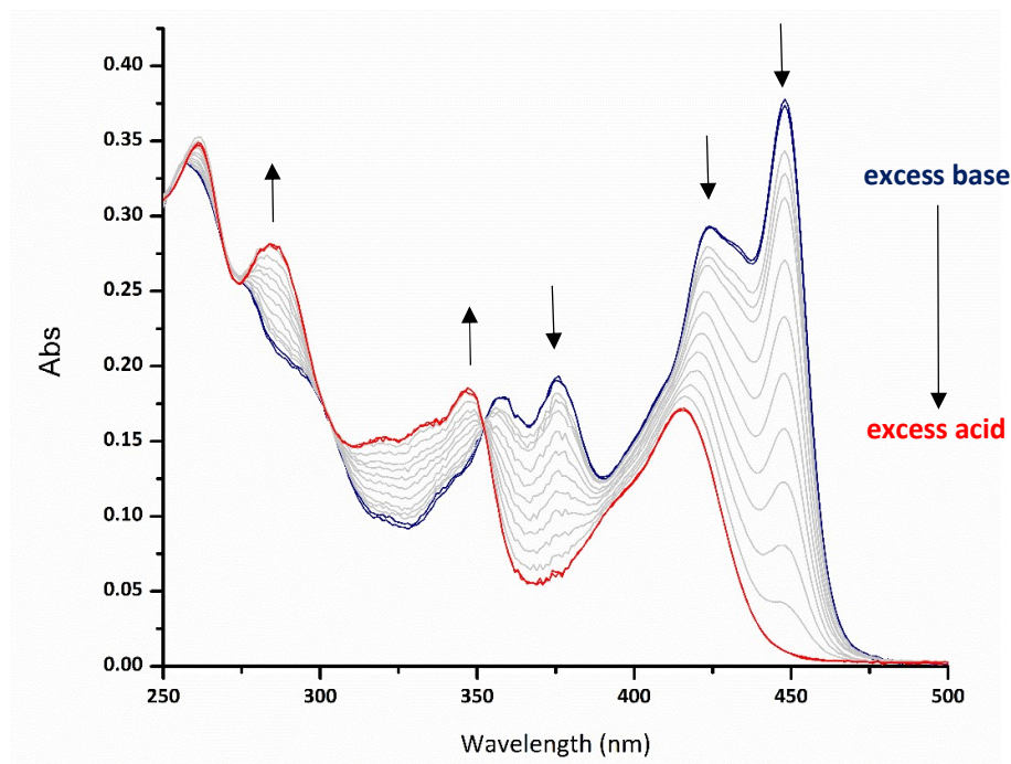
Figure 4.7: UV-Vis electronic absorption of \text{PtL}^6\text{Cl} at various concentrations of acid and base in MeCN
