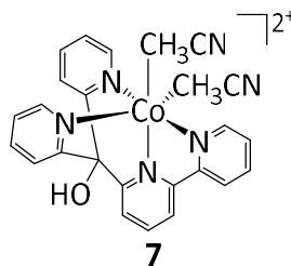
Figure 1.8: Tetradentate polypyridyl \text{Co}^{\text{II}} complex reported by Chang and co-workers.
