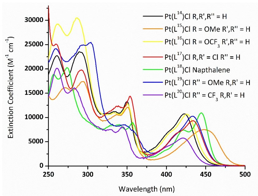
Figure 4.9: UV-Vis electronic absorption spectra of PtL 14-20 Cl.
