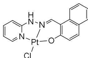
Figure 3.15: Pt(II) complexes of hydrazone (N-H) based N ^ N ^ O ligands.
