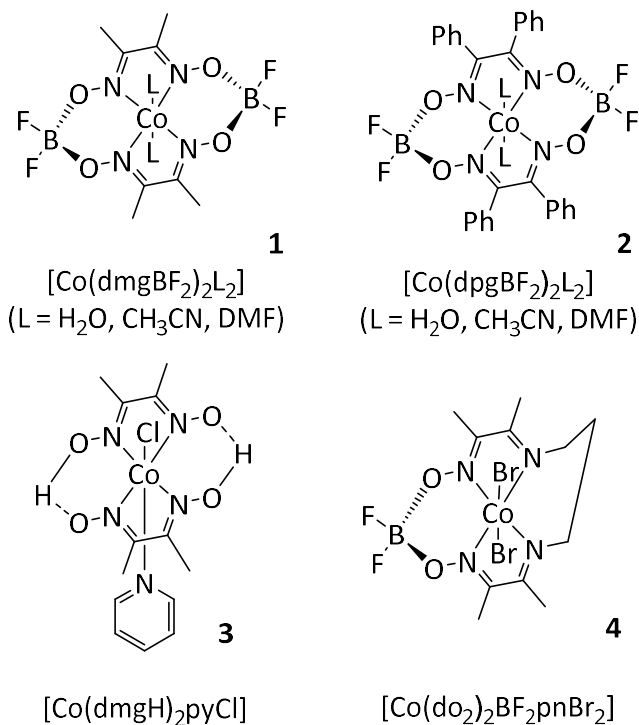
Figure 1.4: Structures of some cobaloximes. ( dmg = dimethylglyoxime, dpg = diphenylglyoxime, do = N 2 , N 2' -propanediylbis(2,3-butandione 2-imine 3-oxime).
