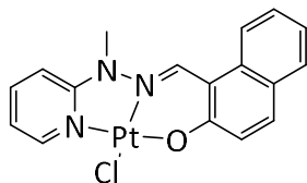
Figure 3.17: Pt(II) complexes of hydrazone (N-Me) based N N O ligands.
