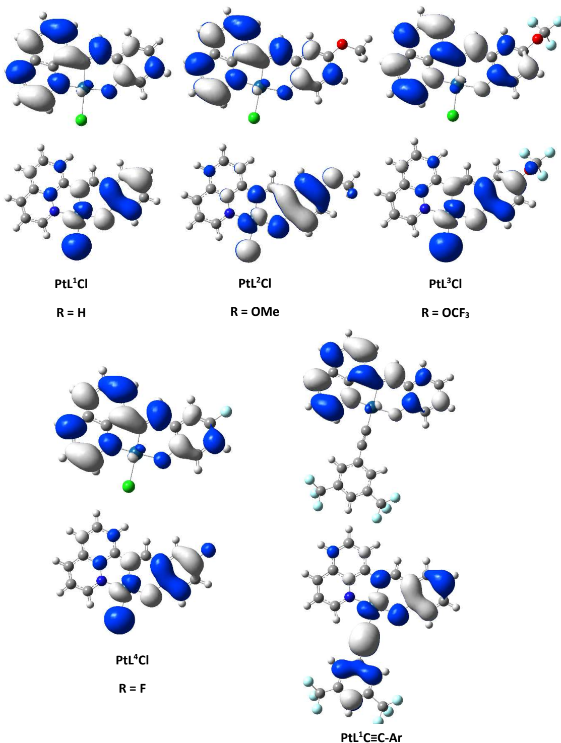
Figure 4.5: Calculated orbital density for the LUMO (top) and HOMO (bottom) of PtL^{1-4}Cl and PtL^1C\equiv C-Ar at their optimised S_0 geometries.
