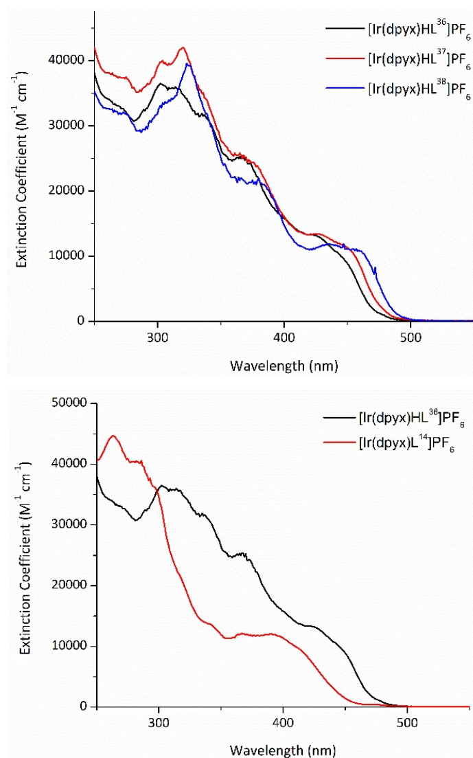
Figure 5.24: UV-Vis electronic absorption spectra of [\text{Ir}(\text{dppyx})\text{HL}^{36}]\text{PF}_6 – [\text{Ir}(\text{dppyx})\text{HL}^{38}]\text{PF}_6 in DCM at 298 K (top) and [\text{Ir}(\text{dppyx})\text{HL}^{36}]\text{PF}_6 and [\text{Ir}(\text{dppyx})\text{L}^{14}]\text{PF}_6 (bottom).
