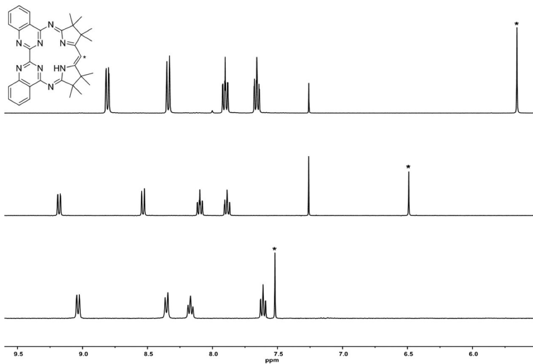
Figure 1.10: ^1\text{H} NMR spectra of HMabiq (top, \text{CDCl}_3 ), 1 (middle, \text{CDCl}_3 ), and 4 (bottom, \text{THF-d}_8 ), showing the aromatic protons and the diketiminate proton (*). 41
