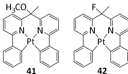
Figure 2.21: C A N * N A C Pt(II) complexes 41 and 42 .
