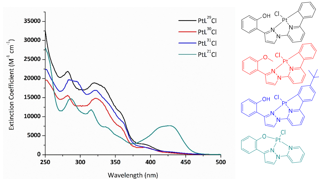
Figure 4.28: UV-Vis electronic absorption spectra of \text{PtL}^{29-31}\text{Cl} and \text{PtL}^{21}\text{Cl} in DCM at 298K.
