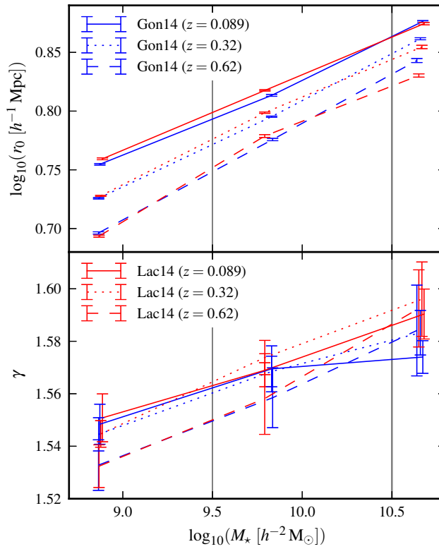
Figure 3.3 – Correlation lengths, r_0 (upper), and slopes, \gamma (lower), of the power law fitted to the \xi(r) shown in Fig. 3.2 for the Gon14 and Lac14 GALFORM models, as a function of stellar mass, M_{\star} , and redshift, z , (see equation 3.7). The vertical lines indicate the divisions between the mass bins used to measure \xi(r) . The M_{\star} values are the medians for each mass bin, model, and redshift. Each panel uses the same linestyles and colours; the legend is split between panels.
