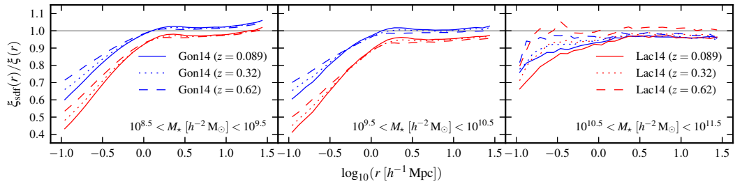
Figure 3.5 – Ratio of the real-space correlation function using the new subhalo dynamical friction merger scheme, \xi_{\text{sdf}}(r) , to that obtained with the default satellite merger prescription, \xi(r) , computed using the Gon14 and Lac14 GALFORM models, as a function of stellar mass, M_* , and redshift, z , (as labelled). The linestyles show different redshifts, and the colours indicate different models, as labelled. The legend is split across the panels.
