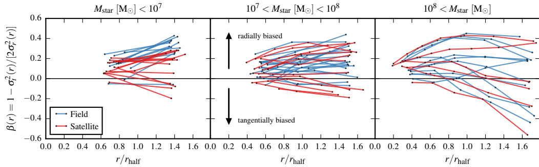
Figure 2.6 – Spherically averaged stellar velocity dispersion anisotropy profiles, \beta(r) , for dispersion-dominated ( \kappa_{\text{rot}} < 0.5 ) field and satellite galaxies in the HR simulations. \beta(r) is negative for tangentially biased dispersions, zero for isotropy, and positive for radially biased dispersions (see equation 2.3). The panels show different stellar mass ranges, as labelled. The profiles include all star particles between a radius of 2.8 times the softening (see Table 2.1) and twice the 3D stellar half-mass radius, r_{\text{half}} . The bin edges are evenly spaced percentiles of the radial distribution of the star particles, and the points show the median galactocentric radius of the star particles in each bin. The number of bins used for a given galaxy depends on how many star particles it has.
