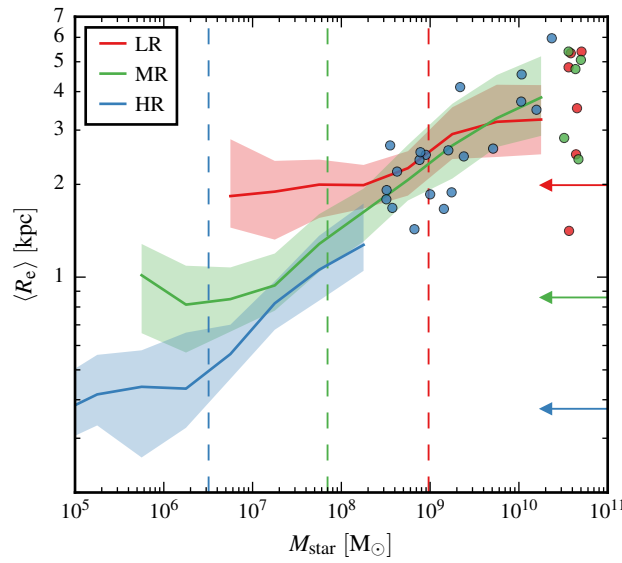
Figure 2.1 – Mean projected stellar half-mass radius, \langle R_e \rangle , versus stellar mass, M_{\text{star}} , for all galaxies that have at least ten star particles in the Δ POSTLE simulations at each resolution level (12 LR, 12 MR, and 2 HR simulations; different colours). The \langle R_e \rangle values are averaged over 1536 evenly distributed projections. For each resolution, the median is shown as a solid line, and the 16 th – 84 th percentiles are indicated by a shaded region of the same colour. Points are shown instead for bins with fewer than ten galaxies. The vertical dashed lines show the minimum M_{\text{star}} of the set of galaxies composed of at least 1000 star particles at each resolution. The horizontal arrows indicate 2.8 times the gravitational softening at each resolution (see Table 2.1).
