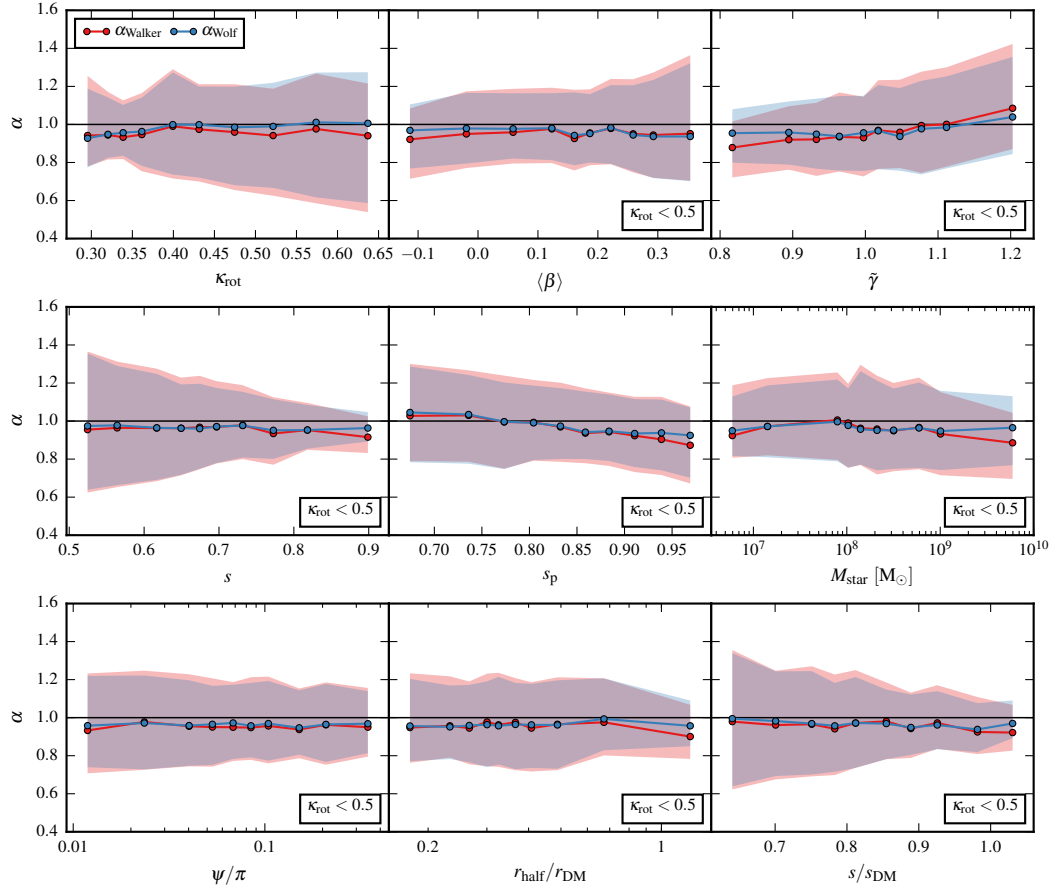
Figure 2.16 – Ratio, \alpha , of the estimated to true mass obtained using the estimators of Walker et al. (2009, \alpha_{\text{Walker}} ) and Wolf et al. (2010, \alpha_{\text{Wolf}} ), by projecting over 1536 evenly distributed lines of sight, as a function of various galaxy and subhalo dark matter properties. The properties shown are: the stellar kinematic measure used to discriminate between galaxies with different levels of rotational support ( \kappa_{\text{rot}} ), the mean stellar velocity dispersion anisotropy ( \langle\beta\rangle ), the stellar equilibrium measure ( \tilde{\gamma} ), the stellar sphericity ( s ), the projected stellar circularity ( s_p ), the stellar mass ( M_{\text{star}} ), the angle between the stellar and subhalo dark matter minor axes ( \psi ), the ratio of the stellar and dark matter scale radii ( r_{\text{half}}/r_{\text{DM}} ), and the ratio of the stellar and dark matter sphericities ( s/s_{\text{DM}} ). The first panel shows \alpha versus \kappa_{\text{rot}} for all galaxies; all other panels consider only those galaxies whose stellar motions are dominated by dispersion ( \kappa_{\text{rot}} < 0.5 ). For each estimator (colours), the solid lines show the median mass ratios and the shaded regions the 16 th – 84 th percentile spread. The bin edges are evenly spaced percentiles of the quantity on the horizontal axis, and the bin centres (points) are the median values in each bin.
