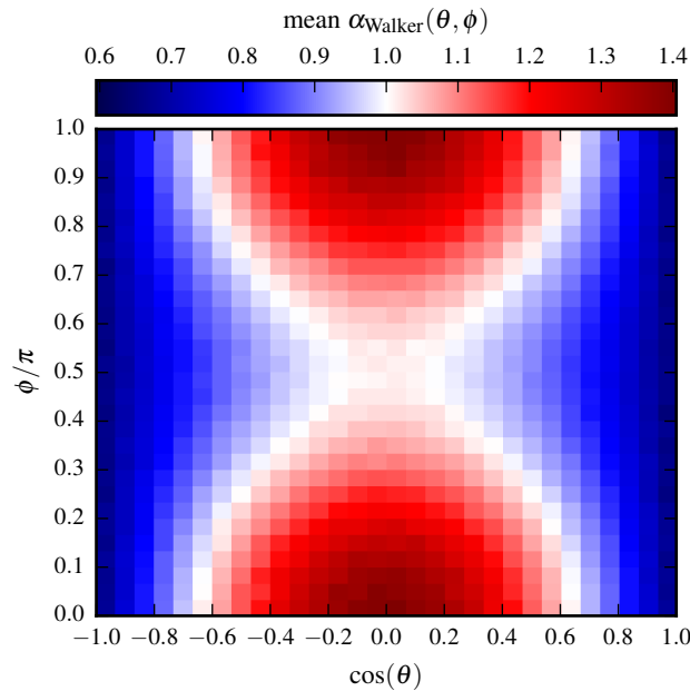
Figure 2.14 – Estimated to true mass ratio, \alpha_{\text{Walker}}(\theta, \phi) , resulting from applying the estimator of Walker et al. (2009) to all galaxies in our dispersion-dominated sample ( \kappa_{\text{rot}} < 0.5 ), by projecting over 1536 evenly distributed lines of sight for each galaxy. \theta and \phi are the spherical polar angles in the galactic coordinate system defined by the eigenbasis of the stellar reduced inertia tensor, where the z axis ( \theta = 0 ) is aligned with the shortest stellar principal axis, and the x axis ( \theta = \pi/2, \phi = 0 ) is aligned with the longest principal axis. The angular ranges are defined as 0 \leq \theta \leq \pi and 0 \leq \phi < 2\pi ; however, since projections in opposite directions are equivalent in the context of our analysis, we consider the coordinates of the set of 1536 unique lines of sight within the half-sphere defined by 0 \leq \theta < \pi and 0 \leq \phi < \pi in the grid shown here (extending the grid to \phi = 2\pi would result in repetition of the data). Since the lines of sight result from an evenly distributed spherical tessellation, plotting \phi versus \cos(\theta) = z/r ensures that the number of projections per grid pixel is approximately constant. The \alpha_{\text{Walker}}(\theta, \phi) value shown in each pixel is the mean over all projections of each galaxy within the relevant angular range. The colour scale is centred on a mass ratio of unity (i.e. white for accurate mean estimates, blue for mean underestimates, and red for mean overestimates). The results for the Wolf et al. (2010) estimator are very similar to those shown here. The distributions of the mass ratios, \alpha , for both estimators are shown in the upper panel of Fig. 2.9 (summing over all projections), and the \alpha variations relative to the galactic mean are shown in the upper panels of Fig. 2.13 (integrating over \theta and \phi separately).
