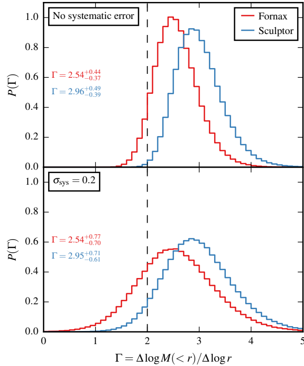
Figure 2.17 – Distributions, P(\Gamma) , of the logarithmic mass profile slope, \Gamma , derived using chemo-dynamically distinct stellar subpopulations in Sculptor and Fornax (see equation 2.15). The upper panel shows the distributions from sampling the posterior probability distribution functions for the half-light radii and velocity dispersions from Walker & Peñarrubia (2011). The lower panel shows the results of repeating this procedure, but introducing a 1\sigma scatter of \sigma_{\text{sys}} = 0.2 in the mass estimates for both populations. The median \Gamma value and 16 th – 84 th percentile confidence interval are given in each panel for each distribution, in the same colours as the lines. Each distribution is normalised such that \int_{-\infty}^{\infty} P(\Gamma) d\Gamma = 1 . The vertical dashed line shows the central (maximum) mass slope for an NFW profile.
