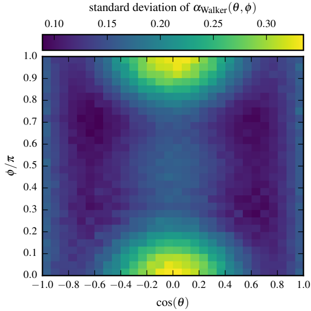
Figure 2.15 – The same as Fig. 2.14, but showing instead the standard deviation of the \alpha_{\text{Walker}}(\theta, \phi) values in each pixel, rather than the mean value. The details of the analysis are otherwise exactly as described in Fig. 2.14.
