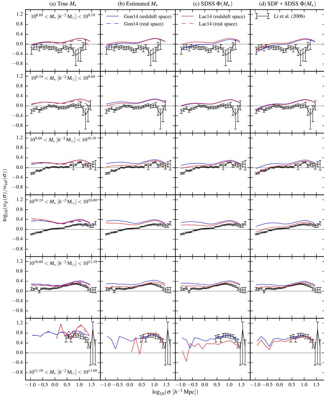
Figure 3.7 – Projected correlation function of galaxies, w_p(\sigma) , as a function of stellar mass, M_* (as labelled in each row), at redshift z = 0.089 , computed using the Gon14 and Lac14 GALFORM models, in real (first column only) and redshift space. The SDSS measurements of Li et al. (2006) are shown (black lines with errorbars). Each w_p(\sigma) has been divided by a reference power law, w_{\text{ref}}(\sigma) , with parameters r_0 = 5 h^{-1} \text{Mpc} and \gamma = 2 (horizontal line; see equation 3.9). Half the standard number of \sigma bins are shown for the highest mass interval, due to the small number of galaxies. Columns (a) and (b) show the default models with the true and estimated masses, respectively. The remaining columns show the results of matching the SDSS stellar mass function (as an adjustment following the SED fitting), for (c) the default models, and (d) the models using the new subhalo dynamical friction (SDF) merger scheme.
