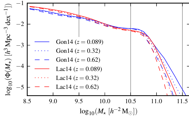
Figure 3.1 – Galactic stellar mass function, \Phi(M_\star) , predicted by the Gon14 and Lac14 GALFORM models, as a function of redshift. The vertical lines indicate the stellar mass samples used to measure \xi(r) in Fig. 3.2. The lower \Phi(M_\star) axis limit corresponds to 50 model galaxies per bin in the MS-W7 simulation volume.
