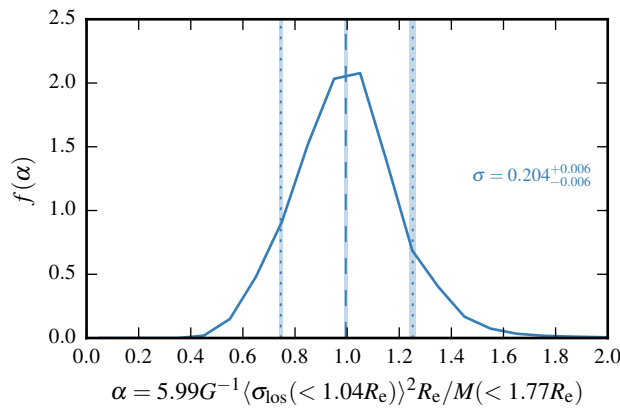
Figure 2.19 – Distribution, f(\alpha) , of the estimated to true mass ratio, \alpha , for the unbiased estimator with minimum scatter of the form given in equation (2.17). The optimum parameters are given in Table 2.3 (as in the horizontal axis label). The distribution considers all dispersion-dominated galaxies ( \kappa_{\text{rot}} < 0.5 ), using projections from 1536 evenly distributed lines of sight. The dashed line shows the median, and the dotted lines show the 10 th and 90 th percentiles. The standard deviation, \sigma , is also shown. The shaded regions around the vertical lines and the quoted errors on \sigma are the 16 th – 84 th percentile confidence limits, derived from applying the estimator to 10^4 bootstrap samples of the galaxies. Note that the similar \sigma errors given in Table 2.3 for this estimator are instead derived from the distribution of optimum \sigma values obtained from repeatedly calibrating equation (2.17) on bootstrap samples of the same galaxies. Each projection of each galaxy contributes to the distribution with equal weight, and the distribution is normalised to have unit area.
