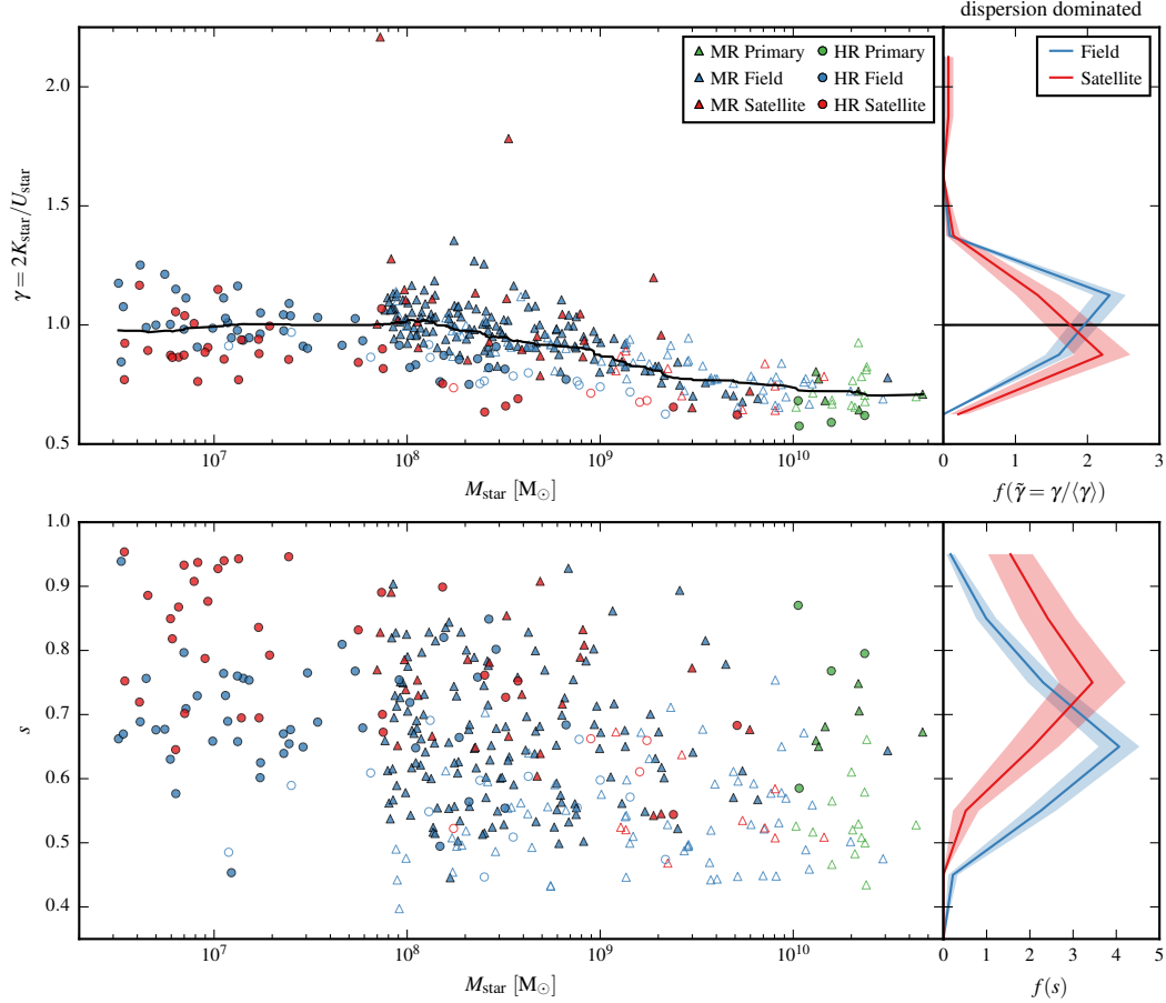
Figure 2.8 – Stellar energy ratio, \gamma (upper; see equation 2.11), and stellar sphericity, s (lower; derived from the reduced inertia tensor as defined in equation 2.12), versus stellar mass, M_{\text{star}} , for all galaxies in our simulated sample. The colours show whether a galaxy is one of the MW or M31 analogues (primary), within 300 kpc of either of these (satellite), or at larger distances (field). The symbol shapes indicate the resolution level (MR or HR). Dispersion-dominated galaxies ( \kappa_{\text{rot}} < 0.5 ) are plotted as filled symbols, while the symbols are unfilled for rotation-dominated galaxies ( \kappa_{\text{rot}} > 0.5 ). The black line in the upper panel shows the running median, \langle\gamma\rangle , of the \gamma values, considering at most 100 neighbouring galaxies in M_{\text{star}} for each galaxy. We define \tilde{\gamma} as the ratio of \gamma to this median line for each galaxy, and assume that galaxies with \tilde{\gamma} \approx 1 are in equilibrium. The panels on the right show the distributions of the rescaled energy ratio, f(\tilde{\gamma}) (not the distribution of \gamma itself), and the sphericity, f(s) , on the same vertical scales as the main panels, for only the dispersion-dominated field and satellite galaxies. Each distribution is normalised to have unit area. The shaded regions show the standard deviation assuming Poisson noise on each bin count.
