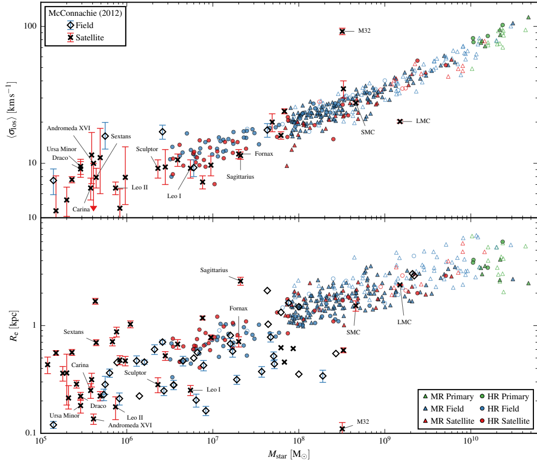
Figure 2.7 – Line-of-sight stellar velocity dispersion, \langle \sigma_{\text{los}} \rangle (upper), and projected stellar half-mass radius, R_e (lower), versus stellar mass, M_{\text{star}} , for all galaxies in our simulated sample. The \langle \sigma_{\text{los}} \rangle and R_e values have been computed for a single, randomly chosen, line of sight through the simulations. The galaxies are classified according to whether they are one of the MW or M31 analogues (primary), within 300 kpc of either of these (satellite), or at larger distances (field), as indicated in the lower right legend (different colours). The symbol shapes indicate the resolution level at which the galaxies have been simulated (MR or HR). Dispersion-dominated galaxies ( \kappa_{\text{rot}} < 0.5 ) are plotted as filled symbols, while rotation-dominated galaxies ( \kappa_{\text{rot}} > 0.5 ) are plotted as unfilled symbols of the same colour and shape. continued...
