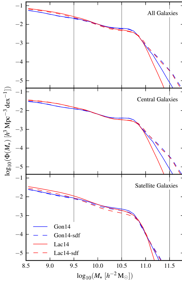
Figure 3.4 – Galactic stellar mass function, \Phi(M_\star) , at redshift z = 0.089 , for all (top), central (middle), and satellite (bottom) galaxies in the Gon14 and Lac14 GALFORM models, and for these models with the alternative subhalo dynamical friction merger scheme (labelled Gon14-sdf and Lac14-sdf). The vertical lines indicate the stellar mass samples used to compute \xi(r) in Fig. 3.5. The lower \Phi(M_\star) axis limit corresponds to 50 model galaxies per bin in the MS-W7 simulation volume. Note that the model parameters have not been recalibrated on adopting the new satellite merger scheme.
