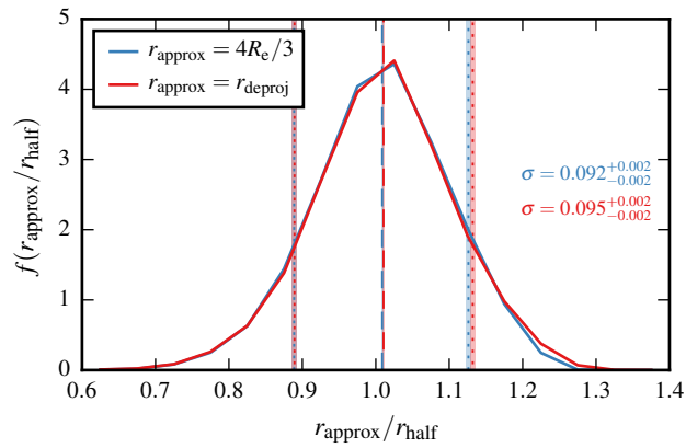
Figure B.1 – Distributions, f(r_{\text{approx}}/r_{\text{half}}) , of the ratio of approximations, r_{\text{approx}} , for the 3D half-mass radius, r_{\text{half}} , to the true value of the radius for galaxies in our dispersion-dominated sample ( \kappa_{\text{rot}} < 0.5 ). The r_{\text{approx}} values are computed for 1536 evenly distributed lines of sight, assuming either that r_{\text{half}} = 4R_e/3 , or using r_{\text{deproj}} from our Abel deprojection procedure (different colours). Each projection of each galaxy contributes to the distributions with equal weight, and each distribution is normalised to have unit area. The vertical dashed lines show the median ratios, and the dotted lines show the 10 th and 90 th percentiles. The standard deviation, \sigma , of each distribution is given in the same colour as the lines. The shaded regions around the vertical lines and the \sigma errors are the 16 th – 84 th percentile confidence limits, derived from 10^4 bootstrap samples of the galaxies for each distribution.
