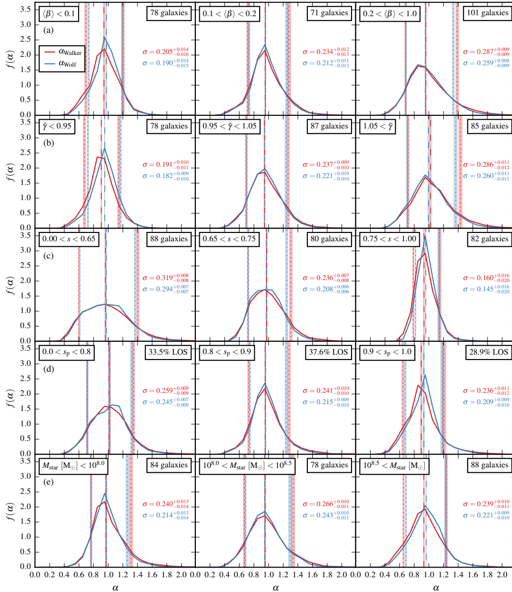
Figure 2.10 – Distribution, f(\alpha) , of the estimated to true mass ratio, \alpha , for dispersion-dominated galaxies ( \kappa_{\text{rot}} < 0.5 ), as a function of various galaxy properties. In each row, the dispersion-dominated sample is split into three bins (columns), according to: (a) the mean stellar velocity dispersion anisotropy, \langle\beta\rangle ; (b) the stellar equilibrium measure, \tilde{\gamma} ; (c) the stellar sphericity, s ; (d) the projected stellar circularity, s_p ; and (e) the stellar mass, M_{\text{star}} . Each panel is labelled with the interval it considers and the number of galaxies it contains (percentage of lines of sight in the case of circularity, where a single galaxy may contribute to more than one panel). The details of the computation of the distributions and the meaning of each line are as described in the caption of Fig. 2.9.
