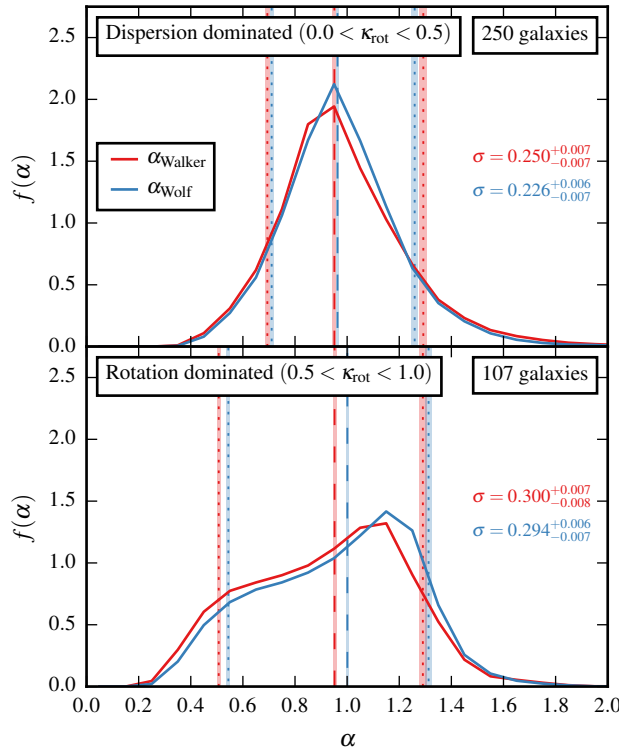
Figure 2.9 – Distributions, f(\alpha) , of the estimated to true mass ratio, \alpha , for all galaxies, obtained by projecting over 1536 evenly distributed lines of sight. The galaxies are split into a dispersion-dominated sample (upper panel), and a rotation-dominated sample (lower panel), according to the value of \kappa_{\text{rot}} (see equation 2.10). Different colours show the distributions obtained using the Walker et al. (2009, \alpha_{\text{Walker}} ) and Wolf et al. (2010, \alpha_{\text{Wolf}} ) estimators, as labelled. The dashed lines indicate the median \alpha values for each estimator and the dotted lines the 10 th and 90 th percentiles. The standard deviation, \sigma , of each distribution is given in the same colour as the lines. The shaded regions around the vertical lines and the quoted errors on \sigma are the 16 th – 84 th percentile confidence limits, derived from 10^4 bootstrap samples of the galaxies for each distribution. Each projection of each galaxy contributes to the relevant distribution with equal weight, and each distribution is normalised to have unit area. The panels are labelled with the number of galaxies they include. We highlight that the f(\alpha) axis limits used in Figs. 2.10, 2.11, 2.12, and 2.19 vary with respect to those used here, in order to optimise the clarity of each individual figure.
