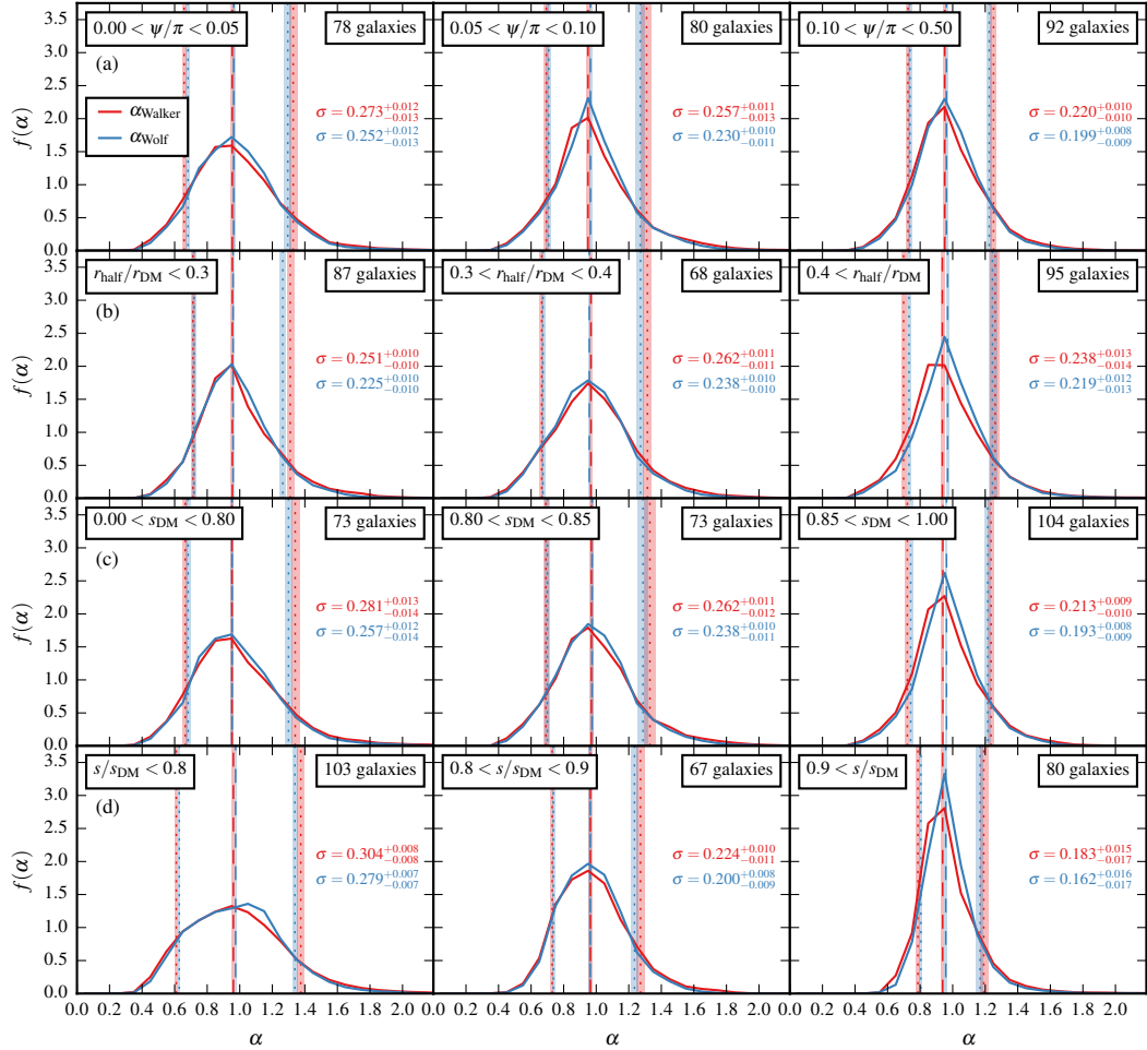
Figure 2.11 – Distribution, f(\alpha) , of the estimated to true mass ratio, \alpha , for dispersion-dominated galaxies ( \kappa_{\text{rot}} < 0.5 ), as a function of various galaxy and host subhalo dark matter properties. In each row, the dispersion-dominated galaxy sample is split into three bins (columns), according to: (a) the angle between the minor axis of the galaxy and that of the dark matter mass distribution within its host subhalo, \psi ; (b) the ratio of the stellar 3D half-mass radius, r_{\text{half}} , to the subhalo dark matter scale radius, r_{\text{DM}} ; (c) the subhalo dark matter sphericity, s_{\text{DM}} ; and (d) the ratio s/s_{\text{DM}} , where s is the stellar sphericity. Each panel is labelled with the interval it considers and the number of galaxies it contains. The details of the computation of the distributions and the meaning of each line are as described in the caption of Fig. 2.9.
