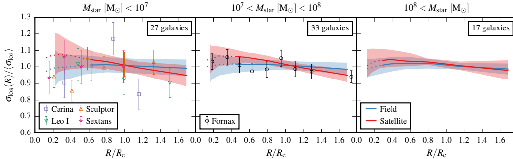
Figure 2.5 – Line-of-sight stellar velocity dispersion profiles, \sigma_{\text{los}}(R) , for dispersion-dominated ( \kappa_{\text{rot}} < 0.5 ) field and satellite galaxies in the HR simulations, where each panel shows a different stellar mass range (labelled with the number of galaxies). The solid lines are the median profiles obtained from 1536 evenly distributed projections for all galaxies of a given type (different colours; legend in right panel), around which the shaded regions of the same colour indicate the 16 th –84 th percentile spread. Each individual profile is scaled, prior to stacking, by the projected stellar half-mass radius, R_e , and the mean stellar velocity dispersion of the whole galaxy, \langle \sigma_{\text{los}} \rangle , for that line of sight. The shaded regions are not shown below the gravitational softening (see Table 2.1; in units of the median R_e in each panel), and the median profiles are dotted below 2.8 times the softening. The symbols with error bars show data for dSph satellites of the MW, where the data for each dSph are plotted in the relevant panel for its stellar mass following McConnachie (2012). The profiles shown are for Carina, Fornax, Leo I, Sculptor, and Sextans, as computed by Strigari et al. (2010). The measurements are scaled in the same way as the simulation predictions, using the half-light radii from McConnachie (2012).
