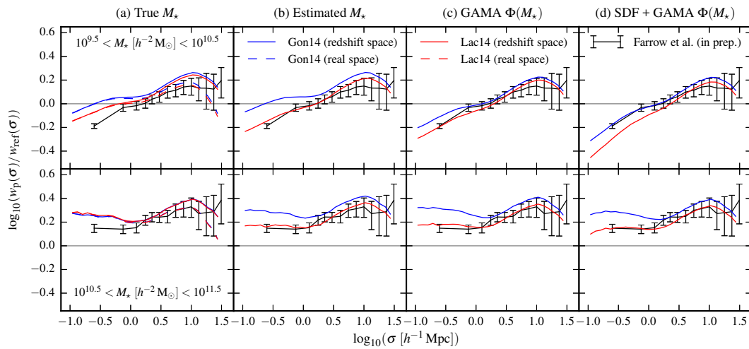
Figure 3.8 – Projected correlation function of galaxies, w_p(\sigma) , for different stellar mass, M_* , bins (as labelled in each row) at redshift z = 0.17 , computed using the Gon14 and Lac14 GALFORM models, in real (first column only) and redshift space. The GAMA measurements of Farrow et al. (2015) are shown, whose apparent magnitude limit has been imposed on the model galaxies (black lines with errorbars; labelled in prep. since the final data published by Farrow et al. 2015 use slightly different mass intervals etc. to those used here; see §3.3.3). For clarity, each w_p(\sigma) has been divided by a reference power law, w_{\text{ref}}(\sigma) , with parameters r_0 = 5 h^{-1} Mpc and \gamma = 2 (horizontal line; see equation 3.9). Columns (a) and (b) show the default models with the true and estimated masses, respectively. The remaining columns show the results of matching the GAMA stellar mass function (as an adjustment following the SED fitting), for (c) the default models, and (d) the models using the new subhalo dynamical friction (SDF) merger scheme.
