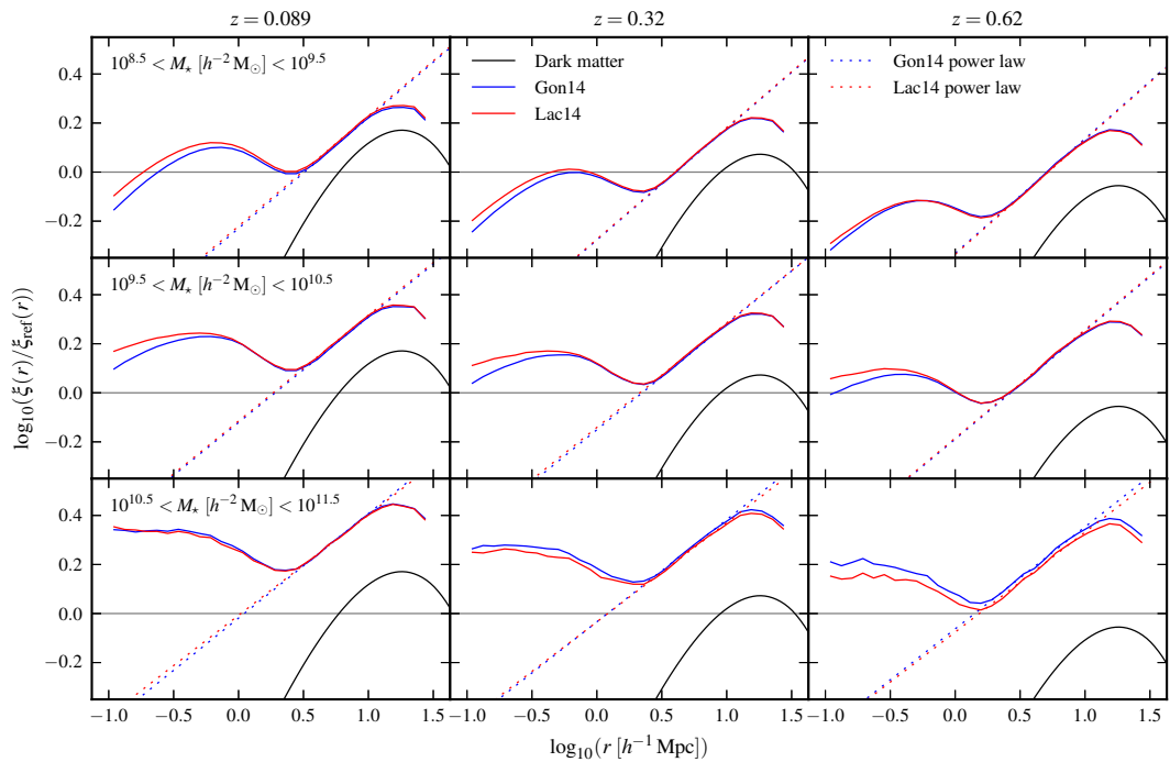
Figure 3.2 – Correlation function of galaxies, \xi(r) , as a function of redshift, z (columns), and stellar mass, M_\star (rows), as predicted using the Gon14 and Lac14 GALFORM models. For clarity, each \xi(r) has been divided by a reference power law, \xi_{\text{ref}}(r) , with parameters r_0 = 5 h^{-1} \text{Mpc} and \gamma = 2 (horizontal line; see equation 3.7). The dotted lines are power law fits to each GALFORM \xi(r) , for 3 < r [h^{-1} \text{Mpc}] < 10 , with the parameters shown in Fig. 3.3. The black curves show \xi(r) for the dark matter at each redshift, computed as the Fourier transform of the MS-W7 linear theory power spectrum (see equation 1.15).
