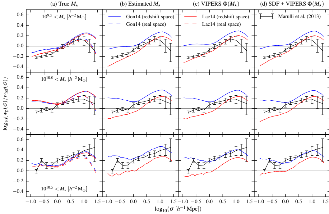
Figure 3.9 – Projected correlation function of galaxies, w_p(\sigma) , as a function of cumulative stellar mass, M_* (as labelled in each row), at redshift z = 0.62 , computed using the Gon14 and Lac14 GALFORM models, in real (first column only) and redshift space. The VIPERS measurements of Marulli et al. (2013) are shown (black lines with errorbars), whose apparent magnitude limit has been imposed on the model galaxies. For clarity, each w_p(\sigma) has been divided by a reference power law, w_{\text{ref}}(\sigma) , with parameters r_0 = 5 h^{-1} Mpc and \gamma = 2 (horizontal line; see equation 3.9). Columns (a) and (b) show the default models with the true and estimated masses, respectively. The remaining columns show the results of matching the VIPERS stellar mass function (as an adjustment following the SED fitting), for (c) the default models, and (d) the models using the new subhalo dynamical friction (SDF) merger scheme.
