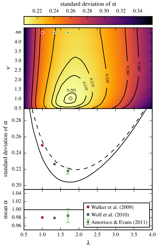
Figure 2.18 – Calibration of mass estimator parameters ( \lambda , \mu , \nu ) using all dispersion-dominated galaxies in our simulated sample (see equation 2.17). The upper panel shows the standard deviation of the estimated to true mass ratio \alpha as a function of \lambda and \nu , where the proportionality constant \mu is chosen such that the estimator is unbiased (mean \alpha equals one) for each combination of \lambda and \nu . The scatter shown is linearly interpolated between \nu = 4 and the case where the dispersion is averaged over the whole galaxy ( \nu \rightarrow \infty ). The lines show contours of constant standard deviation, as labelled. The diamond symbol indicates the location of minimum scatter (see Table 2.3). The middle panel shows the scatter as a function of \lambda , for the choice of \nu which minimises the scatter at each value of \lambda (solid line), and using instead the velocity dispersion averaged over the whole galaxy (dashed line). The points show the corresponding results from applying the estimators of Walker et al. (2009), Wolf et al. (2010), and Amorisco & Evans (2011), which each use the dispersion averaged over the whole galaxy. Note that the \alpha distribution for a given estimator can have a lower scatter than the dashed line, provided that it is biased in the mean. The lower panel shows the mean \alpha for each of these three estimators.
