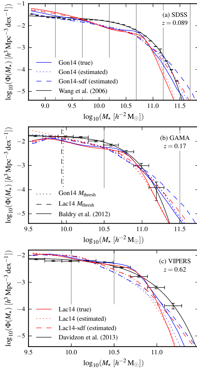
Figure 3.6 – Galactic stellar mass function, \Phi(M_\star) , as predicted using the Gon14 and Lac14 GALFORM models, at redshifts (a) 0.089, (b) 0.17, and (c) 0.62. Solid and dotted lines show the true and estimated \Phi(M_\star) respectively for the default models. Dashed lines show the estimated \Phi(M_\star) for the models using the new merger scheme (Gon14-sdf and Lac14-sdf). The formats of the model lines are the same in each plot, and are labelled in (a) and (c). The points with error bars are the measurements of (a) Wang et al. (2006) using SDSS, (b) Baldry et al. (2012) using GAMA, and (c) Davidzon et al. (2013) using VIPERS; shown alongside Schechter (1976) function fits (black lines; see Table 3.1). continued...
