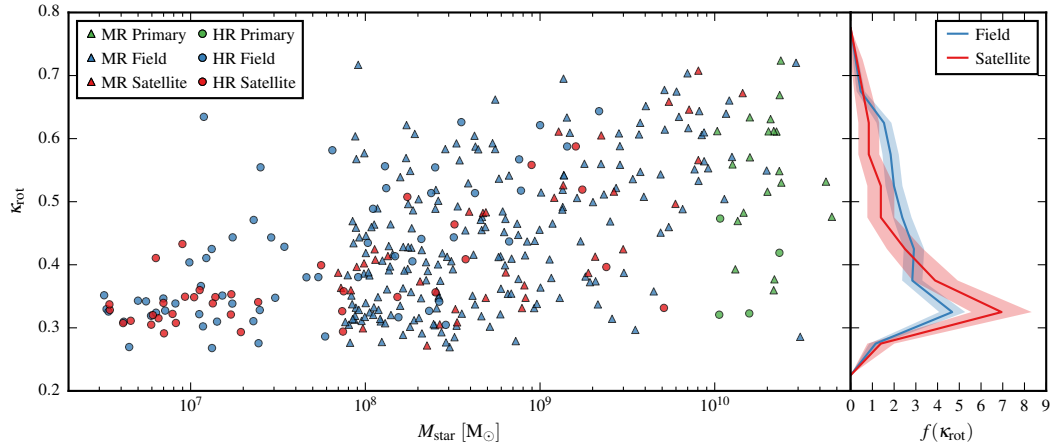
Figure 2.2 – Kinematic measure, \kappa_{\text{rot}} , used to discriminate amongst galaxies with different levels of stellar rotational support (see equation 2.10), shown versus stellar mass, M_{\text{star}} , for all galaxies in our simulated sample. The galaxies are classified according to whether they are one of the MW or M31 analogues (primary), within 300 kpc of either of these (satellite), or located at larger distances (field). The symbol shapes indicate the resolution level at which each galaxy has been simulated (MR or HR). Our dispersion-dominated galaxy sample consists of all galaxies that have \kappa_{\text{rot}} < 0.5 . The panel on the right shows the distributions, f(\kappa_{\text{rot}}) , of \kappa_{\text{rot}} for all field and satellite galaxies. Each distribution is normalised to have unit area. The shaded regions show the standard deviation assuming Poisson noise on each bin count.
