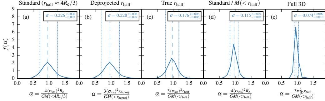
Figure B.2 – Distributions, f(\alpha) , of the estimated to true mass ratio, \alpha , for all dispersion-dominated galaxies ( \kappa_{\text{rot}} < 0.5 ), obtained from projecting over 1536 evenly distributed lines of sight, using different versions of the estimator proposed by Wolf et al. (2010). The definition of \alpha is different in each panel, and is given explicitly in each horizontal axis label. The definitions are: (a) the ratio of the estimated mass using equation (2.9) to the mass enclosed within the assumed 3D half-mass radius ( 4R_e/3 ) – this is the standard definition of \alpha_{\text{Wolf}} as given in equation (2.14), (b) the estimated to true mass ratio from equation (2.8) using the deprojected 3D half-mass radius, r_{\text{deproj}} , from our Abel integration procedure in place of r_{\text{half}} , (c) the same as (b) but using the true 3D half-mass radius, r_{\text{half}} , (d) the ratio of the estimated mass from equation (2.9) to the mass within r_{\text{half}} (i.e. this is the ratio of the estimated to true mass within different spheres , unless r_{\text{half}} = 4R_e/3 ), and (e) the estimated to true mass ratio if we replace \langle \sigma_{\text{los}} \rangle in equation (2.8) with the mean one-dimensional stellar velocity dispersion, \sigma_{1D} = \sigma_{3D}/\sqrt{3} (so no projected information is used in this panel). Each projection (if applicable) of each galaxy contributes to the distributions with equal weight, and each distribution is normalised to have unit area. The vertical dashed lines show the median \alpha values, and the dotted lines show the 10 th and 90 th percentiles. The standard deviation, \sigma , of each distribution is given in each panel. The shaded regions around the vertical lines and the \sigma errors are the 16 th – 84 th percentile confidence limits, derived from 10^4 bootstrap samples of the galaxies for each distribution.
