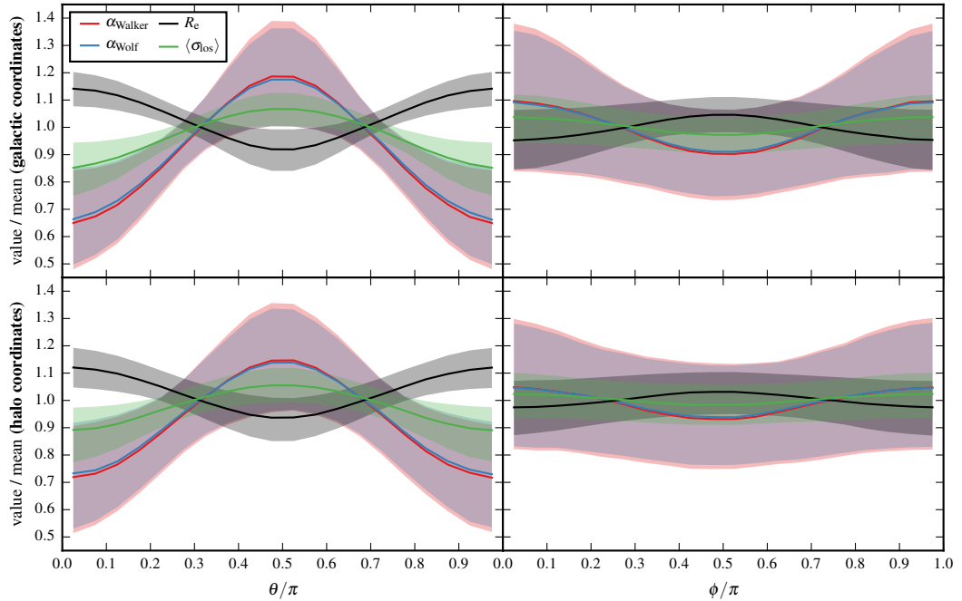
Figure 2.13 – Angular variation of the estimated to true mass ratio for the Walker et al. (2009, \alpha_{\text{Walker}} ) and Wolf et al. (2010, \alpha_{\text{Wolf}} ) estimators, the projected stellar half-mass radius, R_e , and the line-of-sight stellar velocity dispersion, \langle\sigma_{\text{los}}\rangle , for dispersion-dominated galaxies ( \kappa_{\text{rot}} < 0.5 ), computed by projecting over 1536 evenly distributed lines of sight. The curves are shown as functions of the spherical polar angles, \theta and \phi , where the coordinate system is aligned with the eigenbasis of the reduced inertia tensor of either the galactic star particles (upper panels) or the dark matter particles of the host subhalo (lower panels). The z axis ( \theta = 0 ) is aligned with the shortest principal axis, and the x axis ( \theta = \pi/2, \phi = 0 ) is aligned with the longest principal axis. The spherical polar angular ranges are defined as 0 \leq \theta \leq \pi and 0 \leq \phi < 2\pi . Since projections in opposite directions are equivalent in this work, the 1536 unique lines of sight are identified by their angular coordinates in the half-sphere defined by 0 \leq \theta < \pi and 0 \leq \phi < \pi within this figure. For each galaxy, the values of \alpha_{\text{Walker}} , \alpha_{\text{Wolf}} , R_e , and \langle\sigma_{\text{los}}\rangle for each projection have been divided by the corresponding mean value over all projections of that galaxy, before computing the curves shown. The solid lines show the median values, and the shaded regions of the same colour indicate the 16 th – 84 th percentile spread (the \theta and \phi axes use the same fixed bin width, in units of \pi ). Each panel makes use of the full set of 1536 lines of sight, so at fixed \theta (left) or \phi (right), the median and percentile range values shown result from the data for all lines of sight (with that particular \theta or \phi ) for all galaxies.
