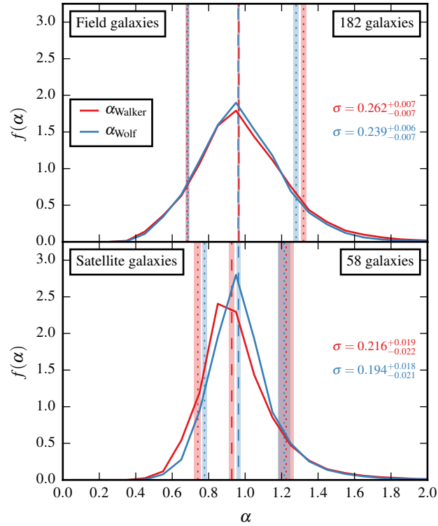
Figure 2.12 – Distributions, f(\alpha) , of the estimated to true mass ratio, \alpha , for field (upper panel) and satellite (within 300 kpc of MW or M31; lower panel) galaxies in the dispersion-dominated sample ( \kappa_{\text{rot}} < 0.5 ). The details of the computation of the distributions and the meaning of each line are as described in the caption of Fig. 2.9.
