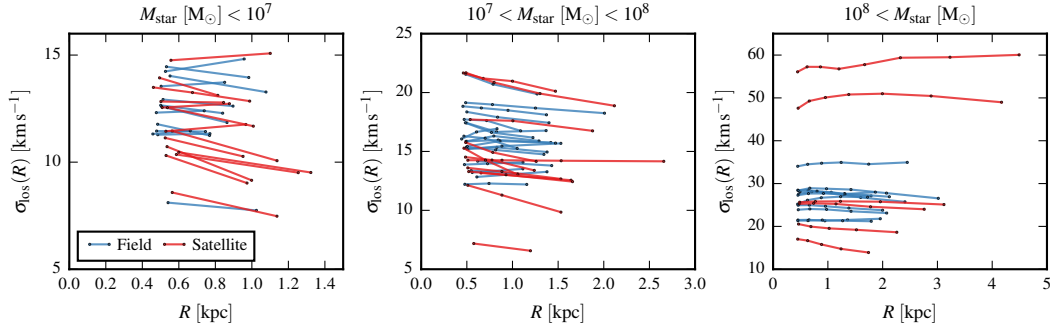
Figure 2.4 – Line-of-sight stellar velocity dispersion profiles, \sigma_{\text{los}}(R) , for dispersion-dominated ( \kappa_{\text{rot}} < 0.5 ) field and satellite galaxies in the HR simulations, where each panel shows a different stellar mass range. The line shown for each galaxy is the median profile obtained from projecting over 1536 evenly distributed lines of sight, considering star particles at projected radii between 2.8 times the gravitational softening (see Table 2.1) and twice the mean projected stellar half-mass radius of the galaxy. The bin edges are evenly spaced in the logarithm of R , and the points shown are the linear means of the bin edges. The number of bins used for each galaxy is a function of its star particle count. Note that the axis limits differ between panels.
