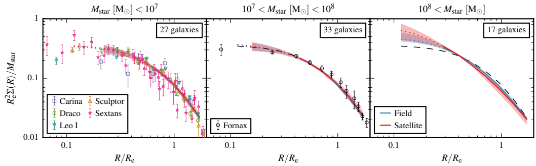
Figure 2.3 – Projected stellar density profiles, \Sigma(R) , for dispersion-dominated ( \kappa_{\text{rot}} < 0.5 ) field and satellite galaxies in the HR simulations. The solid lines are the median projected profiles obtained from 1536 evenly distributed projections for all galaxies of a given type (different colours; legend in right panel), around which the shaded regions of the same colour indicate the 16 th – 84 th percentile spread. Each individual profile is scaled, prior to stacking, by the projected stellar half-mass radius, R_e , for that line of sight, and the stellar mass, M_{\text{star}} . The shaded regions are not shown below the gravitational softening (see Table 2.1; in units of the median R_e in each panel), and the median profiles are dotted below 2.8 times the softening. The panels show different stellar mass ranges, and are labelled with the number of simulated galaxies they contain. As a visual aid, the median profile for all galaxies in the lowest mass bin is repeated as a dashed black line in the higher mass bins. The symbols with error bars show data for dSph satellites of the MW, where the data for each dSph are plotted in the relevant panel for its stellar mass following McConnachie (2012). The data shown are for Carina (Muñoz et al., 2006), Draco (Odenkirchen et al., 2001), Fornax (Coleman et al., 2005), Leo I (Smolčić et al., 2007), Sculptor (Battaglia et al., 2008), and Sextans (Irwin & Hatzidimitriou, 1995). The measurements are scaled in the same way as the simulation predictions, assuming either a Gaussian (Leo I) or Plummer (all others) density profile fit.
