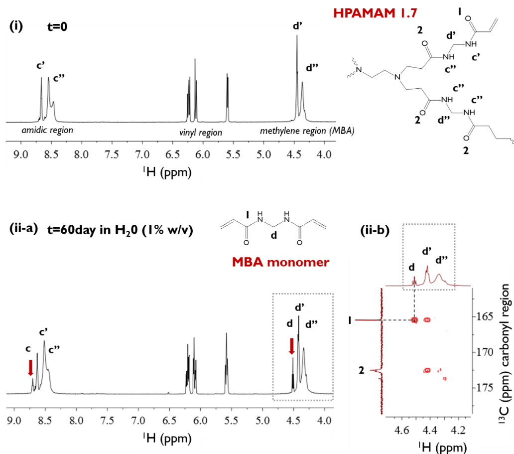
Figure 4.21 ^1\text{H} -NMR (700MHz, d-DMSO) of : (i) the polymer HPAMAM 1.7; (ii-a) the same sample after 2 months (60 days) in water at 1% w/v in which the presence of MBA is also detected. (ii-b) ^1\text{H} , ^{13}\text{C} -HMBC enlargement.
