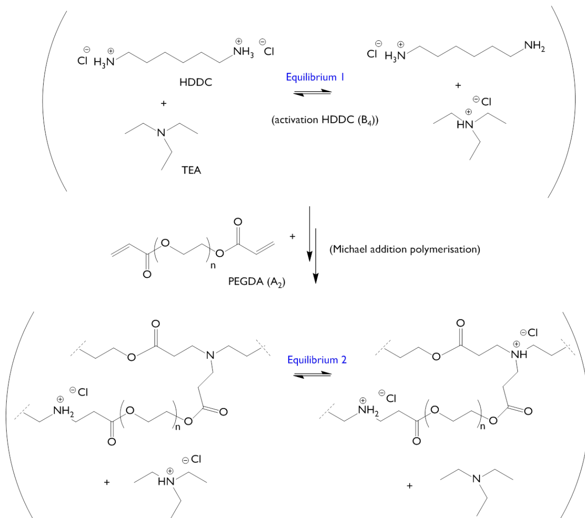
Scheme 3.10 Equilibrium reactions likely involved in the polymerisation \text{A}_2 + \text{B}_4 \cdot 2\text{HCl} .
