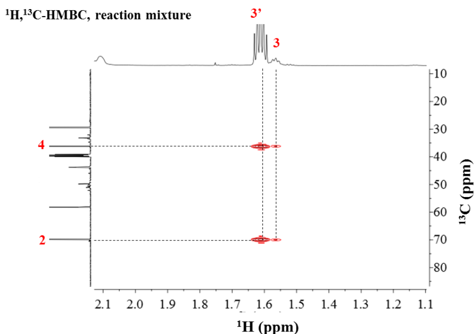
Figure 5.5 Enlargement of the ^1\text{H},^{13}\text{C} -HMBC spectrum of the product analysed without purification before the precipitation of the mixture of the polyaddition 2.5MBA+1.3MPAM+1EDA (HPAMAM 1.A5).
