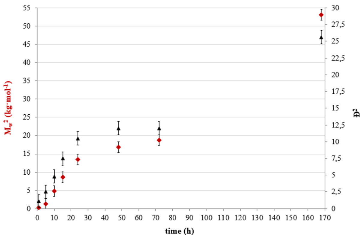
Figure 4.15 Increase of the M_w^2 and \bar{D}^2 (obtained by DMF-SEC analysis - PEO as stds - excluding the unreacted monomer from the distribution of the chromatograms) with the time of the reaction 3MBA-1EDA at 40°C in methanol/water (18% w/v).
