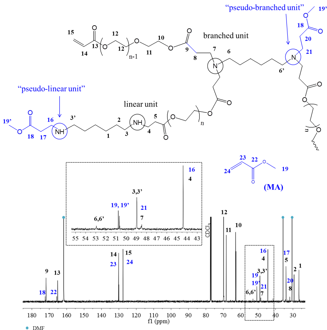
Figure 3.14 ^{13}\text{C} -NMR (176MHz, \text{CDCl}_3 ) and structure of the product of the reaction 1.5PEGDA+1MA+1HDA (in DMF 25% w/v, T=60°C). The spectrum was recorder after 3 hours and it is relative to the product analysed without purification.
