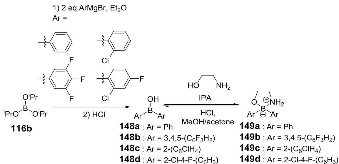
Scheme 29 Synthesis of ethanolamine complexes 149 and their reverse hydrolysis to borinic acids 148
