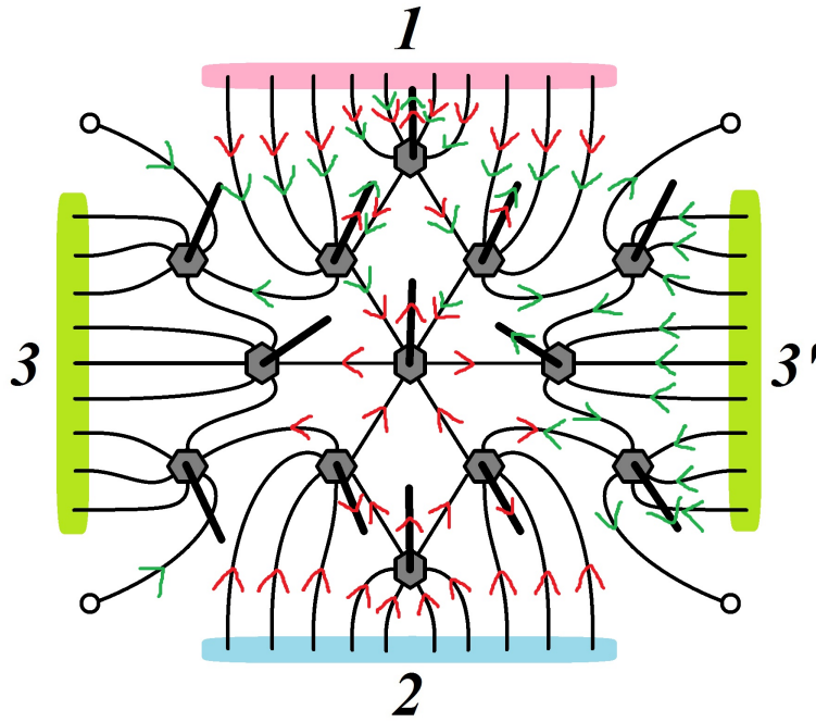
Figure 48: A holographic septagon code for three-boundary wormhole in the wheel regime. Dangling bulk legs are indicated by thicker lines. The red and green arrow assignments depict our attempts to reconstruct the operator bulk site at the centre. The red arrow assignment corresponds to choosing the 1 and 2 for which we can reconstruct the central site. The green arrow assignment attempts to reconstruct the central site from just boundary 1 and 3' (half of boundary 3) and fails. The code thus behaves like a quantum secret sharing scheme, for which access to information, here pertaining to local bulk information, is only accessible with a sufficiently large share in hand; in this case being a sufficiently large portion of the boundary.
