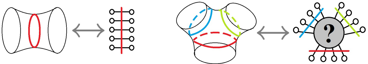
Figure 12: (Left) The entanglement between the two boundaries in BTZ can be distilled to bell pairs crossing the horizon, meaning that the entanglement is entirely bipartite. (Right) for a triply-connected, three-boundary wormhole with three horizons (red, green and blue), we might anticipate that the entanglement structure is in some sense intrinsically tripartite.
