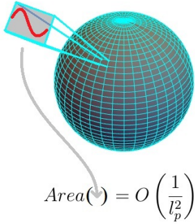
Figure 2: In quantum gravity, the black hole entropy can be thought to derive from microscopic degrees of freedom associated to Planck-scale regions of the black hole horizon, since the Bekenstein-Entropy measures the horizon area according to (1.1).
