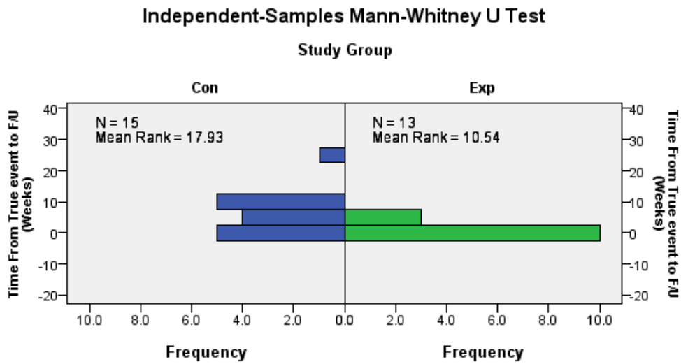
Figure 18 - Mann-Whitney U test comparison illustration and test statistics used in the calculation
