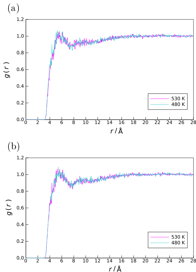
Figure 6.19: The radial distribution function for (a) phenyl-2 pairs and (b) phenyl-3 pairs of the C4O-Ph-ODBP mesogen.
