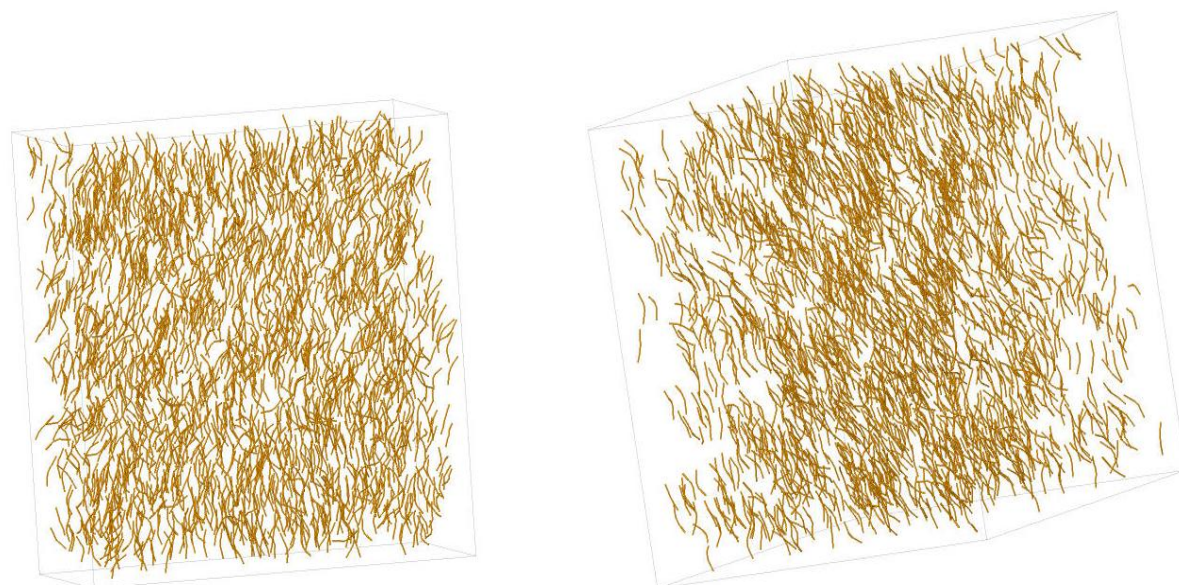
Figure 5.29: Snapshots of the C5-Ph-ODBP-Ph-OC12 system showing simplified ODBP cores only at 450 K for N = 2048 molecules: (a) Test 1 and (b) Test 2.
