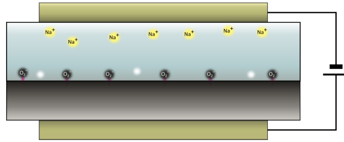
Figure 7.2: Schematic of the anodic bonding process. Substrates to be bonded are placed between 2 electrodes. Vacancies are formed at the bond interface by the diffusion of sodium atoms towards the cathode. Silicon atoms can then move into these vacancies forming silicon-oxide bonds.
