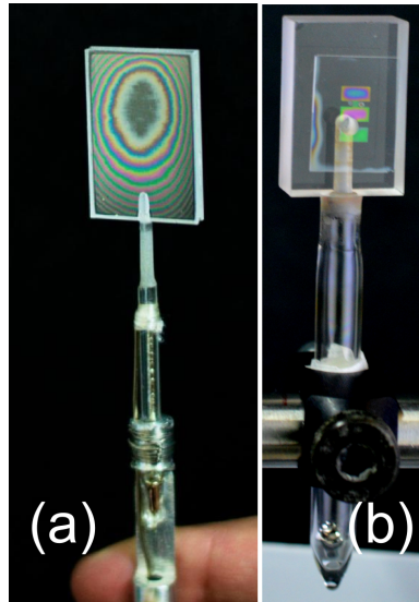
Figure 1.3: (a) Sapphire nanocell containing Cs produced in Armenia. Length ranges from 30-2000 nm. Photo courtesy of James Keaveney. (b) Three chambered quartz Rb nanocell produced in Durham, with chambers of length 1.5, 0.75 and 0.5 \mu\text{m} .
