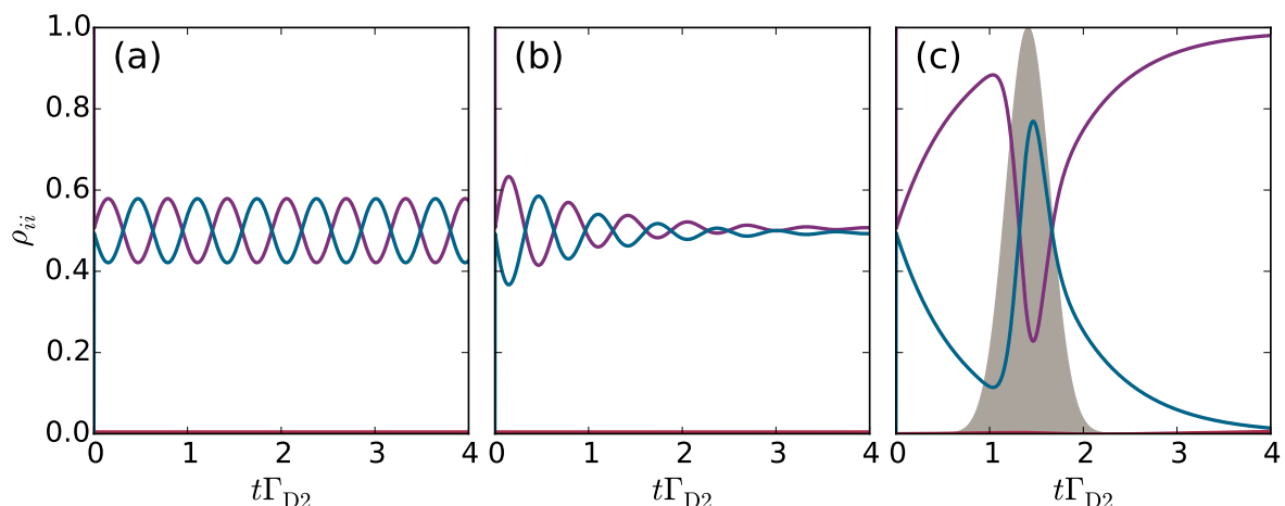
Figure 6.2: Optical Bloch simulation results for the 3 level vee system shown in Fig. 6.1, for starting parameters \rho_{gg,ee} = 0.5 , \Omega_e/2\pi = 127 MHz and \Omega_p/2\pi = 5 MHz. The ground state population \rho_{gg} is plotted as a set of blue lines, the excited state \rho_{ee} is plotted in purple. The probe state population \rho_{pp} is plotted in red. Panel (a) shows the system response for CW excitation with no decay mechanisms present. Panel (b) shows the system response for a vapour with both spontaneous decay and decay due to inter-atomic collision events. Panel (c) shows the time evolution for a pulsed excitation beam of FWHM 10 ns. The exciting pulse is plotted as a grey area for reference. The time axis is scaled to the natural line-width of the excited state transition \Gamma_{D2} .
