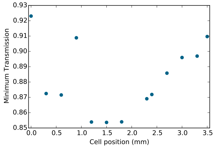
Figure 7.15: Change in minimum transmission as the probe beam ( \lambda=780 nm) is moved laterally across the cell science chamber. Minimum transmission decreases towards the centre of the cell, indicating that it is increasing in length.
