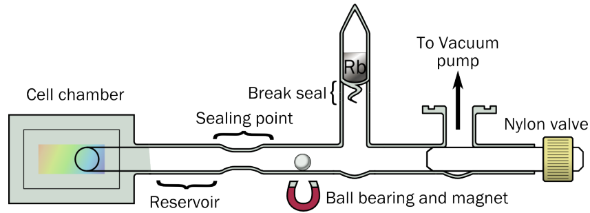
Figure 7.5: Loading manifold for sealing with pure Rb. Rb is sealed in a chamber that can be broken using a ball bearing that is placed inside the manifold. The rubidium is then distilled into the cell reservoir using a heat gradient.
