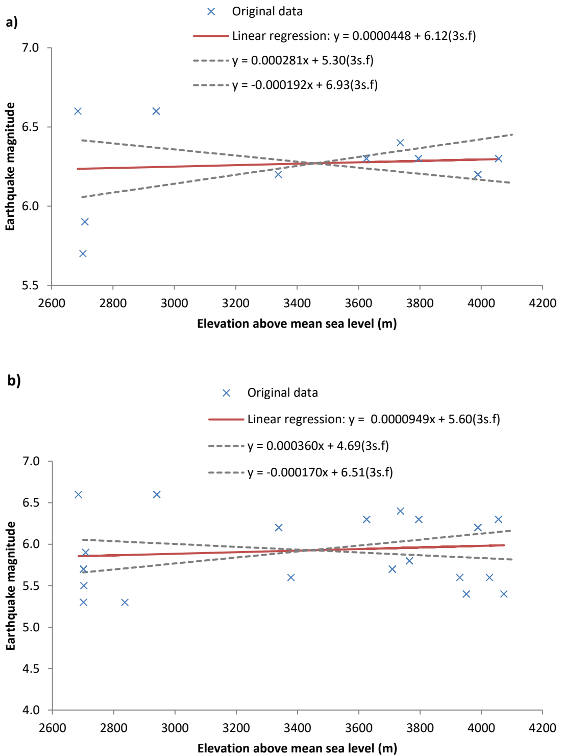
Figure A2.3: Linear regression plots for the sub-sector of the Qilian Shan. The bin width is 500 m and the enveloped considers the a) top 10 %, and b) 20 % of the data. The significance value for (a) 0.30113 and R^2 value is 0.05613. For (b) the significance value is 0.84505 and R^2 value is 0.00108. The graph additionally shows the upper and lower bounds of all the linear regression lines that would remain within the 95 % significance level. In both cases the gradient of the regression line can be seen to switch from positive to negative while remaining at 95 % significance.
