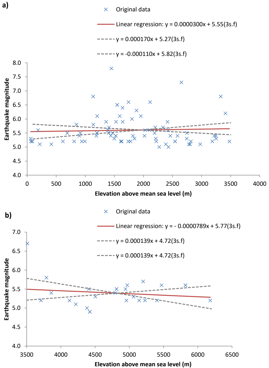
Figure A2.1: Linear regression plots for the Himalayas a) below, and b) above, the defined seismic cut-off. The significance level for (a) is 0.67131 and R^2 value is 0.00232. For (b) the significance value is 0.46257 and R^2 value is 0.02270. The bin width is 500 m and the envelope considers the top 10 % of the data. The graph additionally shows the upper and lower bounds of all the linear regression lines that would remain within the 95 % significance level. In both cases the gradient of the regression line can be seen to switch from positive to negative while remaining at 95 % significance.
