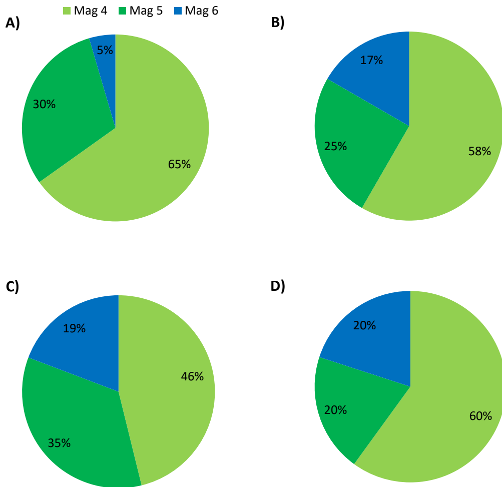
Figure A3.2: Data from the small sub-sector in the Qilian Shan. Pie charts show the area-normalised number of earthquakes at a) 2.5-3.0 km, b) 3.0-3.5 km, c) 3.5-4.0 km and d) 4.0-4.5 km after the 'aftershocks' that occurred within the same month have been removed
