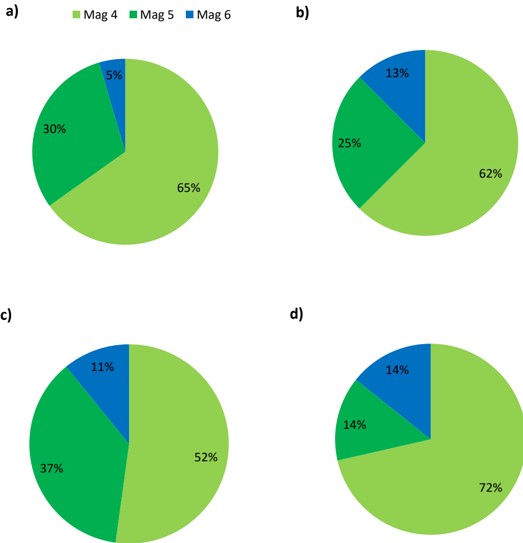
Figure A3.1: Data from the small sub-sector in the Qilian Shan. Pie charts show the area-normalised number of earthquakes at a) 2.5-3.0 km, b) 3.0-3.5 km, c) 3.5-4.0 km and d) 4.0-4.5 km after the 'aftershocks' that occurred within the same day have been removed.
