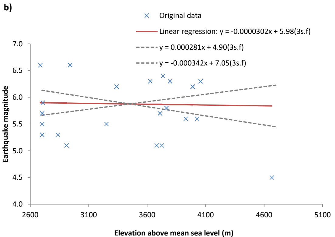
Figure A2.2: Linear regression plots for the sub-sector of the Qilian Shan. The bin width is 250 m and the enveloped considers the a) top 10 %, and b) 20 % of the data. The significance value for (a) 0.30113 and R^2 value is 0.05613. For (b) the significance value is 0.84505 and R^2 value is 0.00108. The graph additionally shows the upper and lower bounds of all the linear regression lines that would remain within the 95 % significance level. In both cases the gradient of the regression line can be seen to switch from positive to negative while remaining at 95 % significance.
