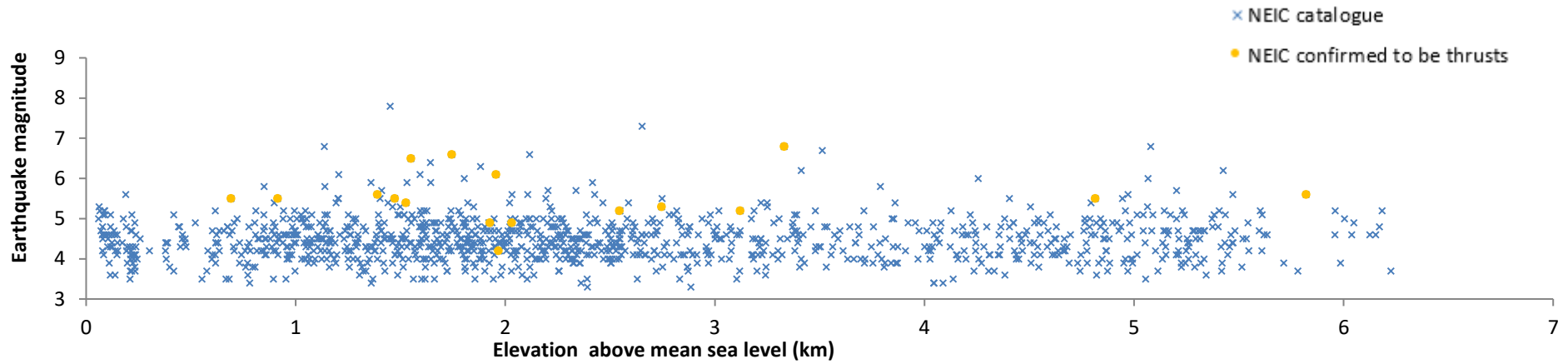
Figure A1.2: Graph showing the earthquake magnitude vs topographic elevation relationship for the whole dataset of Himalayas. Elevations are taken relative to mean sea level from a topography smoothed to 20 km. The majority of the data was acquired from the NEIC catalogue. Events in the NEIC catalogues that were confirmed to be thrusts via cross-coordination with the CMT catalogue, have been plotted using their NEIC coordinates and are labelled as 'NEIC confirmed to be thrusts'.
