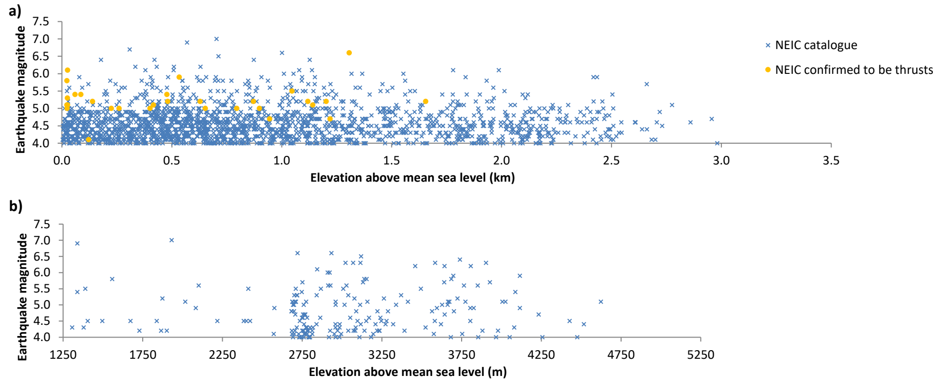
Figure A1.1: Graph showing the earthquake magnitude vs topographic elevation relationship for the whole dataset in a) the Zagros and b) the Qilian Shan prior to the identification of small 'sub-sectors'. Elevations are taken relative to mean sea level from a topography smoothed to 20 km. The majority of the data were acquired from the NEIC catalogue. Events in the NEIC catalogue that were confirmed to be thrusts via cross-coordination with the CMT catalogue, have been plotted using their NEIC coordinates, and are labelled as 'NEIC confirmed to be thrusts'.
