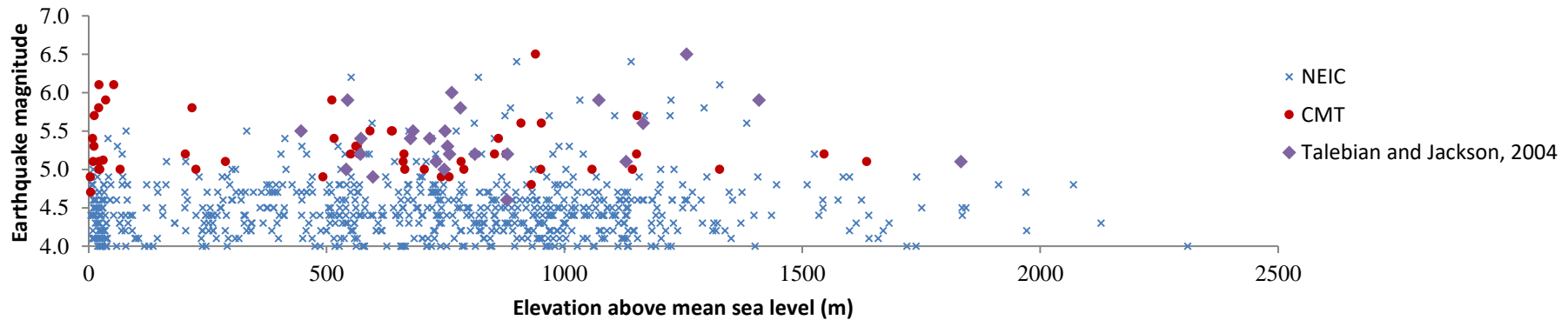
Figure A1.3: Graph showing the earthquake magnitude vs topographic elevation relationship for the small sub-sector of the Zagros. Elevations are taken with respect to mean sea level from a topography smoothed to 10 km. Data is that of Figure 2.5 but the 'NEIC confirmed to be thrusts' have been plotted with their CMT coordinate instead. Despite this M \geq 5 earthquakes still persist above the 1250 m seismicity cut-off.
