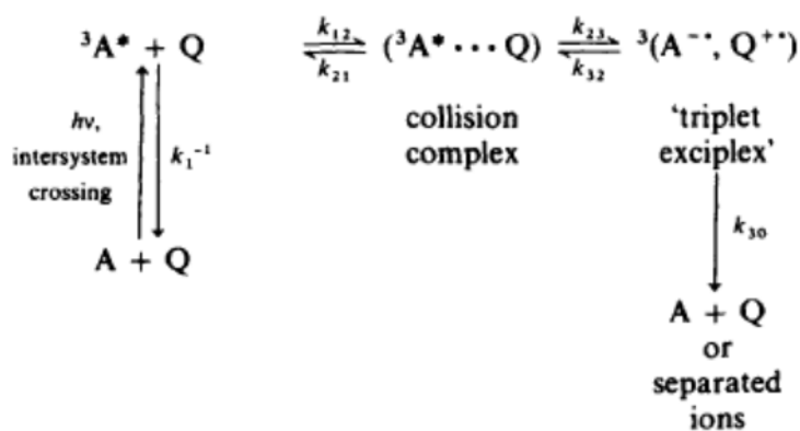
Figure 15 Triplet excited state quenching mechanism of TX, image was taken from 60
