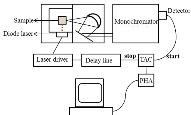
Figure 33 TCSPC equipment
