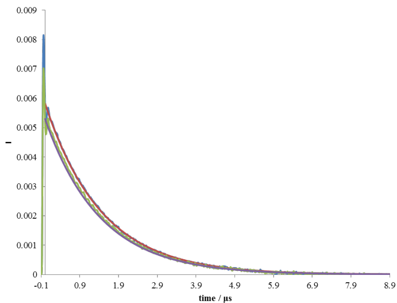
Figure 55 Phosphorescence decay of ^1O_2 in methanol of TX (blue), TX fitting (red), TXCOOH (green), TXCOOH fitting (purple)
