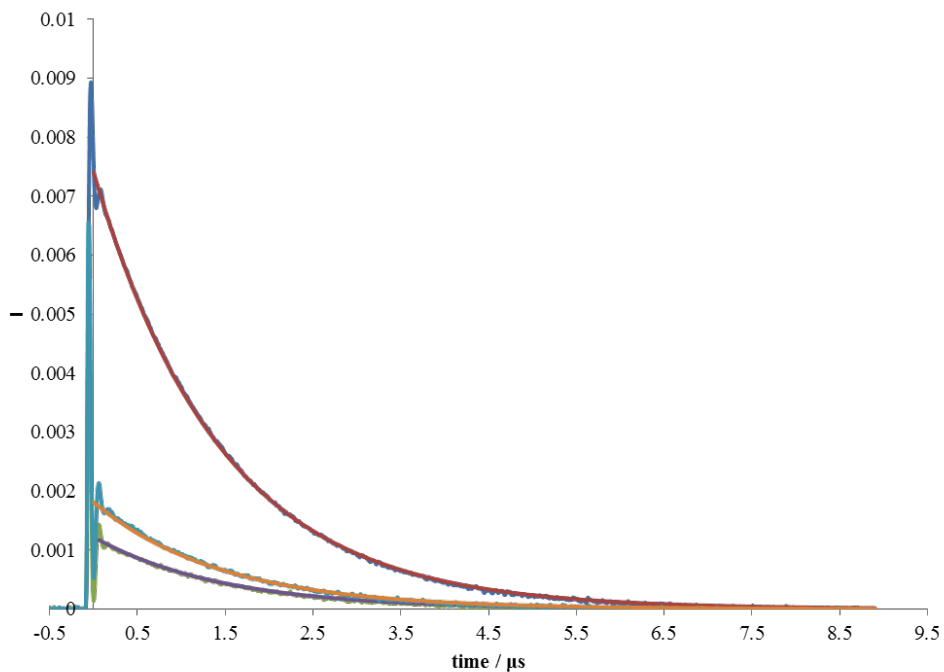
Figure 56 Phosphorescence decay of ^1O_2 in methanol of TXCONC 7 (blue), TXCONC 7 fitting (red), TERTTX (green), TERTTX fitting (purple), TXCOMORPHO (light blue), TXCOMORPHO fitting (orange)
