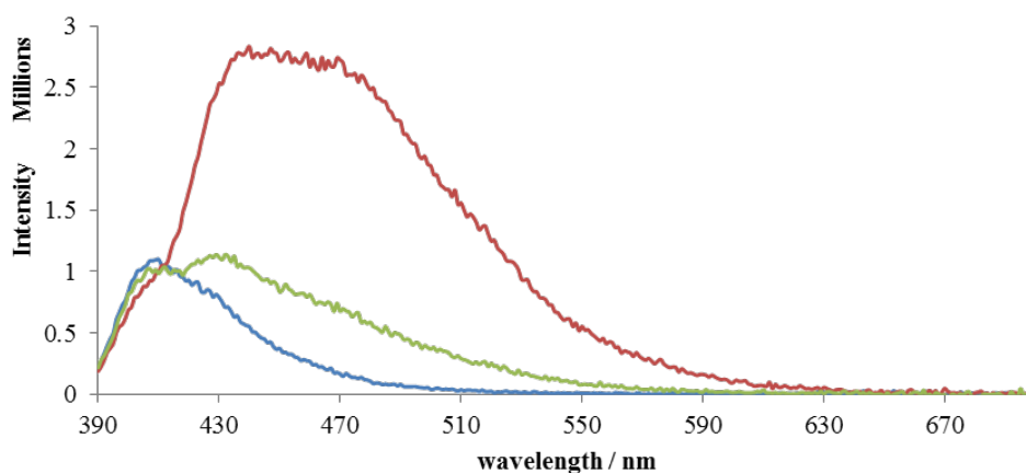
Figure 102 Fluorescence emission of TX at different acid concentrations, \lambda_{exc} 380 nm. Spectra in: DCM (blue), TFA 3.26 \times 10^{-6} M (green), TFA 1.3 \times 10^{-4} M (red).
