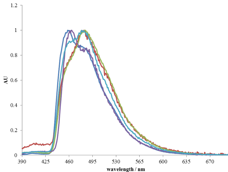
Figure 49 Normalised phosphorescence emission in EPA at 77K \lambda_{ex} 380 nm of TX (blue), TXCOMORPHO (red), TXCOGLY (green), TERTTXMORPHO (purple), TERTTXGLY (light blue)
