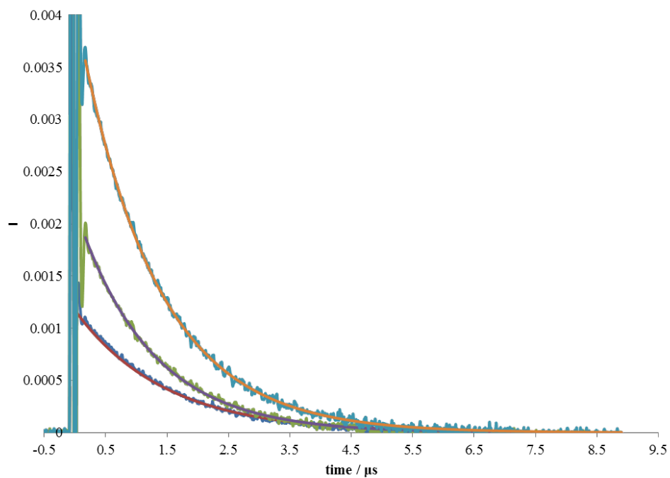
Figure 57 Phosphorescence decay of ^1O_2 in methanol of TERTXMORPHO (blue), TERTXMORPHO fitting (red), TERTTXGLY (green), TERTTXGLY fitting (purple), TXCONET 2 (light blue), TXCONET 2 fitting (orange)
