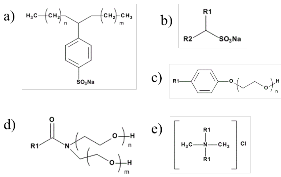
Figure 3 a) LAS general structure n+m=7-10 b) Secondary Alkanesulfonates (SAS) R1 and R2 C_{11-17} c) Alkylphenol Ethoxylates (APE) R1 C_{8-12} n 5-10 d) Fatty Acid Alkanolamides (FAA) R C_{11-17} n 1,2 m 0,1e Dialkyldimethylammonium Chlorides R C_{16-18}
