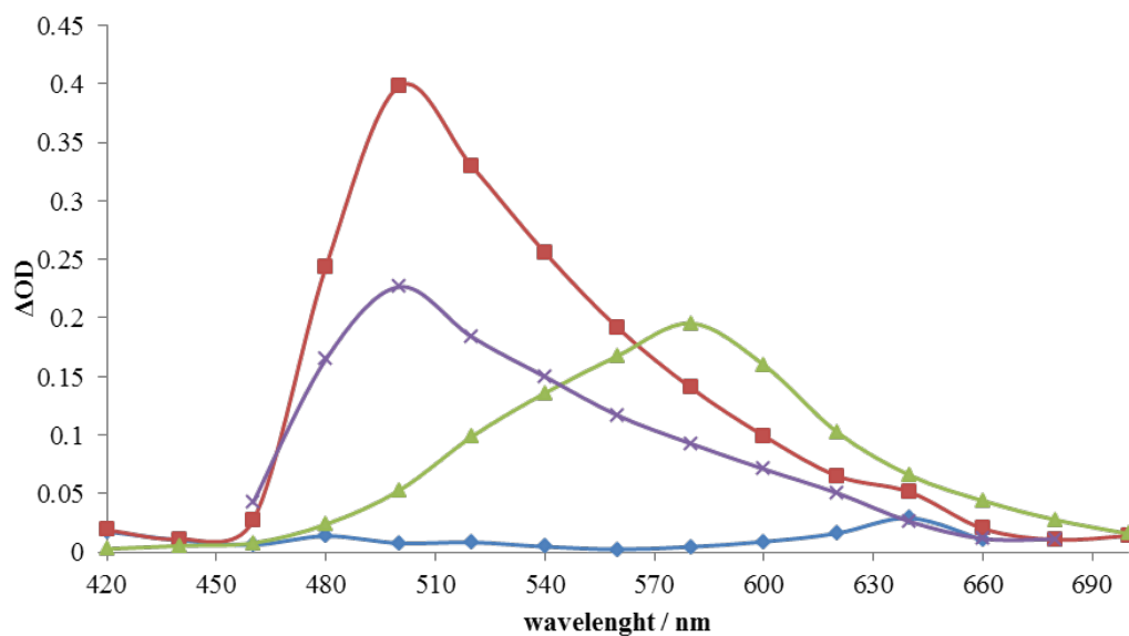
Figure 107 Triplet-triplet absorption spectra of TX: DCM (blue), MeOH:H 2 O (green), H 2 SO 4 (13 M) (purple), TFA (13 M) (red).
