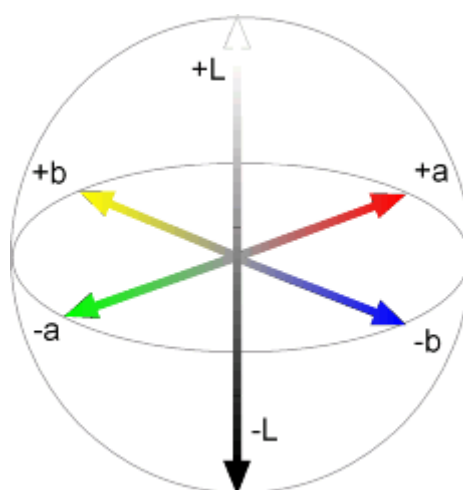
Figure 87 L,a,b colour space
