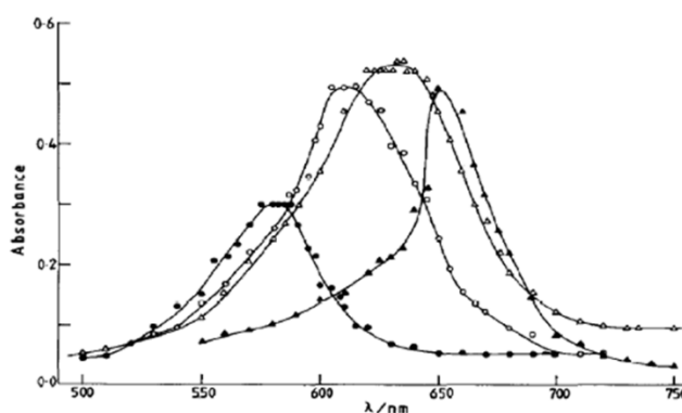
Figure 22 Triplet-triplet absorption spectra of TX obtained on laser flash photolysis of deaerated solution: triangle in acetonitrile measured 5 μs after the end of the excimer laser pulse; circle in ethanol measured 2 μs after the end of the ruby laser pulse; full circle in 2,2,2-trifluoroethanol measured 2 μs after the end of the ruby laser pulse; full triangle in cyclohexane measured 500 ns after the end of the excimer laser pulse. Figure is taken from 71
