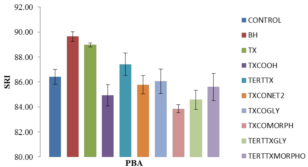
Figure 126 SRI values of vinalool with a PBA concentration of 0.5 mg/L with detergent
