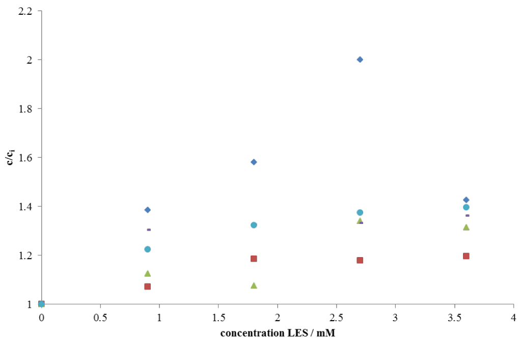
Figure 80 Concentration changing of TX (blue), TERTTX (red), TXCOOH (green), TXCOGLY (purple), TXCOMORPHO (light blue), TXCONC 7 (orange) upon concentration of LES
