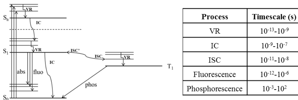
Figure 4 Jablonski diagram
