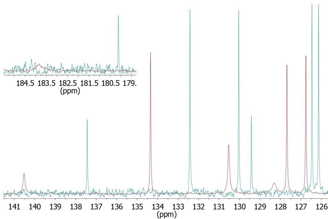
Figure 93 C-NMR of protonated TX in CDCl_3 and TFA (red) and not protonated (blue).
