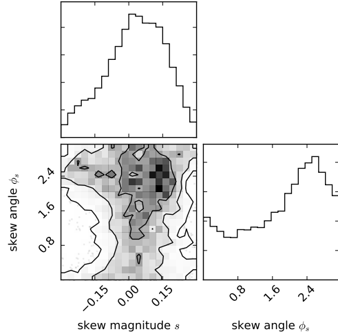
(c) Galaxy N2
