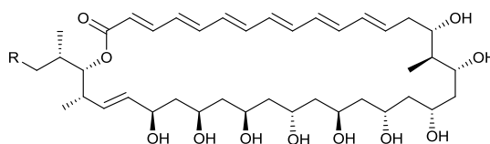
dermostatin A 124 R = H
