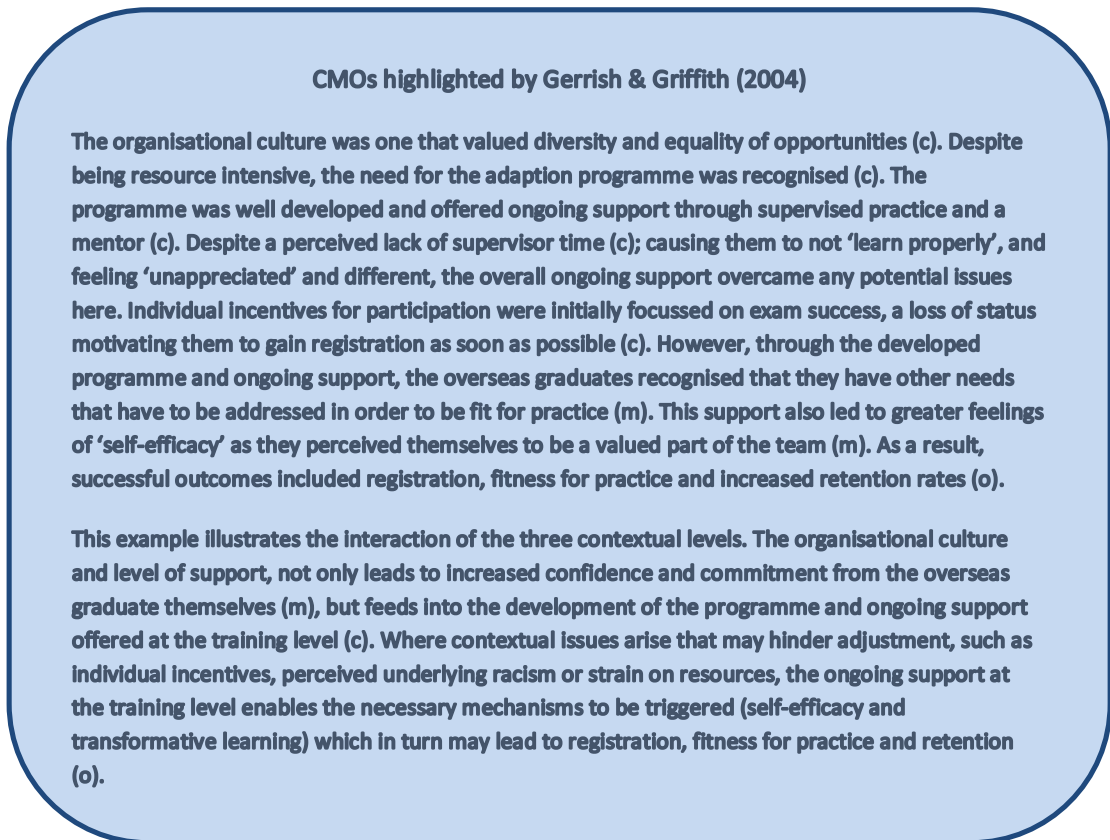
Figure 12. Use of theory to explain why Gerrish & Griffith 195 reported successful intervention outcomes
