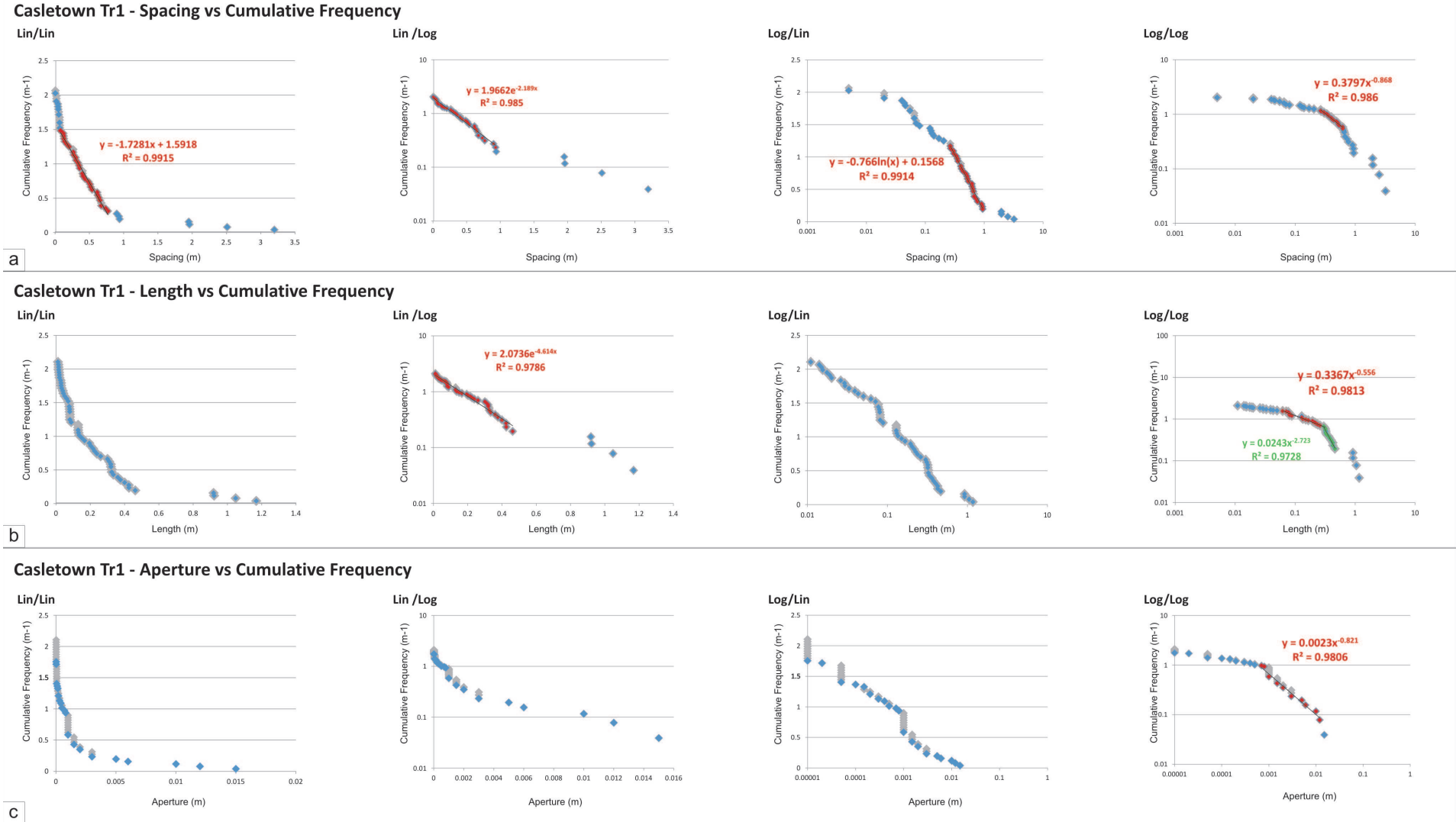
Figure D.6: Lin-Lin, Lin-Log, Log-Lin, Log-Log cumulative distribution plots for the transect Casletown Tr1 (a) spacing and (b) length and (c) aperture
