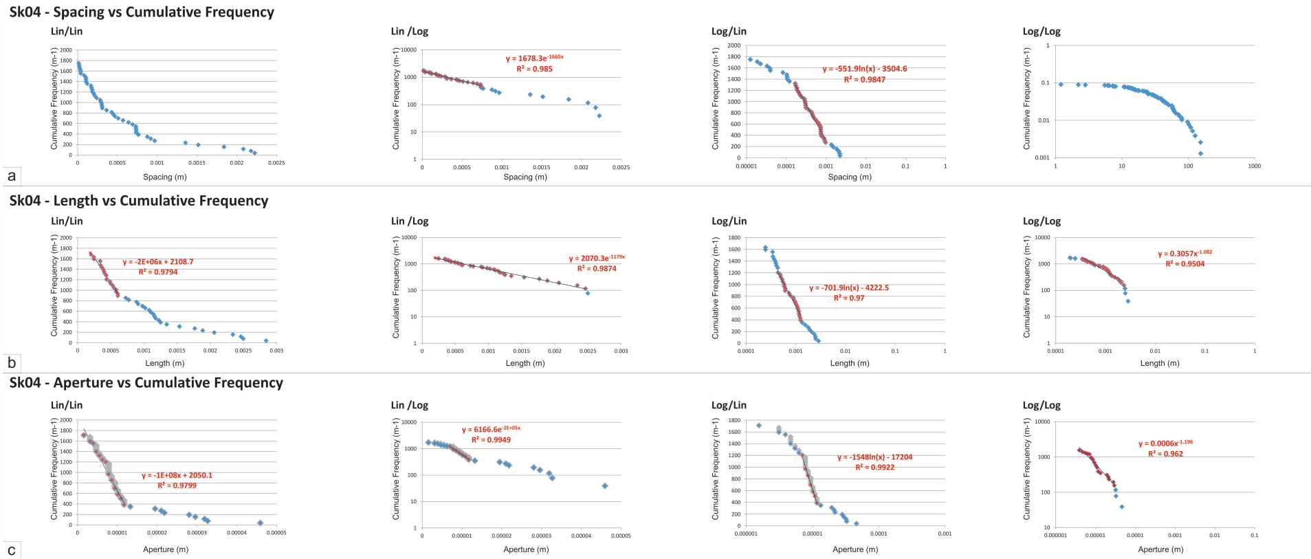
Figure D.10: Lin-Lin, Lin-Log, Log-Lin, Log-Log cumulative distribution plots for the transect Sk04 (a) spacing and (b) length and (c) aperture
