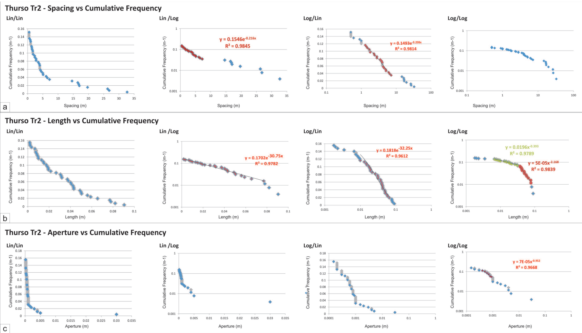
Figure D.9: Lin-Lin, Lin-Log, Log-Lin, Log-Log cumulative distribution plots for the transect Thurso Tr2 (a) spacing and (b) length and (c) aperture
