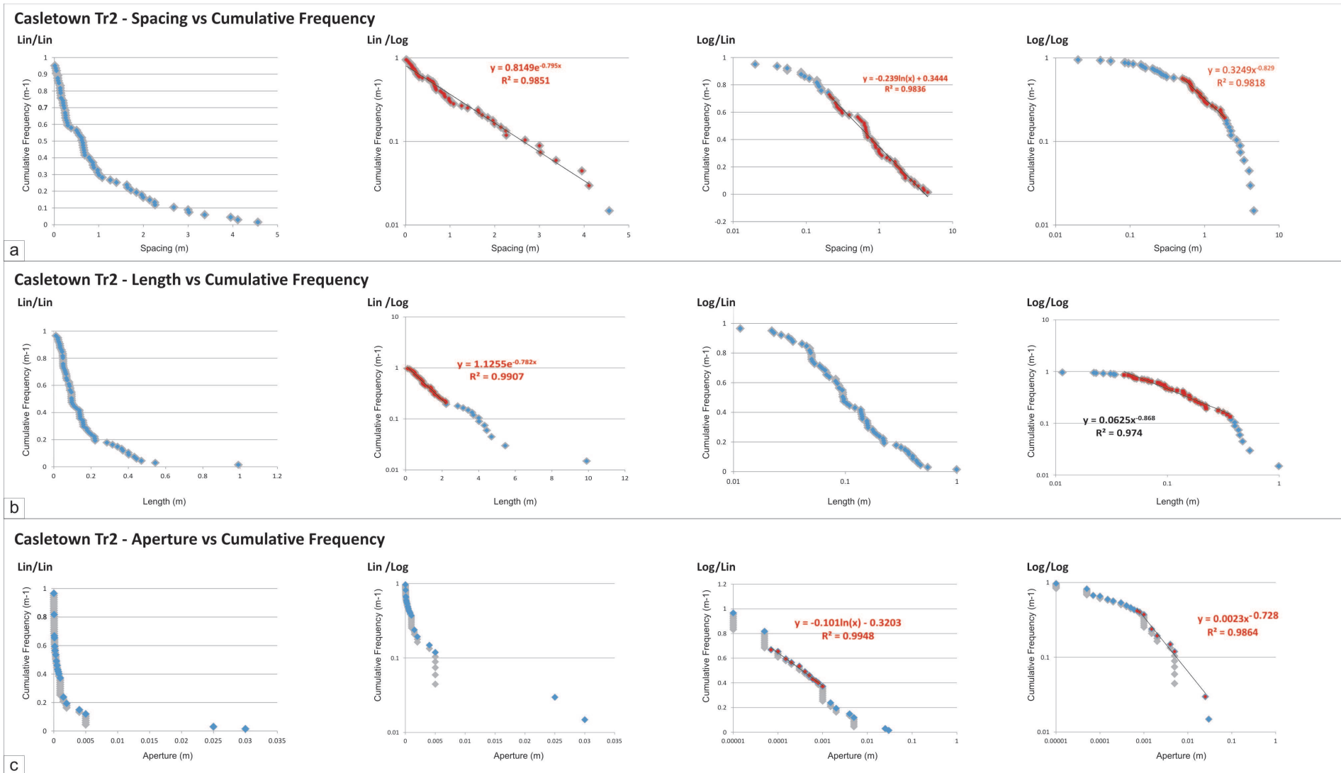
Figure D.7: Lin-Lin, Lin-Log, Log-Lin, Log-Log cumulative distribution plots for the transect Castletown Tr2 (a) spacing and (b) length and (c) aperture
