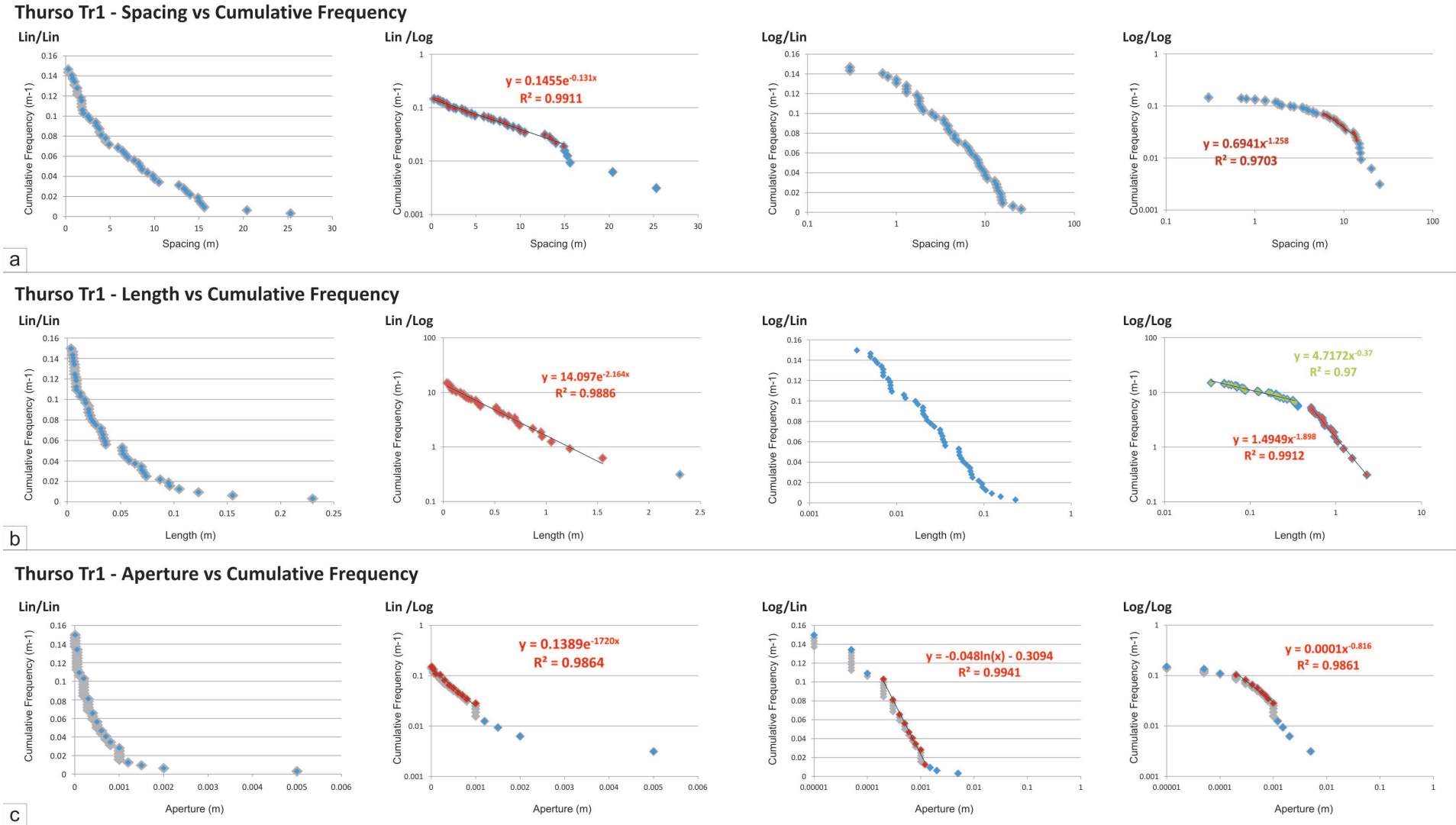
Figure D.8: Lin-Lin, Lin-Log, Log-Lin, Log-Log cumulative distribution plots for the transect Thurso Tr1 (a) spacing and (b) length and (c) aperture
