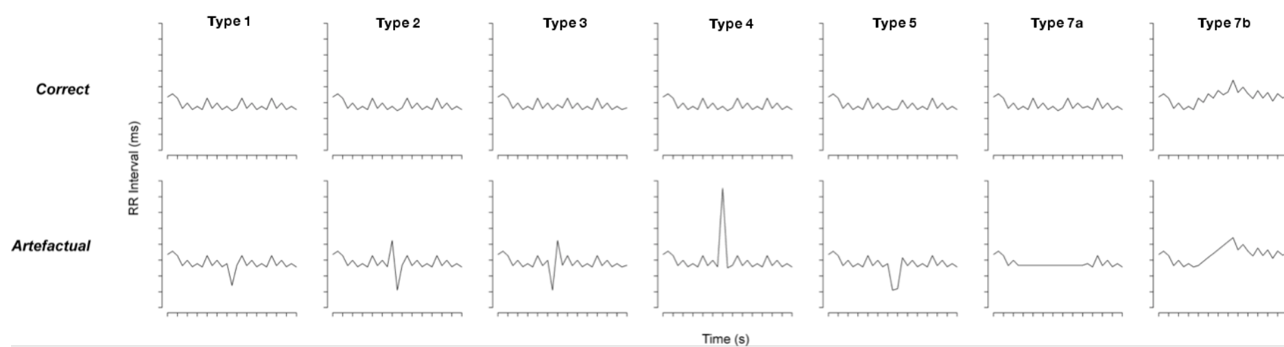
Figure 2.6. Common artefacts in Polar ® RR interval recordings. Type 1 to 5 artefacts are categorised as “Peaks”. Type 1 artefacts are single point discrepancies that can be either positive or negative. Type 2 artefacts are characterised by a long RR interval (i.e. a “spike”) followed by a compensatory short RR interval (i.e. a “trough”). Type 3 artefacts are similar to Type 2 artefacts, except they are characterised by a short RR interval followed by a compensatory long RR interval. Type 4 artefacts are characterised by 2–3 extremely long RR intervals, often two or three times longer than the surrounding RR intervals. Type 5 artefacts are characterised by a flat-bottomed trough, consisting of two short RR intervals. Type 7a and Type 7b artefacts are categorised as “Flats” and “Stairs”, respectively. Type 7a artefacts occur when an RR interval is the same as the interval preceding it. Type 7b artefacts occur when the difference between successive intervals is the same. Taken and adapted from Marchant-Forde et al. (2004) and Jonckheer-Sheehy et al. (2012).
