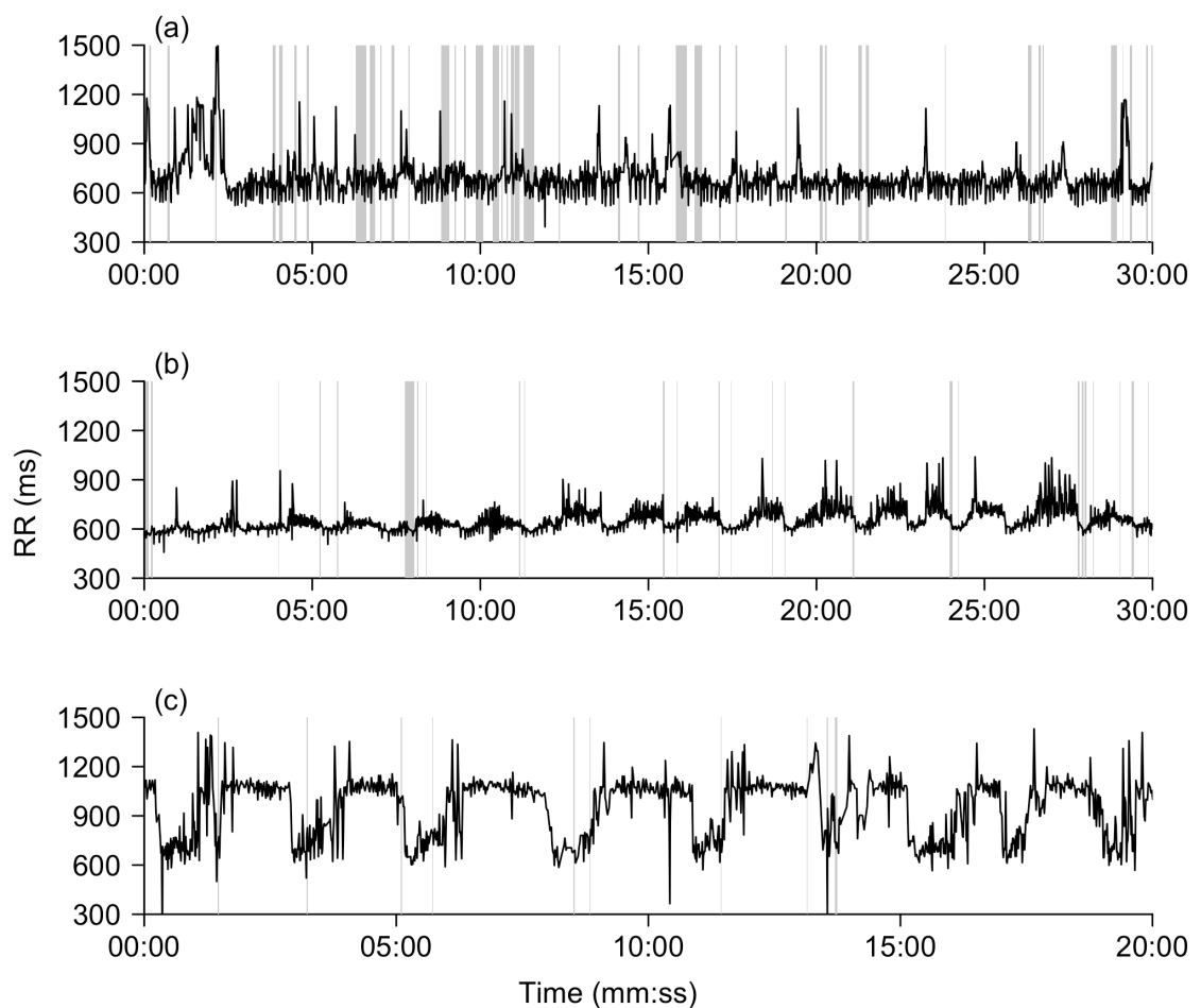
Figure 3.1. Examples of RR intervals recorded using Polar® devices from three different female grey seals on the Isle of May, Scotland during rest. The two main patterns observed were steady, variable HR (a) , and episodes of slight (b) and pronounced (c) bradycardia. Light grey blocks indicate periods of Vigilance.
