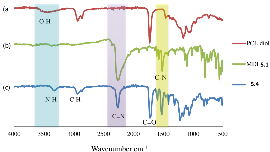
Figure 5.15: FT-IR spectra of (a) PCL diol, (b) MDI 5.1 and (c) MDI-PCL-MDI diisocyanate prepolymer 5.4
