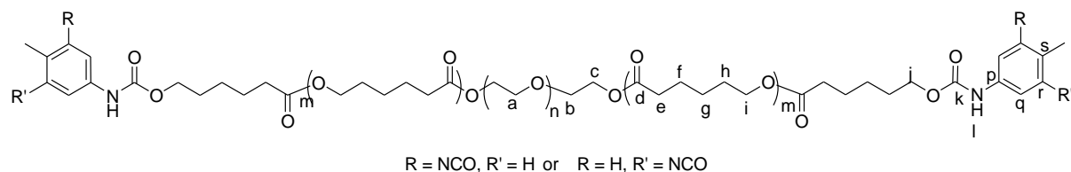
Figure 5.4: TDI-based Diisocyanate Prepolymer containing a central PCL- b -PEG- b -PCL moiety with a \overline{DP} of 50 per arm 5.5
