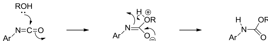
Scheme 1.1: Mechanism of the nucleophilic attack at an isocyanate
