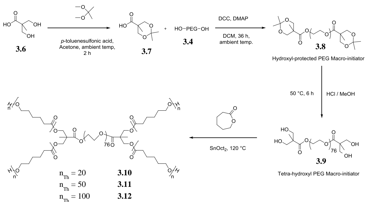
Scheme 3.3: Synthesis of four-arm star (PCL) 2 -b-(PEG)-b-(PCL) 2 3.10 – 3.12
