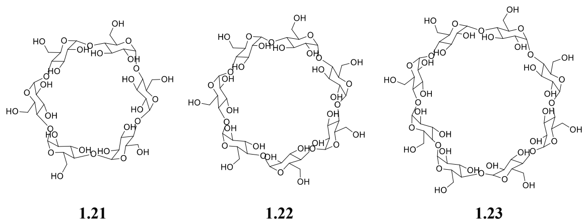
Figure 1.6: Structures of \alpha -CD 1.21 , \beta -CD 1.22 and \gamma -CD 1.23
