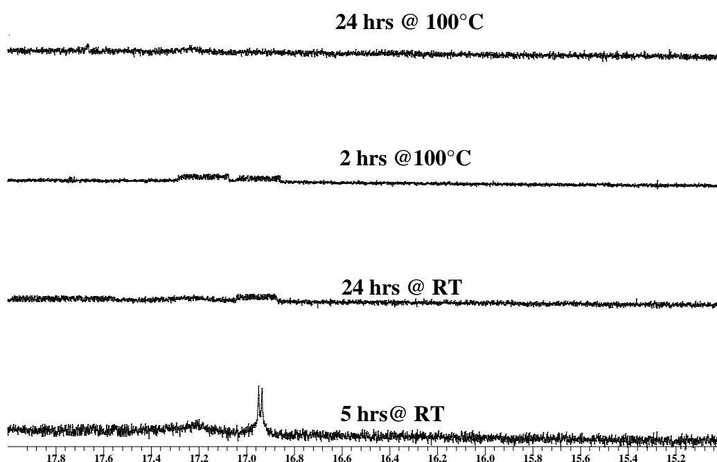
Figure 3.24. 400 MHz ^1\text{H} NMR spectra showing the alkylidene region for the ROMP reaction of exo -N-ethylhexyl norbornene-5,6-dicarboxyimide monomer using chelated product of (3.2.1) as an initiator with the ratio of monomer: initiator (10:1) in \text{C}_7\text{D}_8
