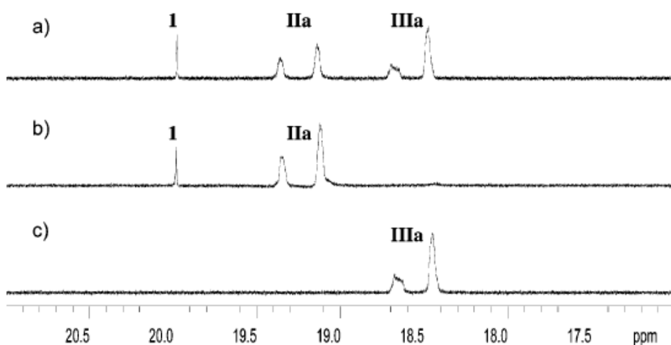
Figure 1.23. Alkydene region of the 1 H NMR spectrum when (a) is subjected to ROMP reaction with Grubbs 1 st generation initiator ( I 5 ), (b) upon the addition of 5 equiv. of Cy 3 and (c) upon the addition of 10 equiv of CuCl. [M] 0 /[I] 0 =20, [I] 0 =15 mM 98
