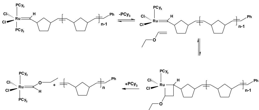
Scheme 1.12. The termination step using \text{RuCl}_2(\text{PCy}_3)_2(=\text{C}(\text{H})\text{Ph}) for ROMP
