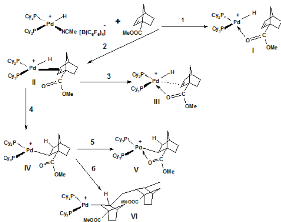
Scheme 3.11. Addition polymerisation of norbornene-1-methyl carboxylate monomer using palladium initiator [\text{Pd}(\text{H})(\text{PCy}_3)_2(\text{CH}_3\text{CN})][\text{B}(\text{C}_6\text{F}_5)_4]
