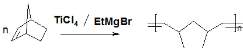
Scheme 1.6. Polymerisation of norbornene proposed by Anderson and Merckling in 1955
