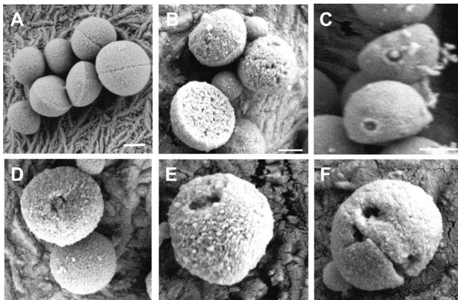
Figure 1.8. Scanning electron microscopy images to show the action of cyclic peptoids on bacterial cell membranes. A untreated cells; B–F cells incubated with peptoid 59 at the MIC value of 3.9\ \mu\text{M} for 18 hours. Reprinted with permission, copyright 2013 John Wiley and Sons. ††,73
