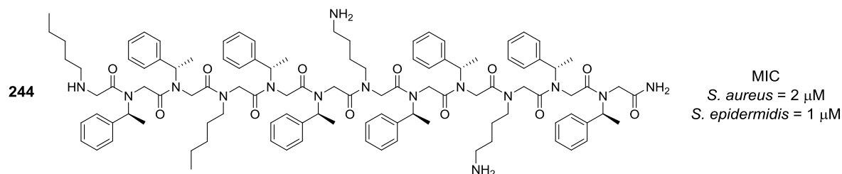
Figure 4.7. Example structure for peptoid 244 where charged NLys residue is replaced by Namy .
