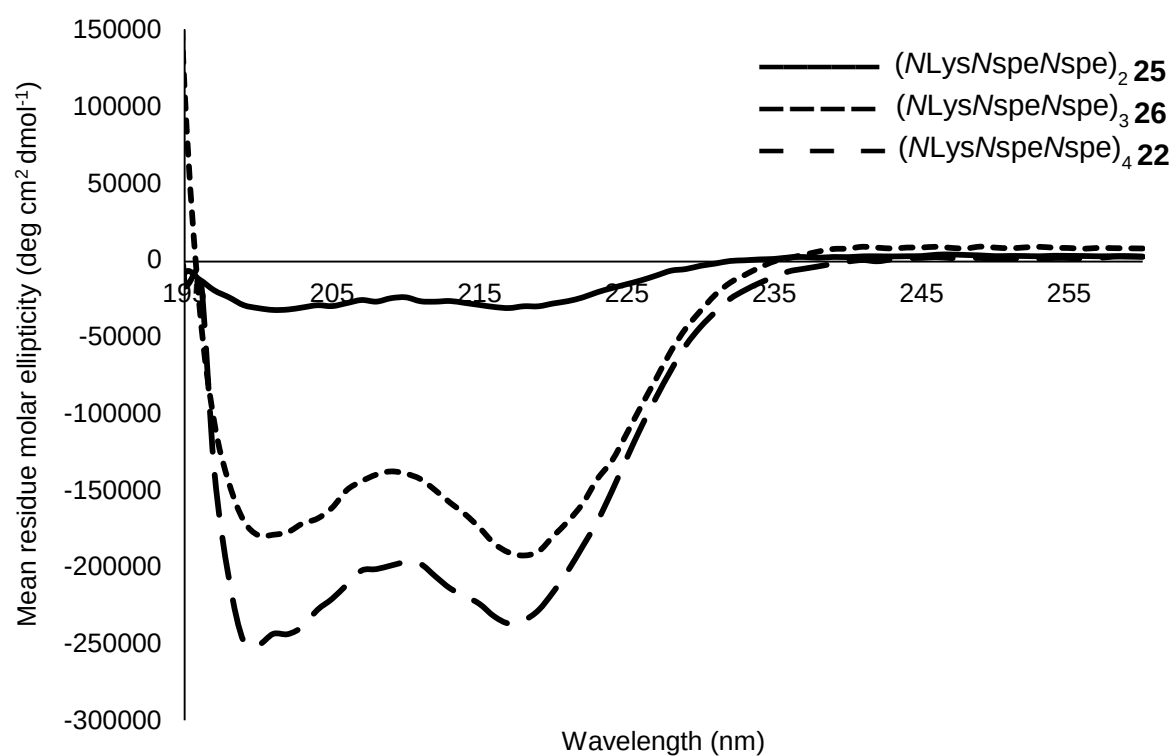
Figure 2.26. CD spectra for peptoid sequences of different lengths containing the \alpha -chiral Nspe monomer, peptoids 22 , 25 , 26 . Data collected at 50 \mu\text{M} in PBS (pH 7.4) at 22 ^{\circ}\text{C} . The structure of the 12 residue sequence 22 is shown. The samples show characteristic signals of peptoid helices.
