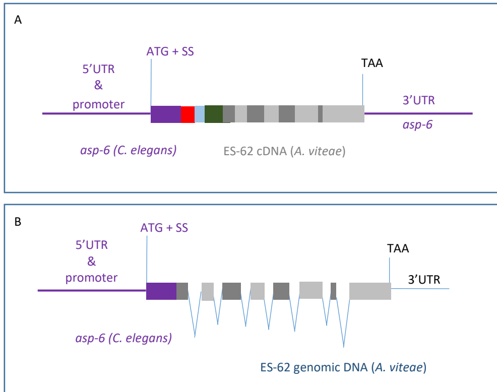
Figure 3.11. Schematic diagram of the asp-6::ES-62 fusion constructs. A) The asp-6::ES-62 cDNA construct consists of 5'UTR, promoter, ATG and signal sequence from C. elegans asp-6 gene fused to ES-62 cDNA from A. viteae and to 3'UTR from C. elegans asp-6 gene. B) The asp-6::genomic ES-62 construct consist of 5'UTR, promoter, ATG and signal sequence from C. elegans asp-6 gene fused to ES-62 genomic DNA fragment from A. viteae with ES-62 3'UTR. asp-6::genomic ES-62 construct contains a large part of genomic ES-62 fragment and not the whole gene.
