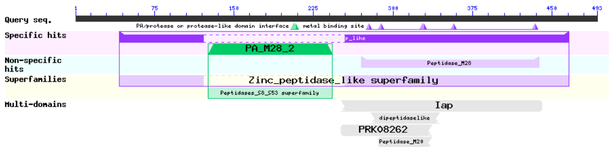
Figure 1.5. Graphical summary of conserved domains on ES-62 (protein BLAST). The BLAST alignment includes ES-62 in the Zinc-peptidase-like superfamily, due to the structural similarities, however, it was found that the active site of ES-62 contains a magnesium cation (Section 1.6.2.).
