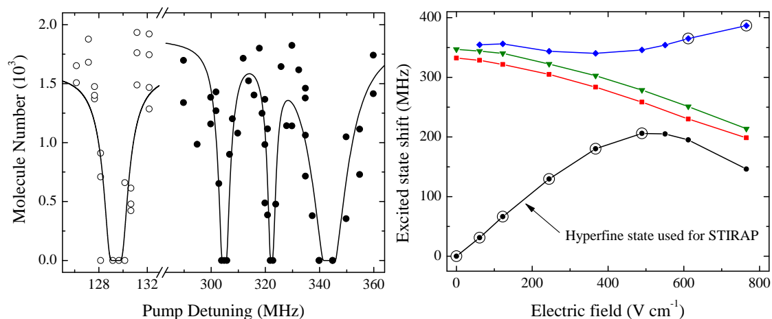
Figure 4.10: One photon Stark spectroscopy from the | -6(2,4)d(2,4) \rangle state close to dissociation. (a) Spectroscopy of the four hyperfine sublevels of the |\Omega' = 1, v' = 29, J' = 1\rangle state observed with an applied electric field of 245 V/cm. Empty circles show data collected with a pump power of 69 \mu\text{W} , filled circles show a pump power of \sim 15.6 mW. (b) Stark shift of these states up to an applied electric field of 765 V/cm. The lowest hyperfine sublevel is used for STIRAP transfer to the rovibrational ground state. An avoided crossing is observed between that state and the higher-lying hyperfine states at an applied electric field of \sim 550 V/cm. Circles show the state used for the ground-state spectroscopy in figure 4.11.
