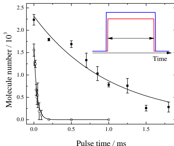
Figure 4.7: Decoherence of the dark-state resonance using the |a^1\Sigma^+ + b^3\Pi_1, v' = 29, J' = 1\rangle intermediate state. Black squares show the loss of molecules with the Stokes laser on resonance with the rovibrational ground state. Open circles are with the pump laser only, for comparison. The curves are exponential decay fits, with \tau = 1.0(1) ms with the Stokes and \tau = 40(5) \mu s without. There is a large range of times from 0.2 ms \rightarrow 1.25 ms where molecules only remain when the Stokes is on, which shows that this intermediate state is suitable for two-photon spectroscopy. Inset: pulse sequence sketch (not to scale). Pump and Stokes are red and blue respectively.
