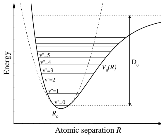
Figure 2.4: Vibrational levels of a diatomic molecule. Near the equilibrium separation R_0 , the potential is approximately parabolic as shown in the dashed line.
