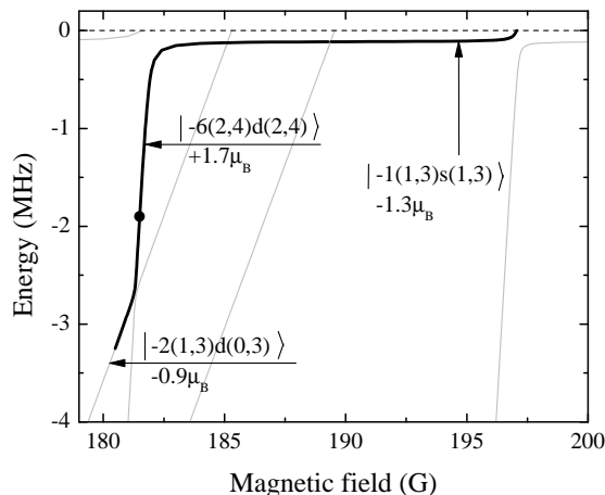
Figure 1.3: Near-dissociation molecular Feshbach states in the magnetic field range we use, relative to the combined ^{87}\text{Rb} |F = 1, m_F = 1\rangle and Cs |3, 3\rangle energies. The solid line shows the Feshbach states we can occupy, and the dot shows the state and magnetic field we use for STIRAP. The magnetic moments of each state are labelled.
