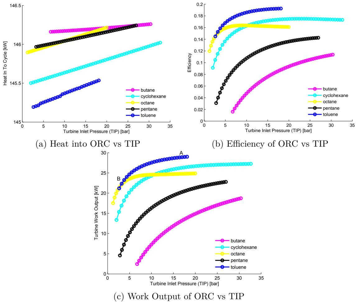
Figure 2.12: Engine case cycle simulations with mass flow rate constrained to 0.6m_O
