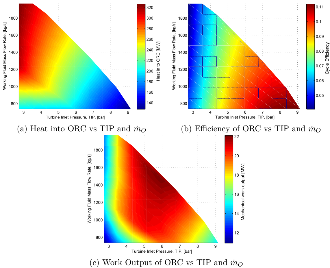
Figure 2.14: Results of Ninian oil field simulations, with working fluid R245fa. Hot brine temperature is 102^\circ and mass flow rate 1231.1 kg/s
