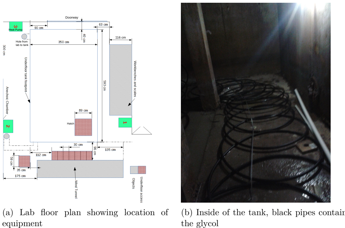
Figure 3.4: Physical layout of experimental rig
