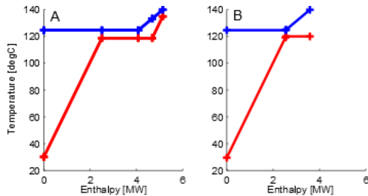
Figure 2.11: T-HPlots of Industrial case evaporator with R245fa working fluid for cycles A and B as labelled in Figure 2.10c
