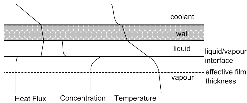
Figure 4.2: Temperature, concentration and heat flux profiles during condensation of a mixture
