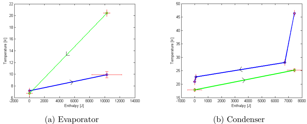
Figure 3.16: Temperature-Enthalpy plots for heat exchangers with R407c
