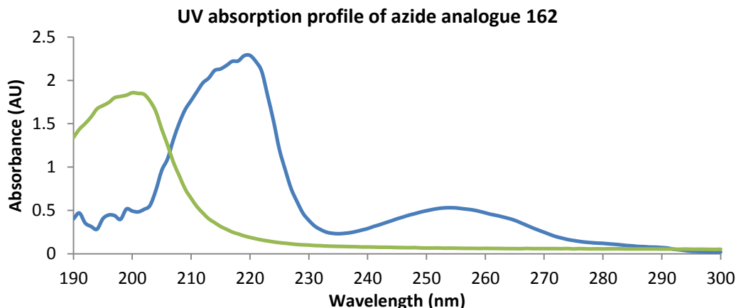
Figure 6–6: UV absorption profile of azide 162 (blue line) at 25 \mu\text{M} in 50 mM phosphate buffer with 600 \mu\text{M} CHAPS. The green line represents blank buffer.
