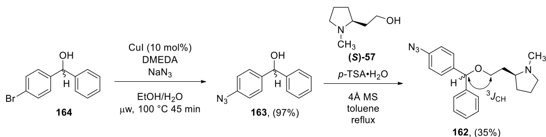
Scheme 6–5: Synthesis of azide clemastine analogue 162
