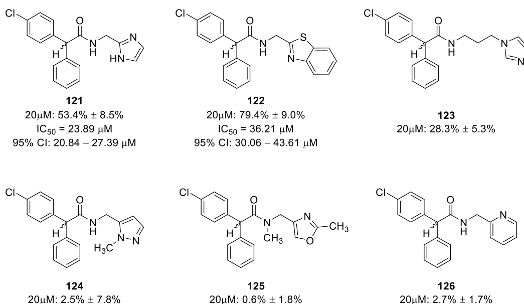
Figure 4–6: Example aromatic N -heterocyclic analogues tested
