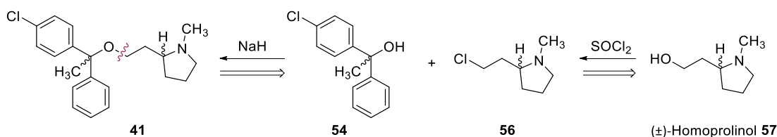
Scheme 3–2: Literature precedent for the synthesis of clemastine 41
