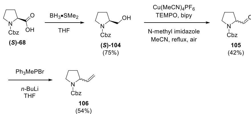
Scheme 3–34: Synthetic route to alkene 106 from ( S )- N -Z-proline ( S )-68
