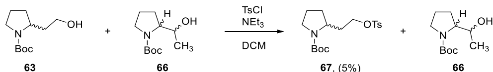
Scheme 3-7: Tosylation of alcohol mixture 63 and 66
