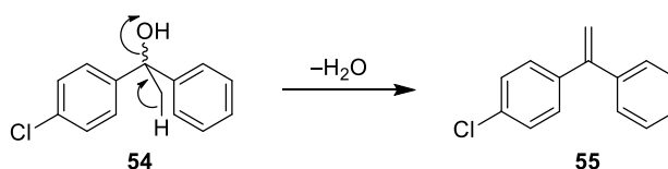
Scheme 3–1: Instability of alcohol 54
