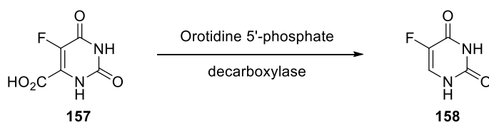
Scheme 6–1: Biosynthesis of 5-fluorouracil 158, catalysed by orotidine 5'-phosphate decarboxylase
