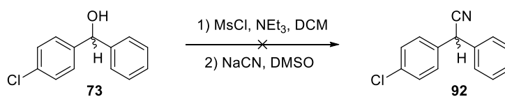
Scheme 3–26: Failed homologation attempt of benzhydrol 73
