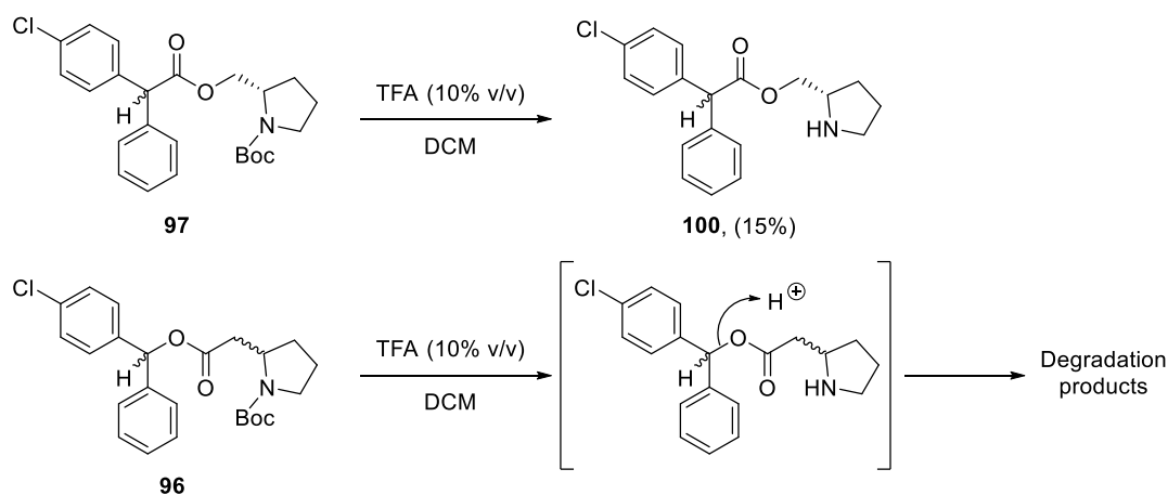
Scheme 3–32: Attempted carbamate deprotection of esters 96 and 97
