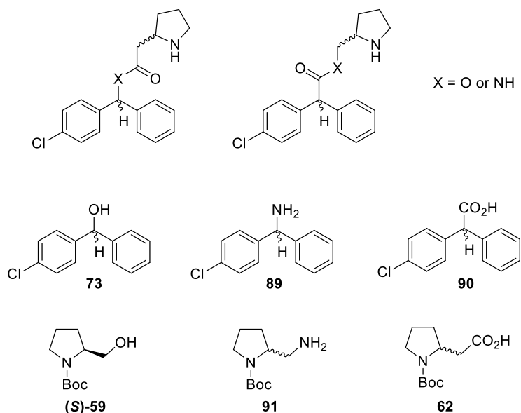
Figure 3–5: Precursors required for synthesis of acyl-linked clemastine analogues
