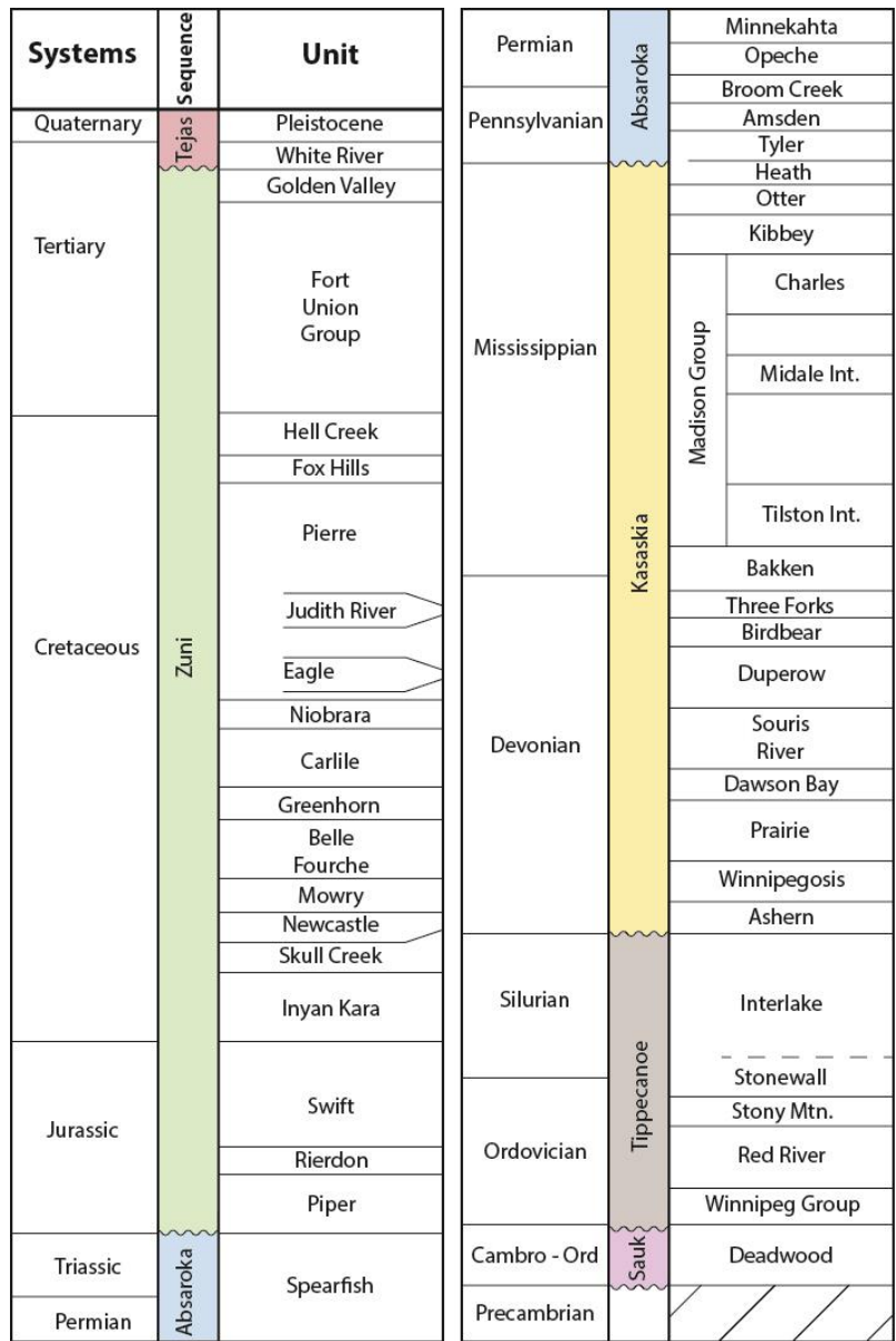
Figure 2.2 - Stratigraphic column of the Williston Basin, showing the Devonian-Mississippian Bakken Formation. After Gerhard et al., (1982) & Webster (1984).
