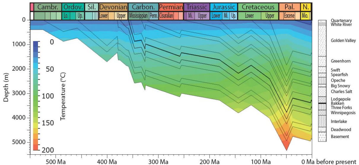
Figure 2.7 - Burial history of the Williston Basin developed for the basin centre in North Dakota (see Figure 2.1 for location). The temperature through time is overlain. Camb - Cambrian, Ordov - Ordovician, Sil - Silurian, Carbon - Carboniferous, Pal - Paleogene, N - Neogene, Up - Upper, Mi - Middle, Lo - Lower, Penn - Pennsylvanian, Mio - Miocene. From Kuhn, (2012).
