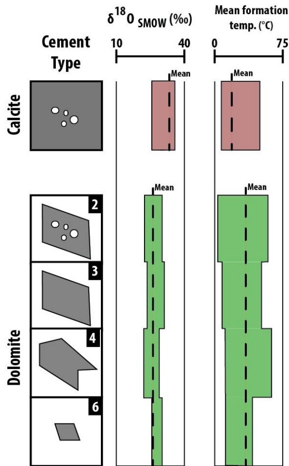
Figure 5.18 – Schematic summarising the differences in oxygen isotope composition and calculated formation temperature in different textures of carbonate phases calcite and dolomite.
