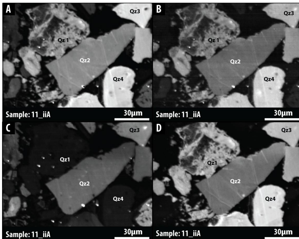
Figure 3.8 - Detrital quartz grains showing different CL character to each to other in sample 11_iiA, 800x A) Panchromatic B) Red C) Green D) Blue.
