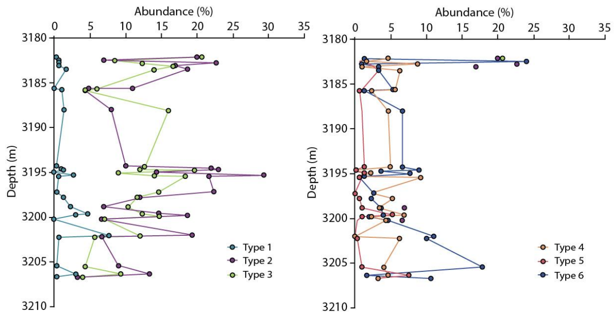
Figure 3.17 - Abundance of different dolomite phases obtained by point counting of thin-sections. Data is split into two plots for clarity.
