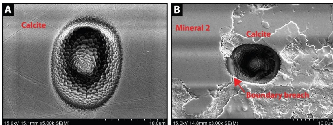
Figure 5.8 - Examples of SIMS pits a) Regular pit, positioned in the centre of a calcite crystal in sample 2-55B; note the ellipsoidal shape and size; b) Irregular pit positioned at the edge of calcite cement, breaking into a second mineral (mineral 2), contaminating the ablated sample, in sample 2-55B.
