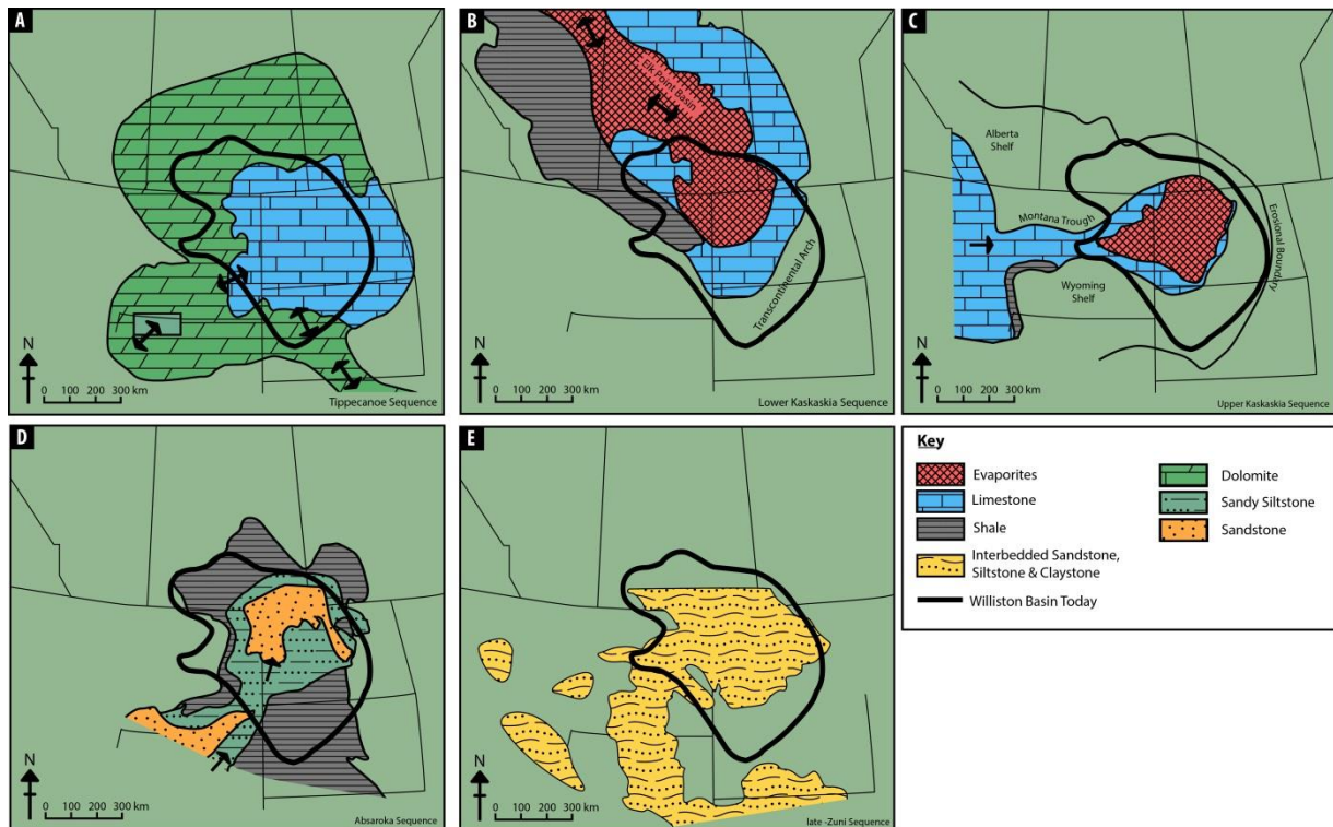
Figure 2.3 - Sequential maps for the time periods of key changes to basin sedimentation, showing source direction of sediment and lateral extent of deposition. A) Tippecanoe sequence B) Lower Kasaskia Sequence C) Upper Kasaskia sequence D) Absaroka sequence E) Late Zuni sequence. After Gerhard et al. (1982) and Peterson & MacCary (1987).
