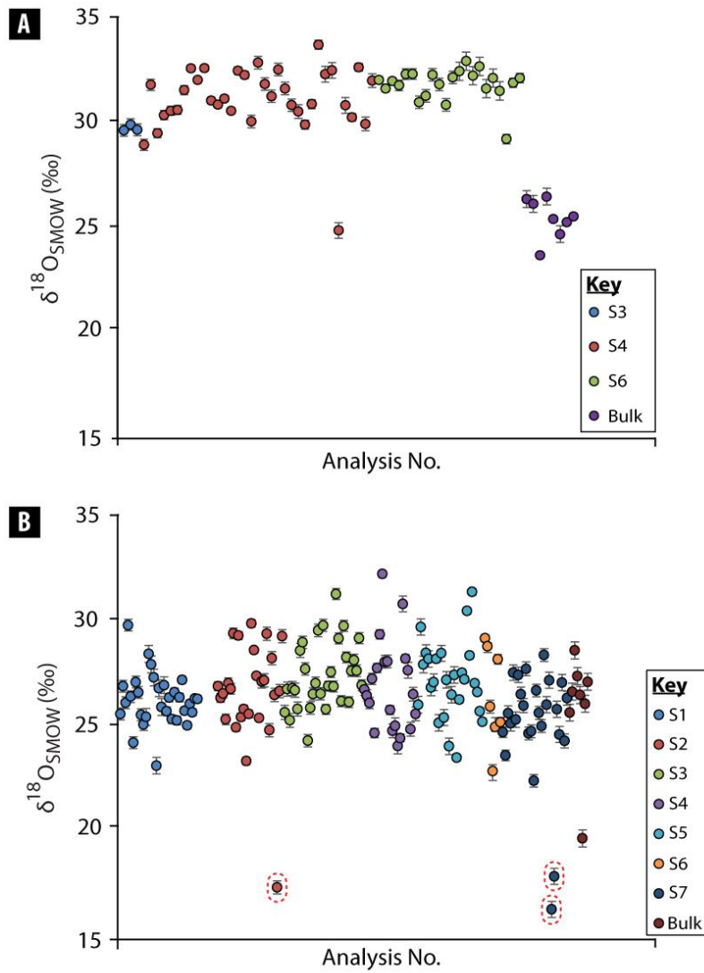
Figure 5.11 - Plot of grain- scale oxygen stable isotope data collected by SIMS from calcite grains. a) Calcite by sample b) Dolomite by sample. Anomalies identified above, circled with red dashed lines. Sx = sample number, e.g. S1 = sample 1.
