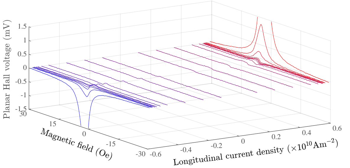
Figure 5.6: Variation of the PHE voltage with magnetic field sweeps taken at \theta = 0^\circ at different current densities.
