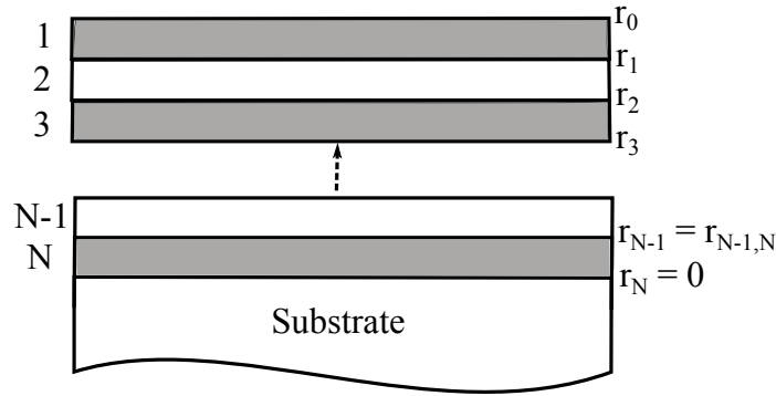
Figure 3.8: Demonstration of the interface and layer label notation used in the Parratt recursive formalism. The Fresnel reflectivity for the substrate interface is r_N . The recursive formalism is applied from the substrate working upwards in steps of N-1 to the surface interface r_0 .
