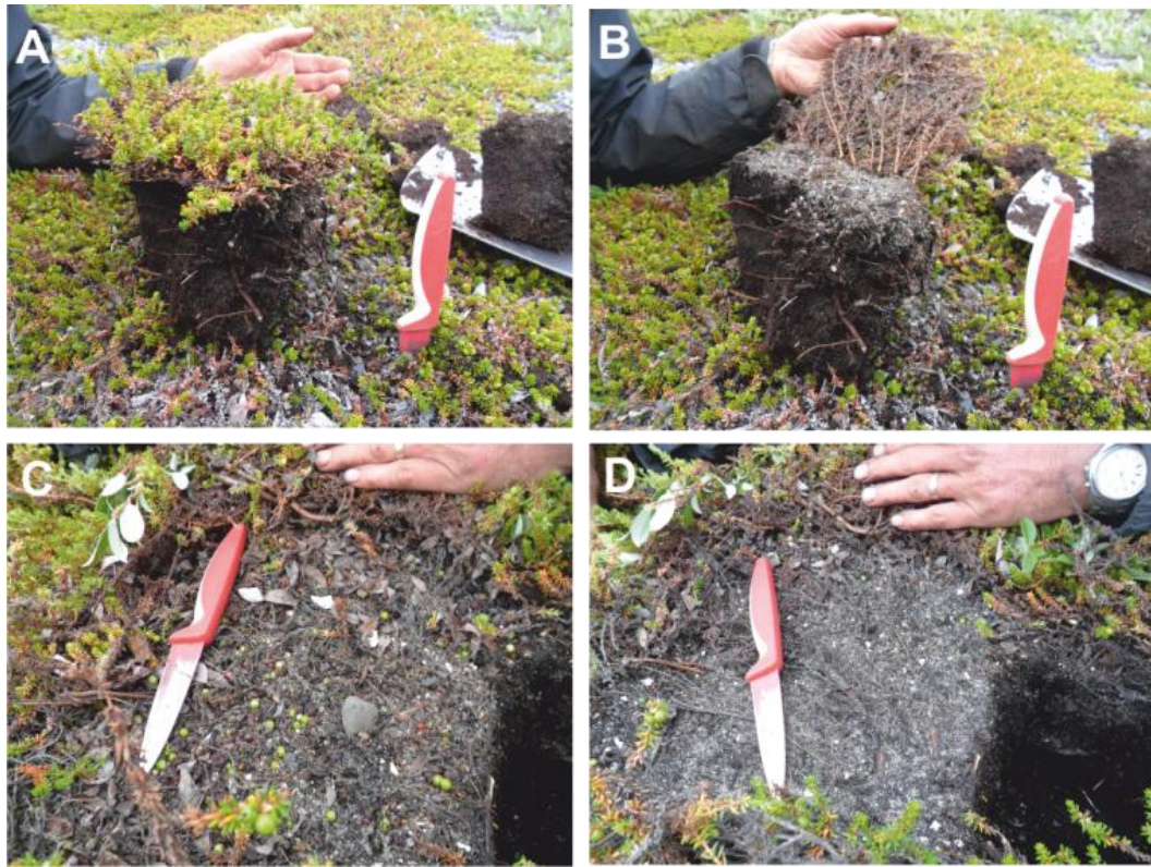
Figure S5. Excavation of the coastal lowland and living Empetrum nigrum surface near Sandstone Point. a, Hand-dug pit revealing E. nigrum in growth position and thickly-rooted underlying peat. b, Removal of E. nigrum surface reveals AD 2000 tsunami deposit comprising sands and gravels that have not been worked into underlying soil by thick E. nigrum rhizomes. In this example, E. nigrum has rooted surrounding soil. c, Second example AD 2000 tsunami deposit, following removal of E. nigrum surface. d, Removal of the AD 2000 tsunami deposit reveals flattened pre-tsunami E. nigrum rhizomes.
