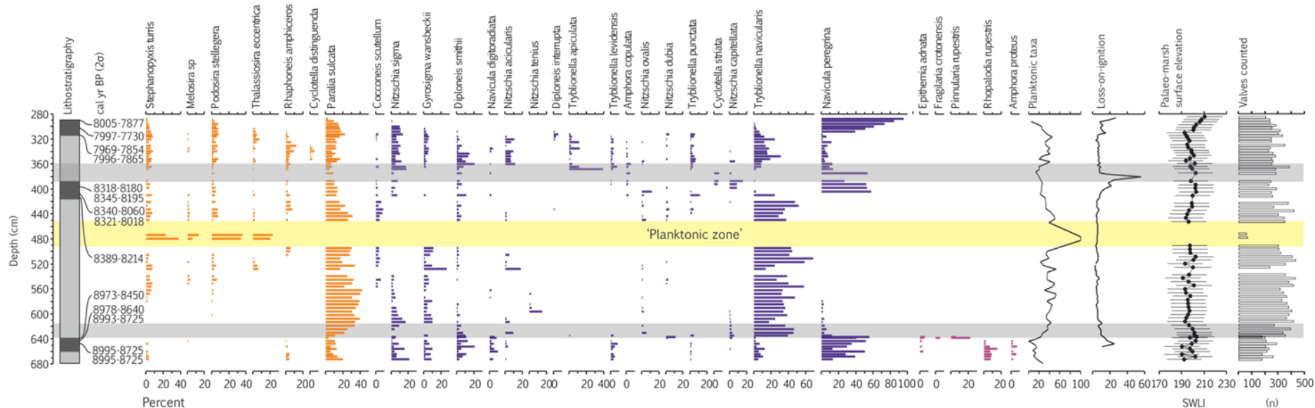
Figure 2.6. Diatom biostratigraphy, chronostratigraphy and LOI of core BC421. Diatom contributions represent >5%. Palaeomarsh surface elevation (in SWLI units) is reconstructed using the component-two model (WA-PLS) of the ‘screened’ training set. For a more detailed view of sample depths of 14 C ages, refer to Figure 2.5 and Table 2.1. Marine taxa (planktonic forms) are indicated in orange, brackish-indifferent taxa in blue and freshwater-brackish taxa in purple. Yellow shading indicates the ‘planktonic zone’ (RSLr 2 ). Grey shading indicates abrupt reductions in SWLI that are accompanied by stratigraphic evidence of marsh drowning (see discussion), with the stratigraphically deepest and shallowest grey shading corresponding to RSLr 1 and RSLr 3 , respectively.
