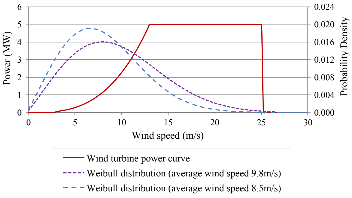
Figure 2.14: The wind turbine power curve against the wind speed and the Weibull wind speed distribution curves.
