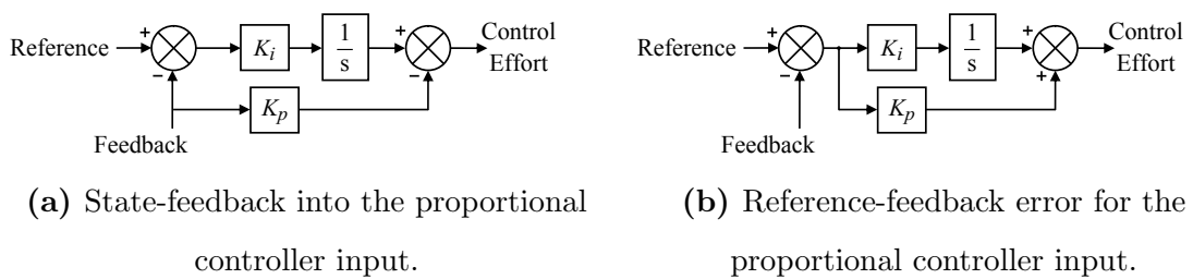
Figure 4.9: Proportional-integral control structures.
