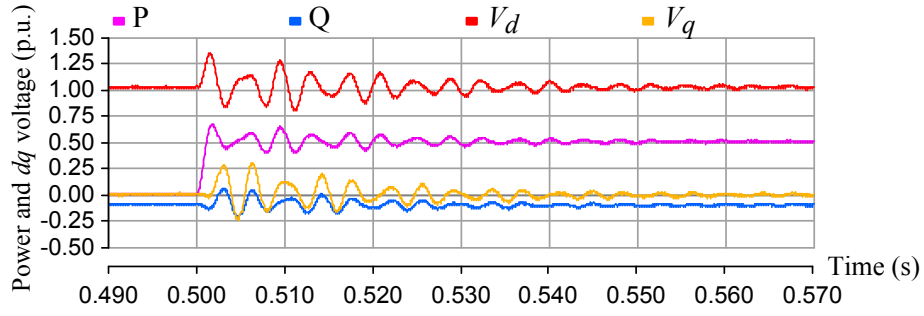
(a) VSC2 is in current control mode and the current loop control bandwidth is equal to the resonant frequency \omega_{ni2} = \omega_0 .
