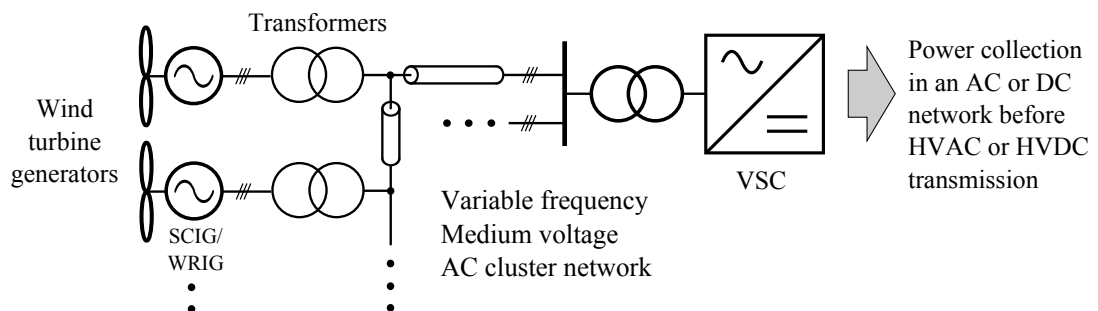
Figure 3.7: A variable frequency network topology.
