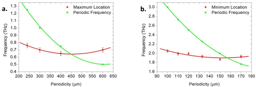
Figure 5.14: Frequency of peak transmission and periodic spacing of; a. 200 \times 40 \mu\text{m} and b. 75 \times 15 \mu\text{m} aperture arrays at various periodic square lattice spacings.
