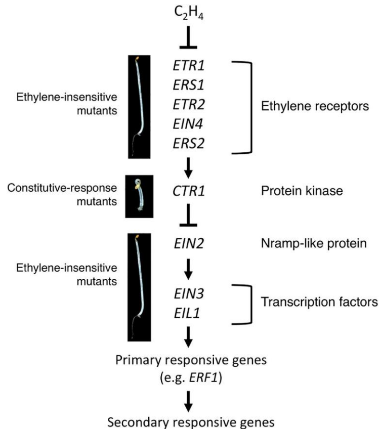
Figure 2. The core ethylene signalling pathway, taken from (Ju and Chang, 2015).
